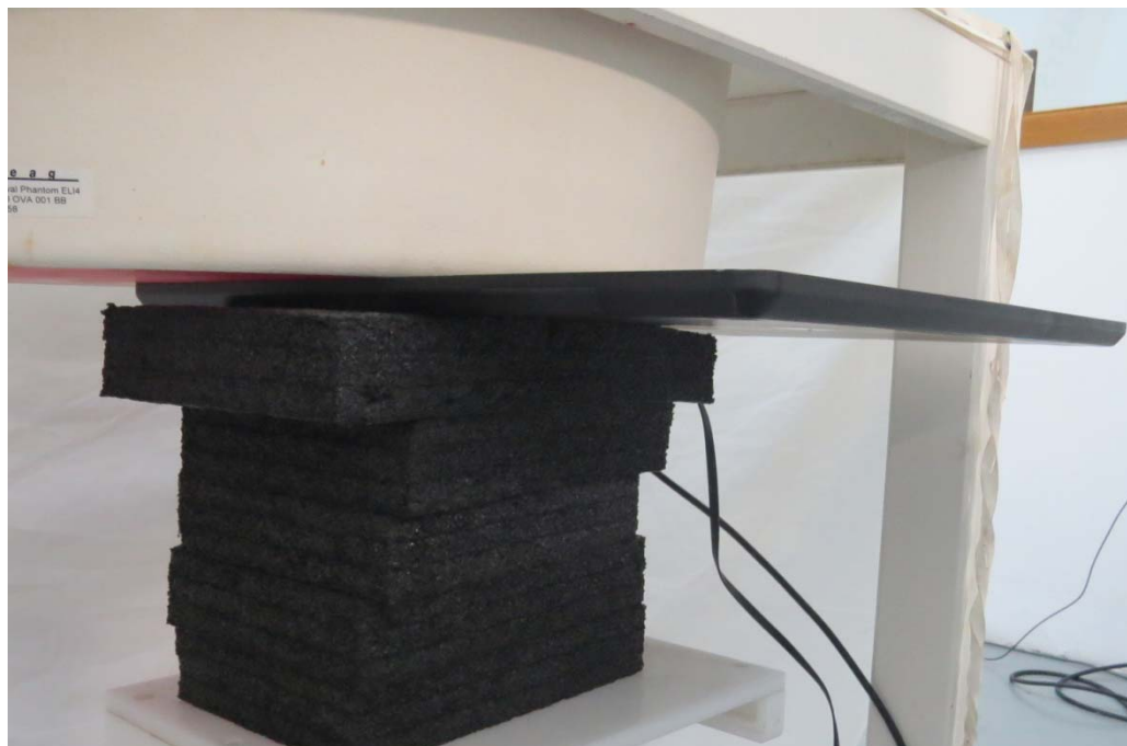
Picture 2: Front Side (Scan 2), the distance from EUT to the bottom of the Phantom is 0mm
