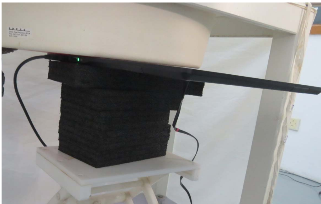
Picture 3: Front Side (Scan 3), the distance from EUT to the bottom of the Phantom is 0mm
