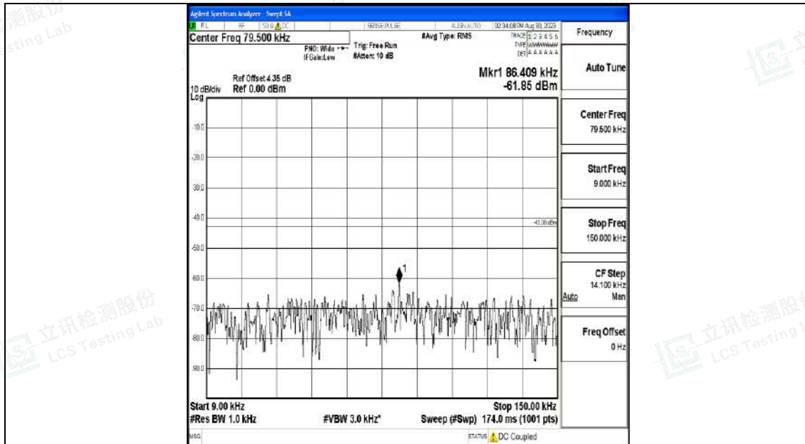
Band25_3MHz_QPSK_26055_1RB#0_0.009~0.15_0.009~0.15
