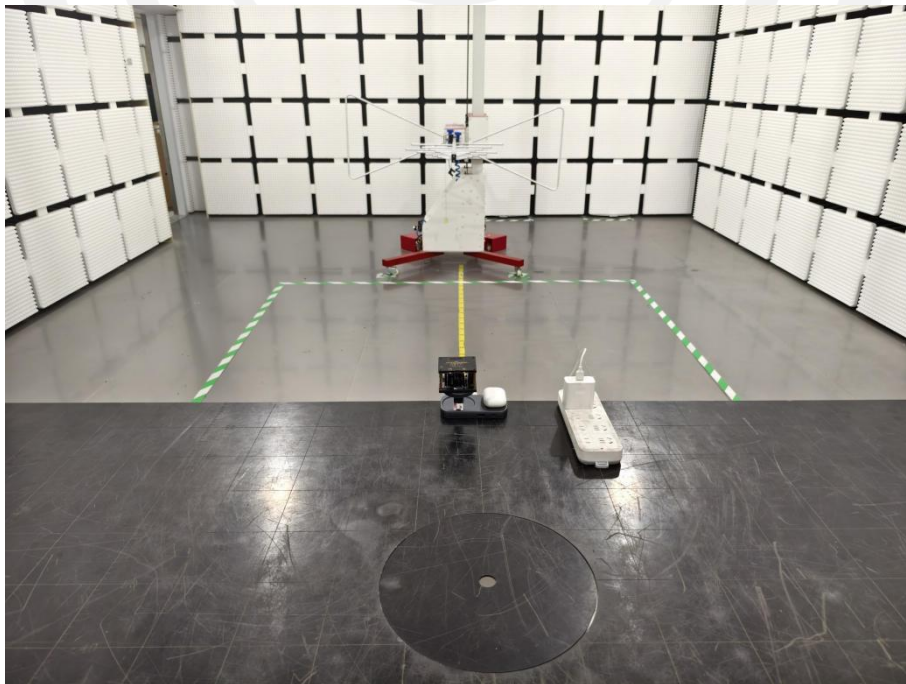
Spurious Radiation Emissions Test (30MHz-1GHz)
