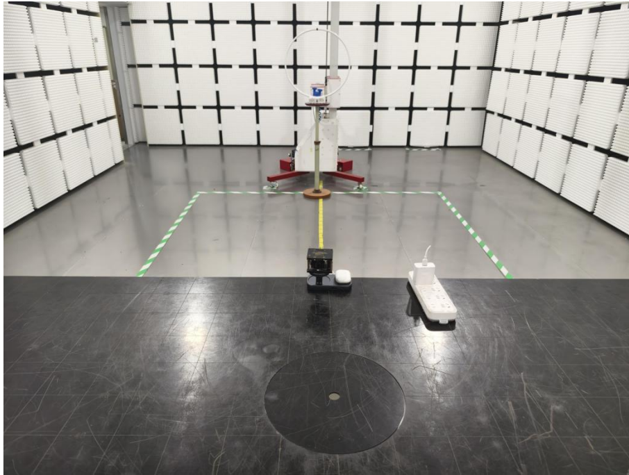
Spurious Radiation Emissions Test (9K-30MHz)
