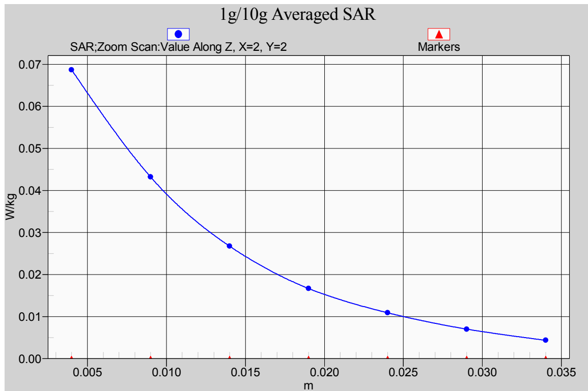
Fig. 38-1 Z-Scan at power reference point (1900MHz CH9400)
