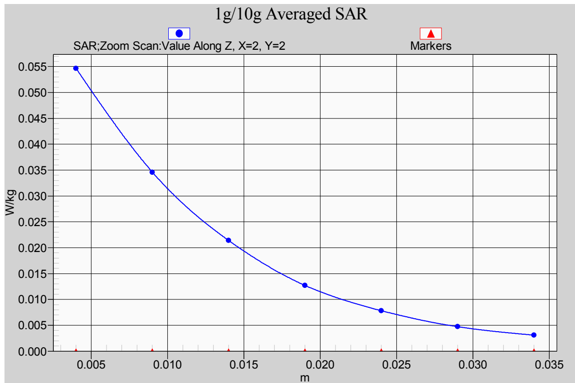
Fig. 20-1 Z-Scan at power reference point (GSM 1900MHz CH512)
