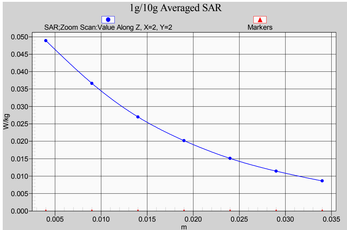
Fig. 9-1 Z-Scan at power reference point (GSM 850MHz CH251)
