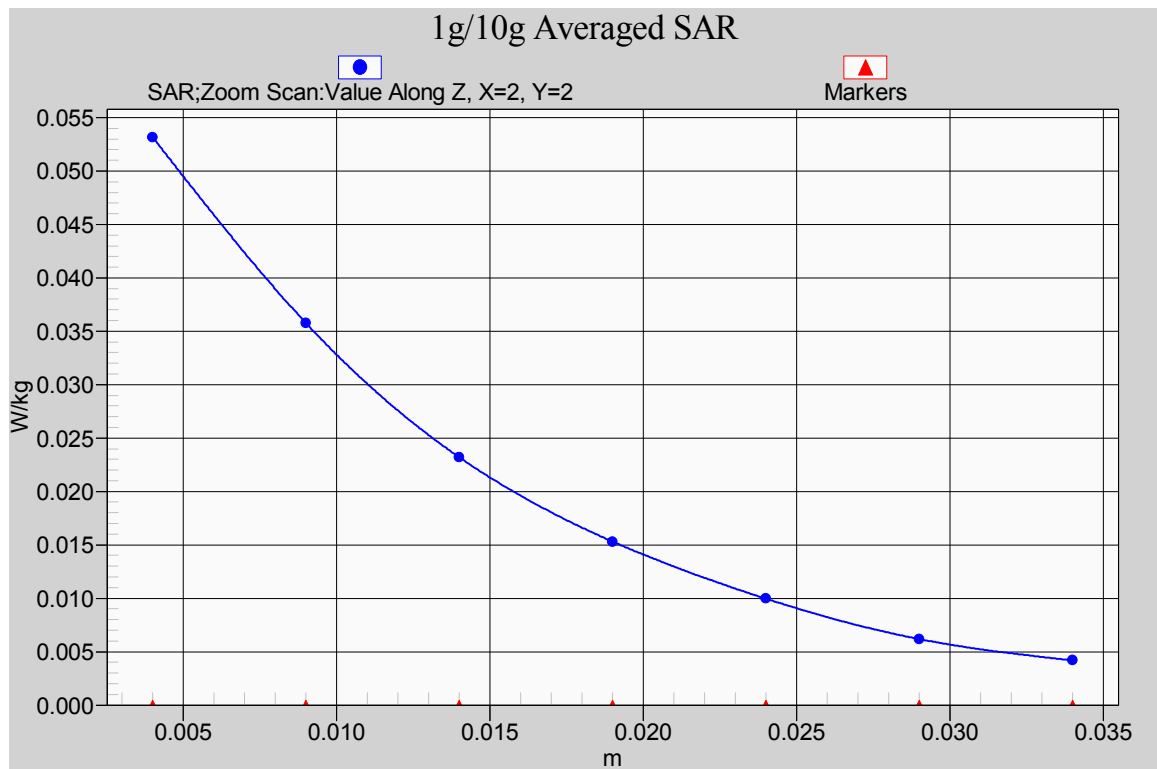
Fig. 36-1 Z-Scan at power reference point (WCDMA 1900MHz CH9262)
