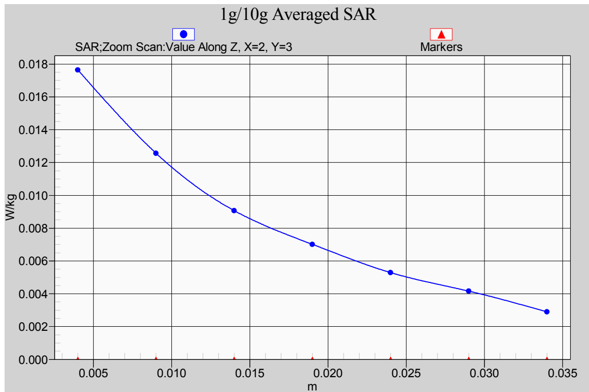
Fig. 25-1 Z-Scan at power reference point (WCDMA 850MHz CH4233)
