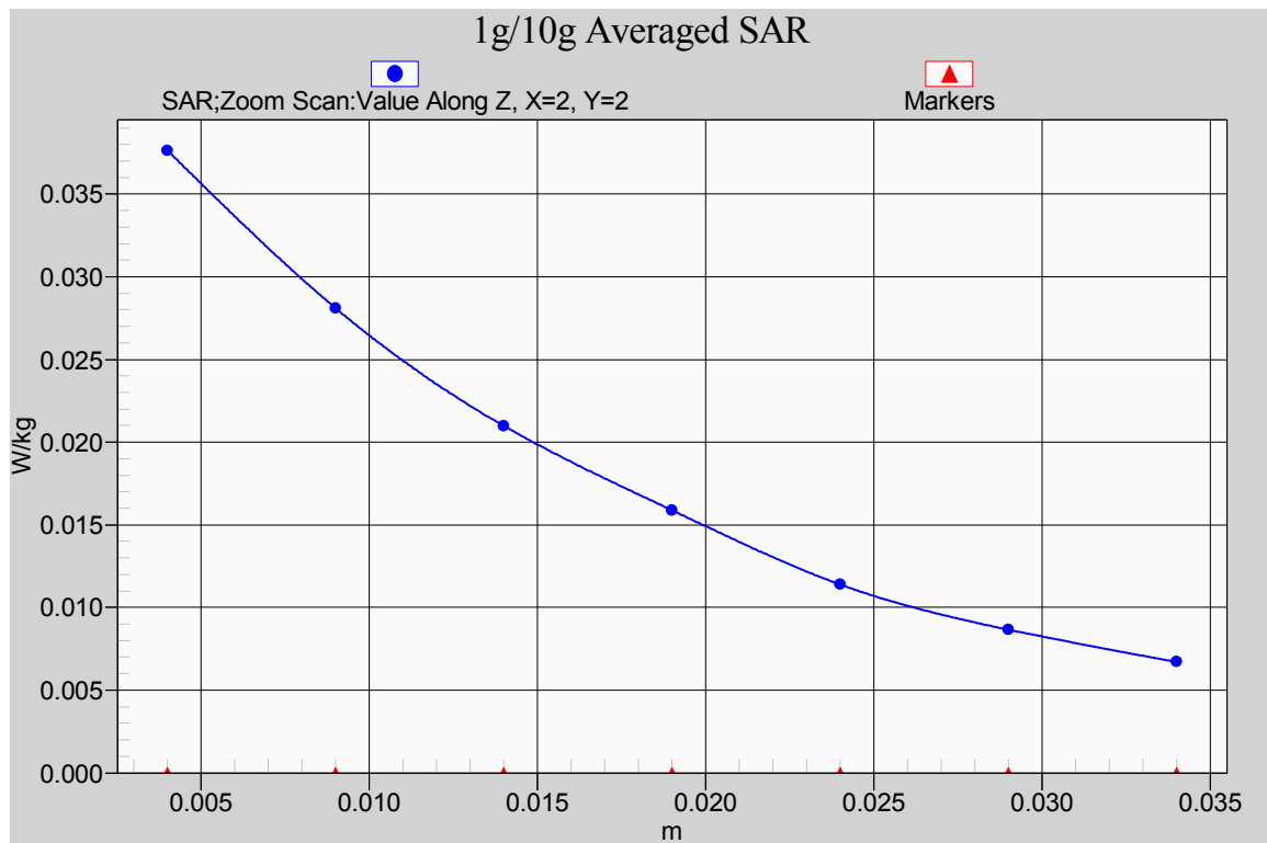
Fig. 30-1 Z-Scan at power reference point (WCDMA 850MHz CH4132)
