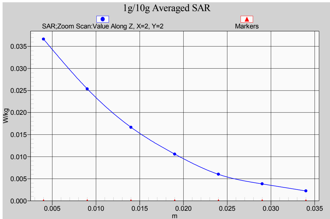
Fig. 16-1 Z-Scan at power reference point (GSM 1900MHz CH512)
