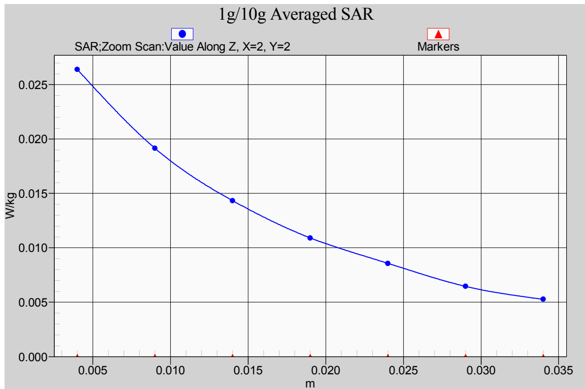
Fig. 5-1 Z-Scan at power reference point (GSM 850MHz CH251)
