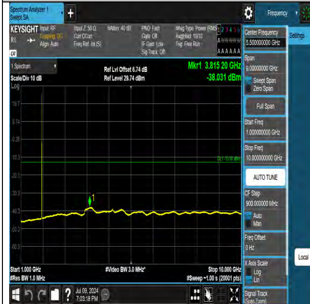
Band25_3MHz_QPSK_26055_1RB#0_1000~10000_1000~10000
