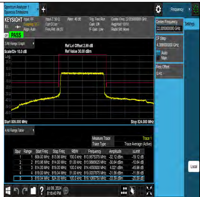
Band26 5MHz 16QAM 26715 25RB#0
