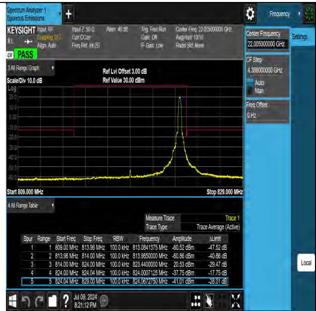
Band26 10MHz QPSK 26740 1RB#49
