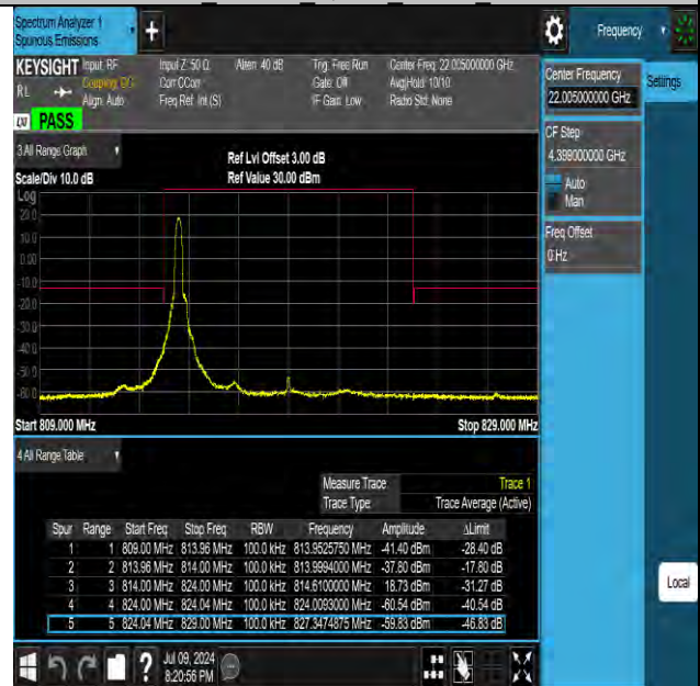
Band26 10MHz 16QAM 26740 1RB#0
