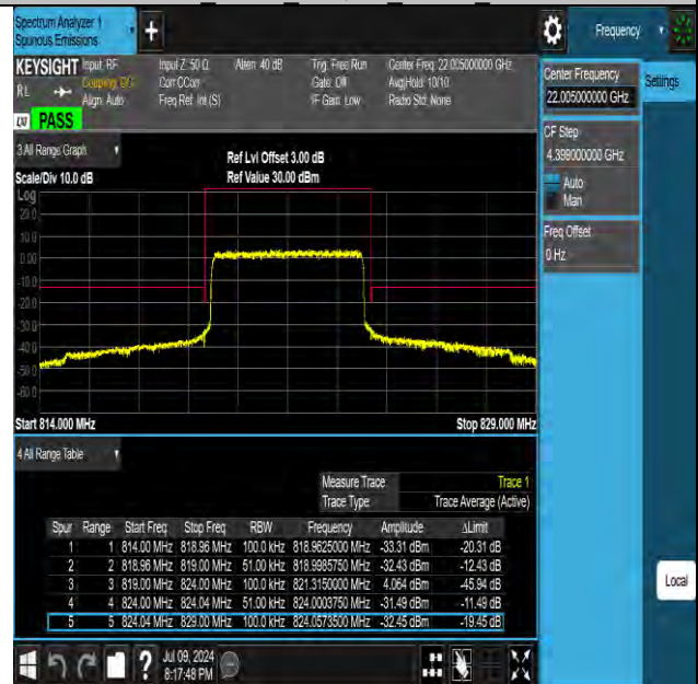
Band26 5MHz 16QAM 26765 25RB#0
