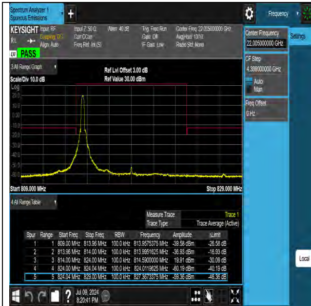
Band26 10MHz QPSK 26740 1RB#0
