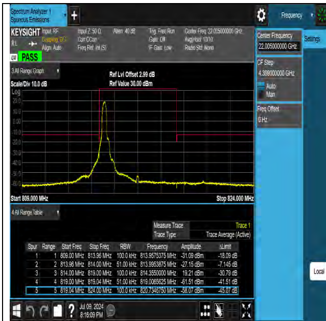
Band26 5MHz 16QAM 26715 1RB#0
