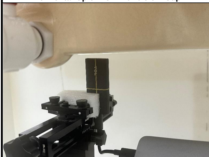
Vertical-Top of EUT with 0.5 cm Gap
