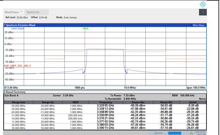
Band48-20MHz-16QAM-3625-1RB#99-PASS
