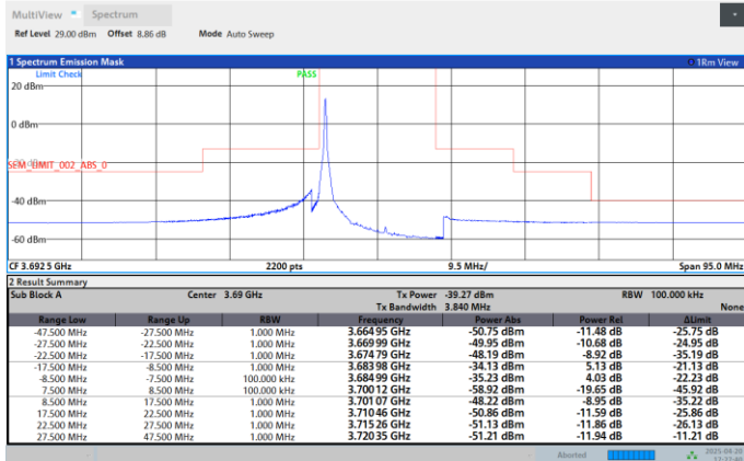
Band48-15MHz-QPSK-3692.5-75RB#0-PASS
