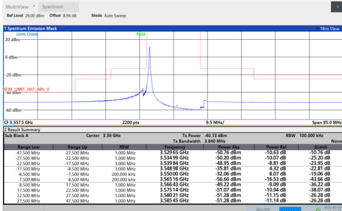
Band48-15MHz-64QAM-3557.5-75RB#0-PASS
