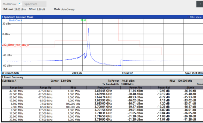
Band48-15MHz-64QAM-3692.5-75RB#0-PASS
