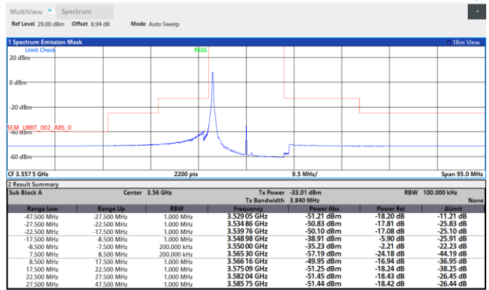
Band48-15MHz-256QAM-3557.5-75RB#0-PASS
