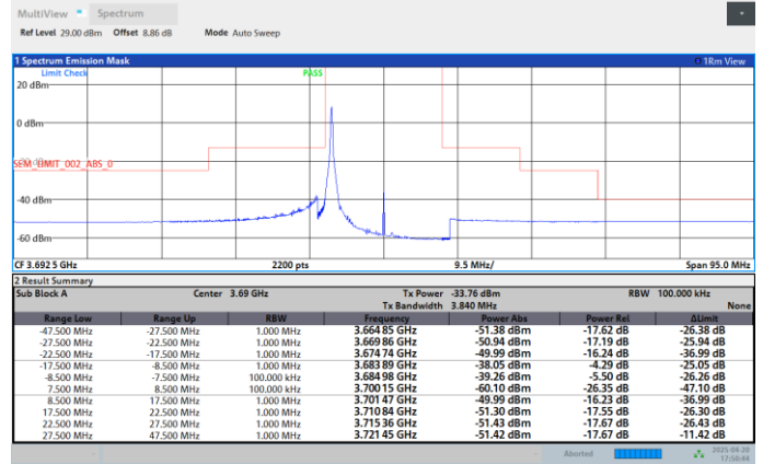
Band48-15MHz-256QAM-3692.5-75RB#0-PASS
