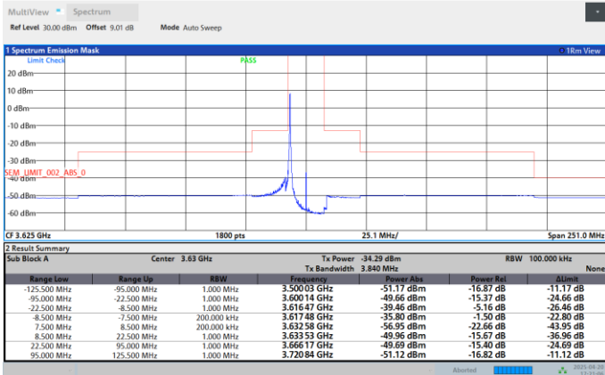
Band48-15MHz-256QAM-3625-75RB#0-PASS
