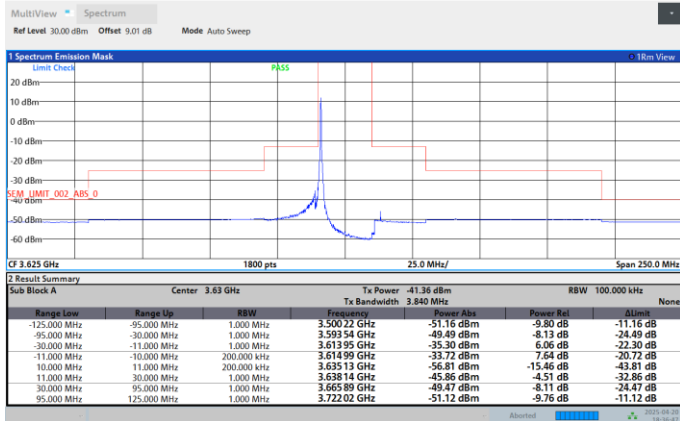
Band48-20MHz-16QAM-3625-100RB#0-PASS
