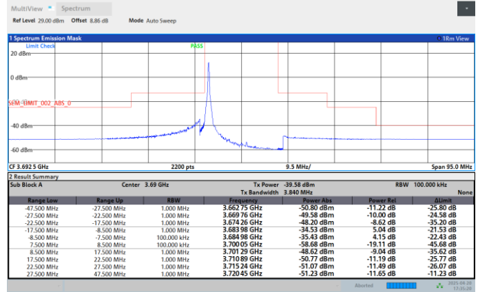
Band48-15MHz-16QAM-3692.5-75RB#0-PASS
