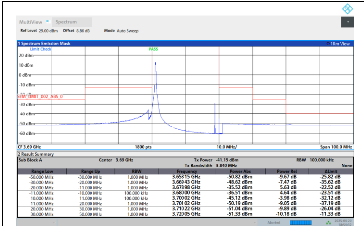
Band48-20MHz-QPSK-3690-100RB#0-PASS
