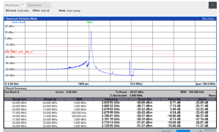
Band48-20MHz-16QAM-3690-100RB#0-PASS
