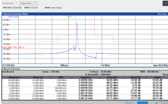
Band48-10MHz-QPSK-3555-50RB#0-PASS
