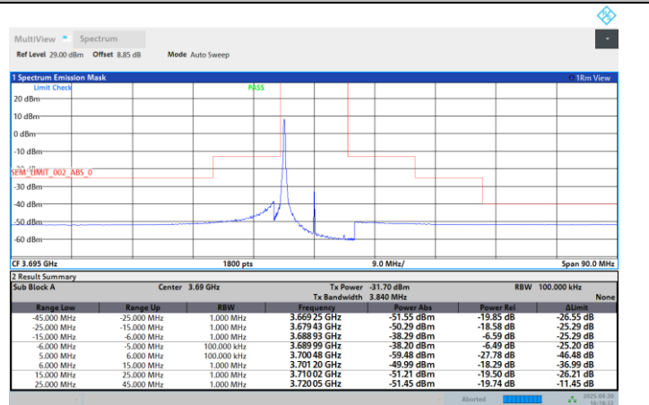
Band48-10MHz-256QAM-3695-50RB#0-PASS
