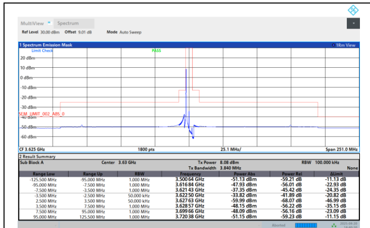
Band48-5MHz-256QAM-3625-25RB#0-PASS
