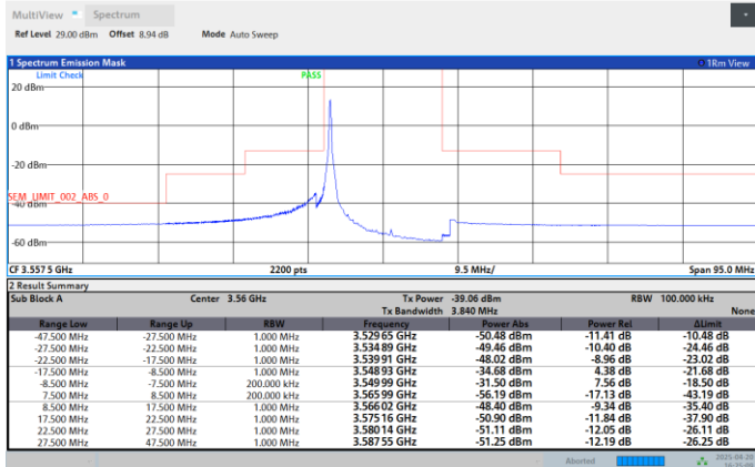
Band48-15MHz-QPSK-3557.5-75RB#0-PASS
