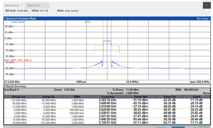
Band48-10MHz-QPSK-3695-1RB#49-PASS
