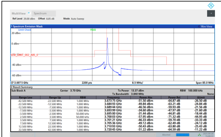
Band48-5MHz-64QAM-3697.5-25RB#0-PASS
