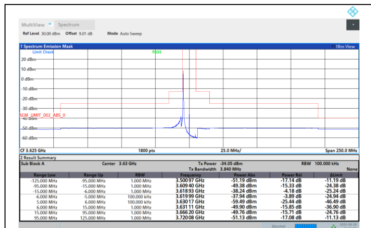
Band48-10MHz-256QAM-3625-50RB#0-PASS
