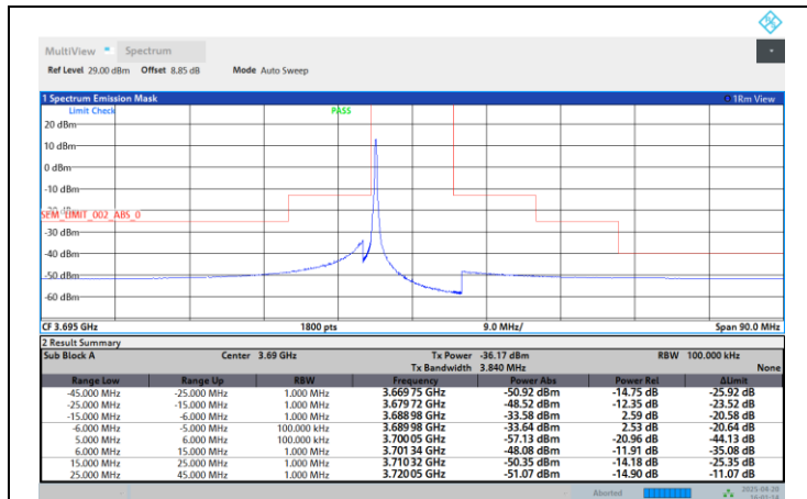
Band48-10MHz-QPSK-3695-50RB#0-PASS
