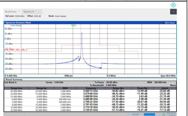
Band48-10MHz-16QAM-3695-50RB#0-PASS
