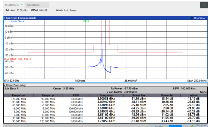
Band48-10MHz-64QAM-3625-50RB#0-PASS
