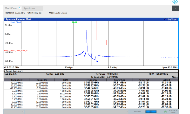
Band48-5MHz-256QAM-3552.5-25RB#0-PASS
