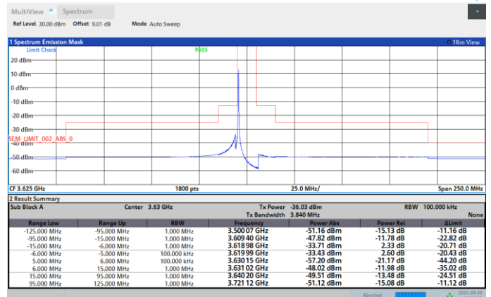
Band48-10MHz-QPSK-3625-50RB#0-PASS
