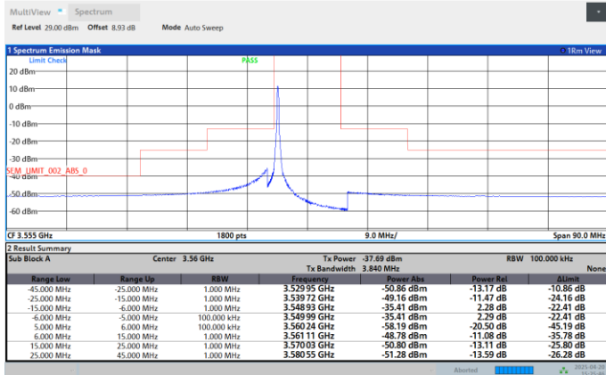
Band48-10MHz-64QAM-3555-50RB#0-PASS
