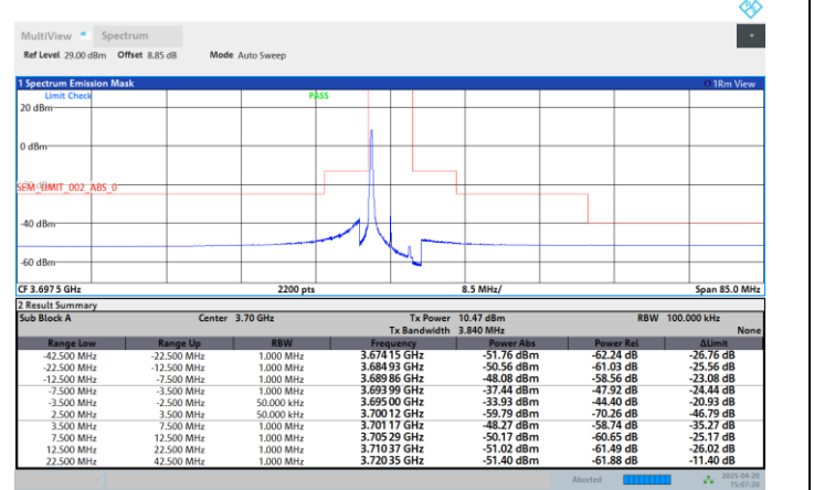
Band48-5MHz-256QAM-3697.5-25RB#0-PASS
