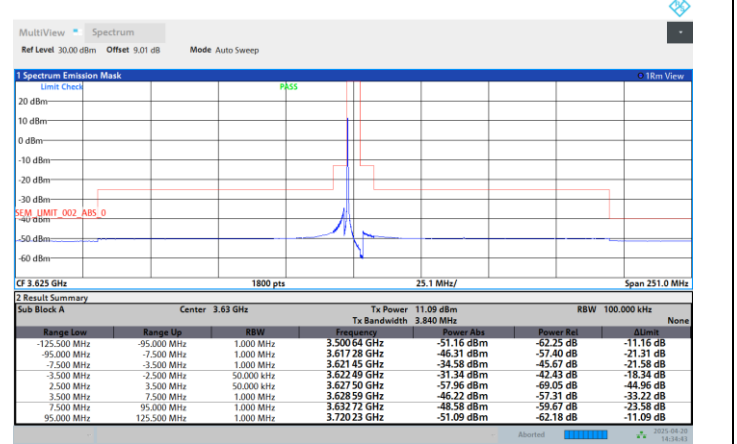
Band48-5MHz-64QAM-3625-25RB#0-PASS
