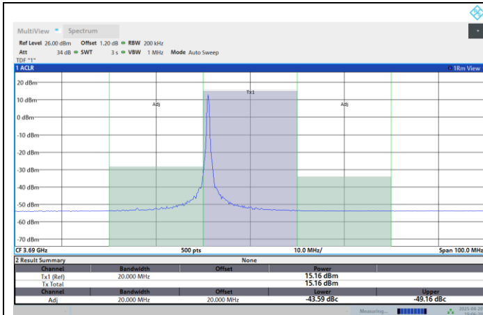
Band48-20MHz-64QAM-3690-100RB#0-PASS
