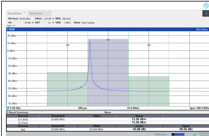
Band48-20MHz-64QAM-3560-100RB#0-PASS
