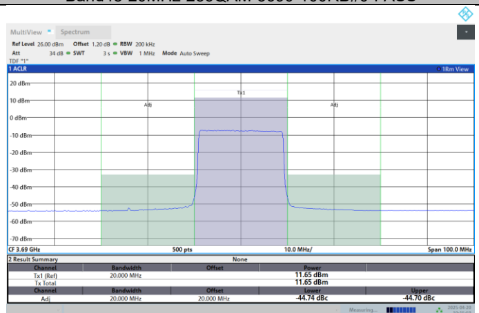
Band48-20MHz-256QAM-3690-100RB#0-PASS
