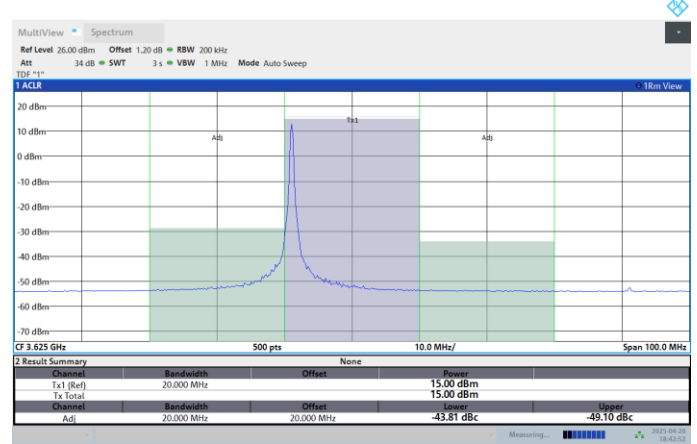
Band48-20MHz-64QAM-3625-100RB#0-PASS
