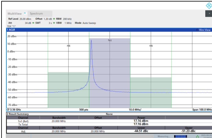
Band48-20MHz-QPSK-3560-100RB#0-PASS
