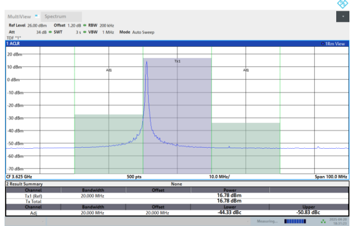
Band48-20MHz-QPSK-3625-100RB#0-PASS
