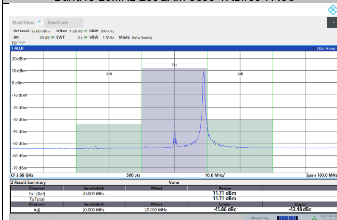
Band48-20MHz-256QAM-3690-1RB#99-PASS
