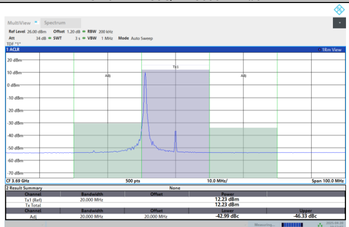
Band48-20MHz-256QAM-3690-100RB#0-PASS
