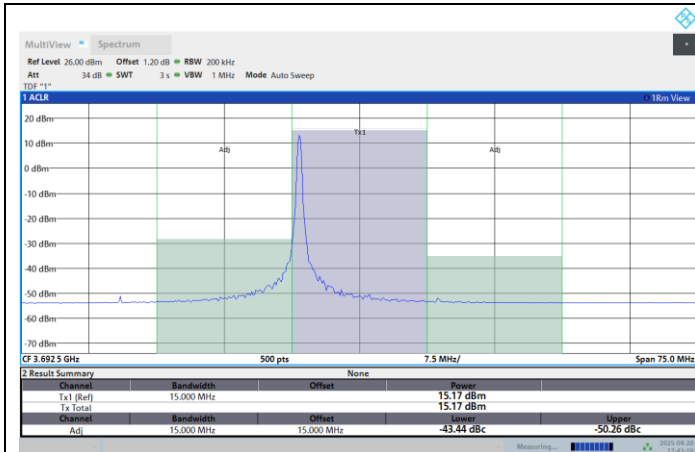
Band48-15MHz-64QAM-3692.5-75RB#0-PASS
