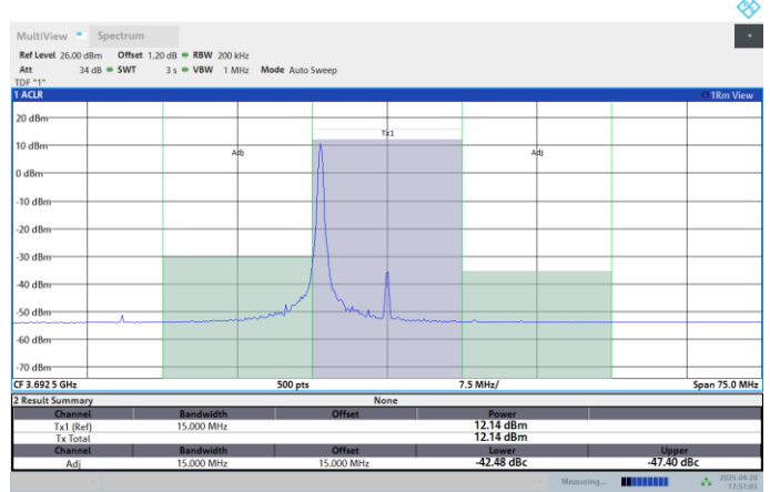
Band48-15MHz-256QAM-3692.5-75RB#0-PASS
