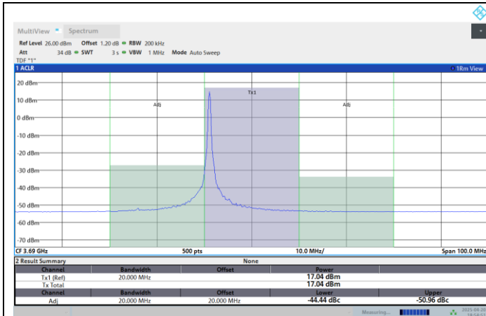
Band48-20MHz-QPSK-3690-100RB#0-PASS
