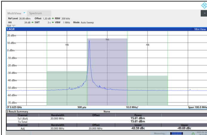
Band48-20MHz-16QAM-3625-100RB#0-PASS
