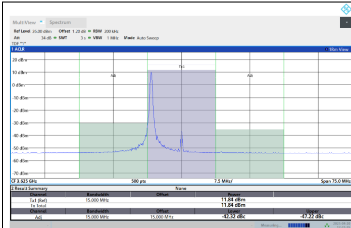
Band48-15MHz-256QAM-3625-75RB#0-PASS
