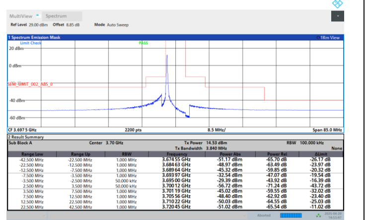
Band48-5MHz-16QAM-3697.5-25RB#0-PASS
