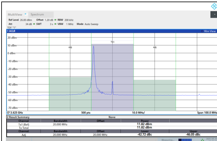
Band48-20MHz-256QAM-3625-100RB#0-PASS
