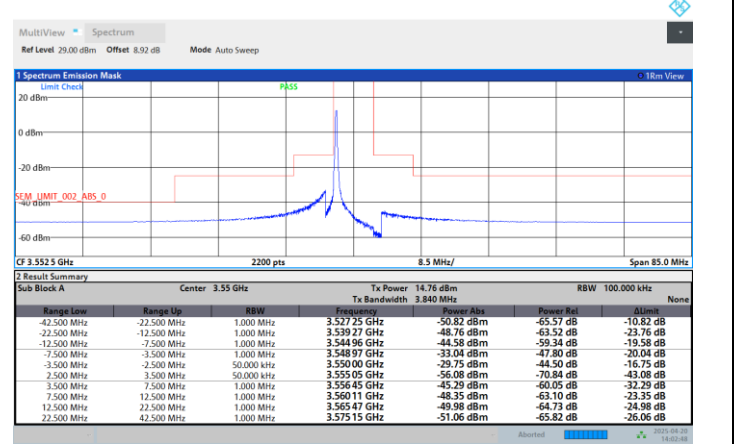
Band48-5MHz-16QAM-3552.5-25RB#0-PASS
