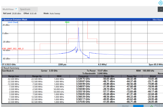
Band48-5MHz-QPSK-3552.5-25RB#0-PASS
