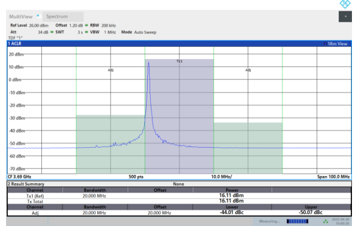
Band48-20MHz-16QAM-3690-100RB#0-PASS
