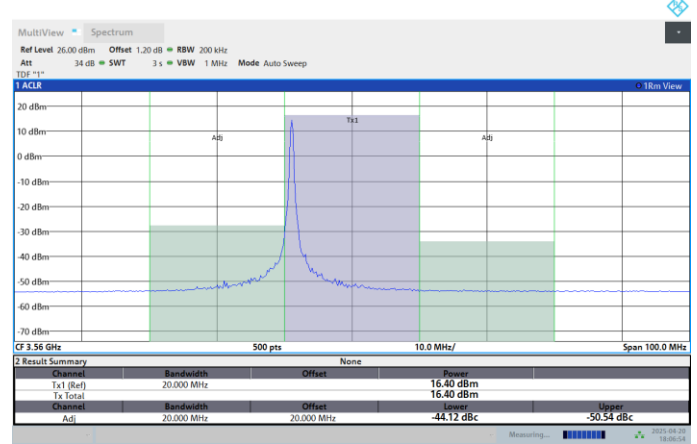
Band48-20MHz-16QAM-3560-100RB#0-PASS
