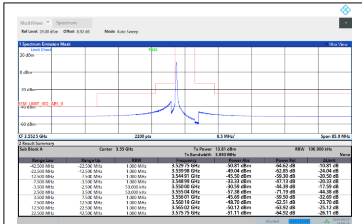
Band48-5MHz-64QAM-3552.5-25RB#0-PASS
