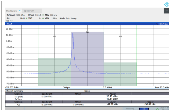
Band48-15MHz-64QAM-3557.5-75RB#0-PASS
