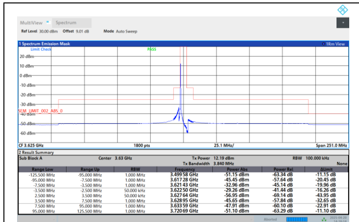
Band48-5MHz-16QAM-3625-25RB#0-PASS
