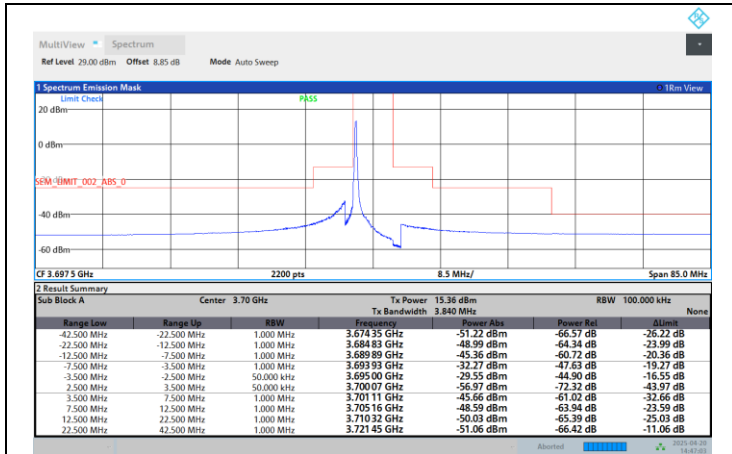
Band48-5MHz-QPSK-3697.5-25RB#0-PASS
