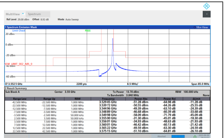
Band48-5MHz-64QAM-3625-1RB#0-PASS
