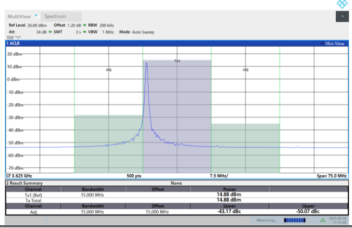
Band48-15MHz-64QAM-3625-75RB#0-PASS
