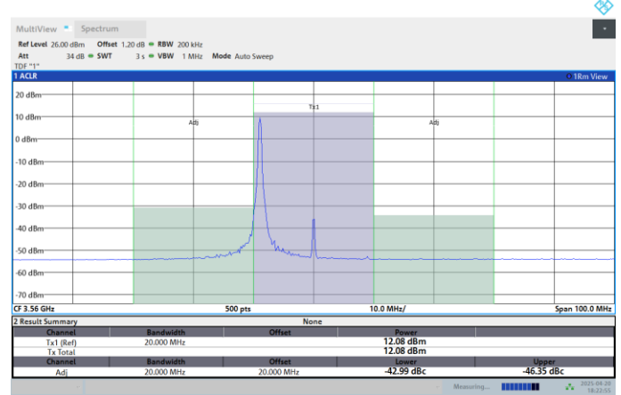
Band48-20MHz-256QAM-3560-100RB#0-PASS
