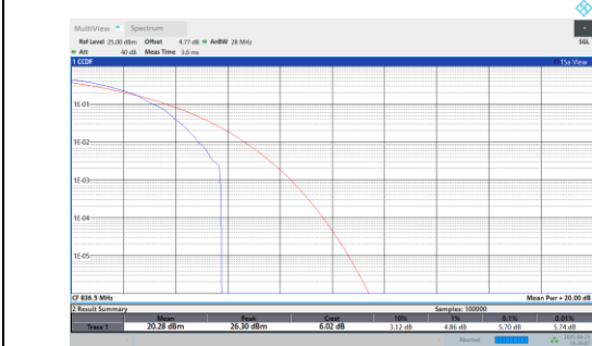
Band 26-5M-MID-1 RB low
