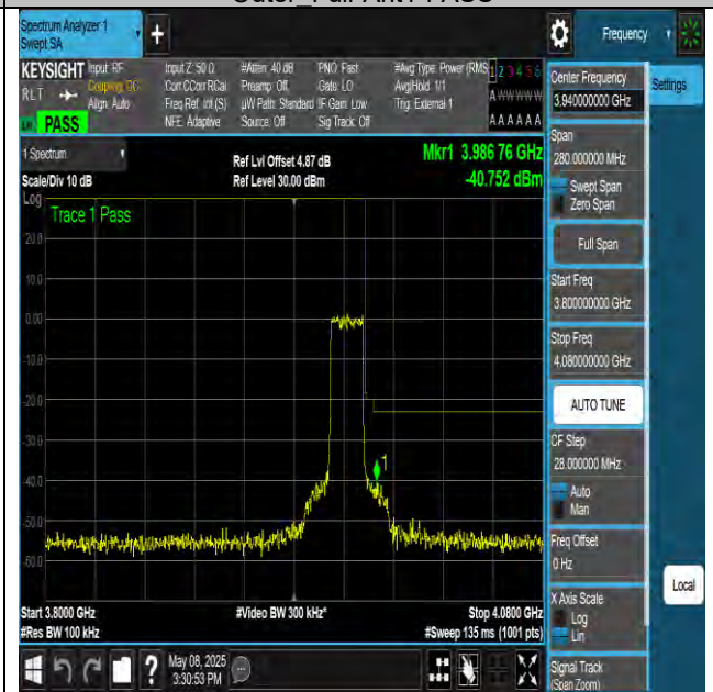
NTNV-N77-3700-3980-PC3-30-20-H-DFT-QPSK- Outer Full-Ant1-PASS
