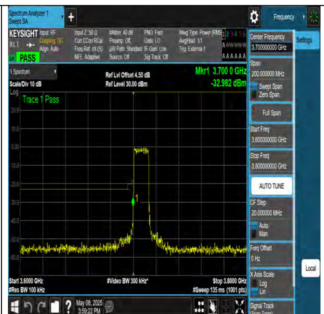
NTNV-N77-3700-3980-PC3-30-15-L-DFT-QPSK- Outer Full-Ant1-PASS
