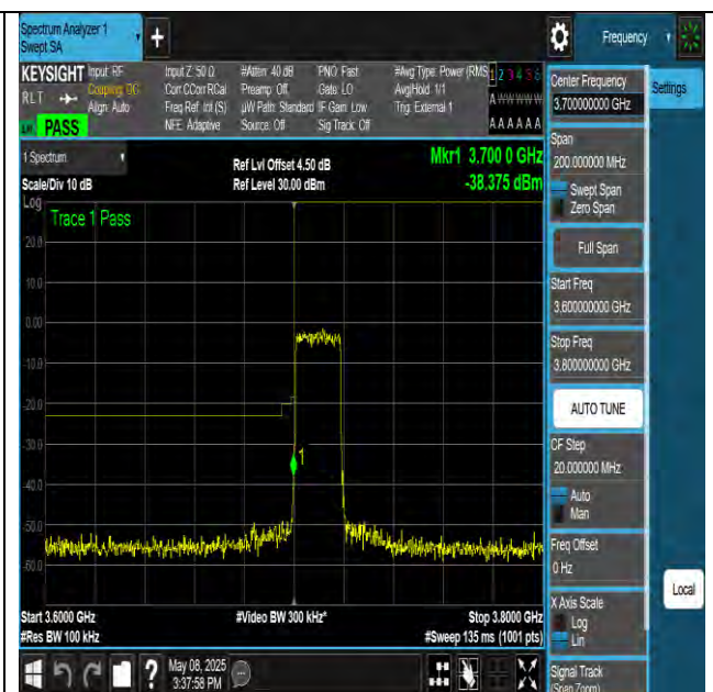
NTNV-N77-3700-3980-PC3-30-20-L-DFT-QPSK- Outer Full-Ant1-PASS
