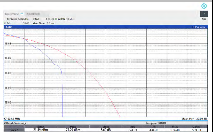
NTNV-N71-PC3-15-10-H-DFT-PI2BPSK-Edge_1RB_Left-PASS
