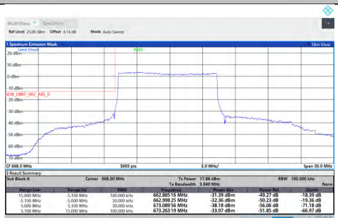
NTNV-N71-PC3-15-10-L-DFT-QPSK-Outer_Full-Ant1-PASS
