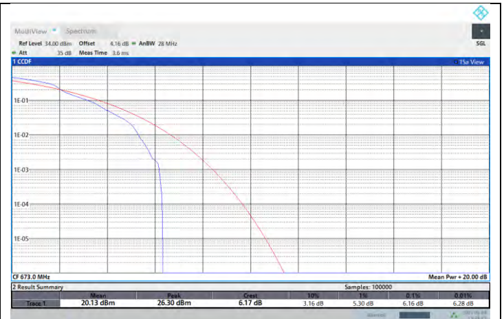
NTNV-N71-PC3-15-20-L-DFT-64QAM-Edge_1RB_Left-PASS
