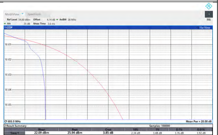
NTNV-N71-PC3-15-10-M-DFT-256QAM-Edge_1RB_Left-PASS
