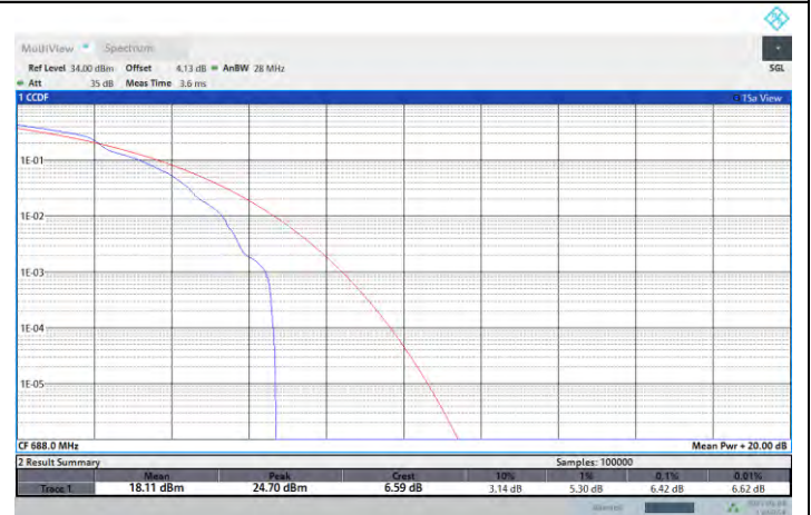
NTNV-N71-PC3-15-20-H-DFT-256QAM-Edge_1RB_Left-PASS
