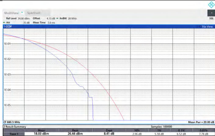
NTNV-N71-PC3-15-10-M-DFT-256QAM-Outer_Full-PASS
