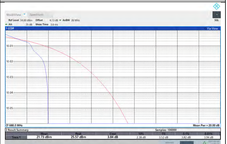
NTNV-N71-PC3-15-20-H-DFT-PI2BPSK-Edge_1RB_Left-PASS
