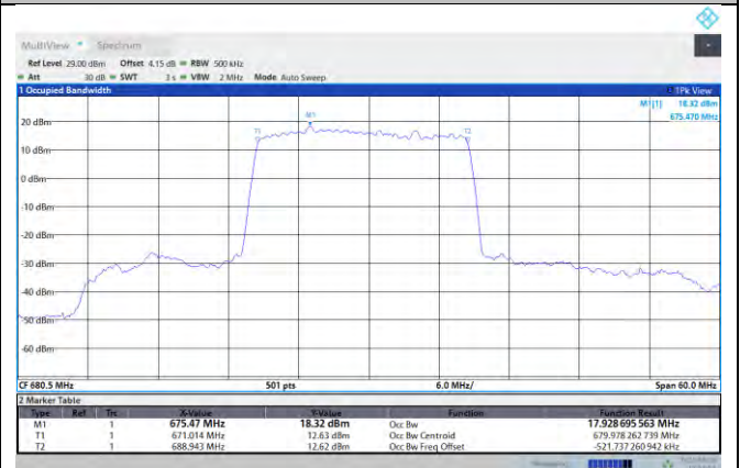
NTNV-N71-PC3-15-20-M-DFT-PI2BPSK-Outer_Full-Ant1-PASS
