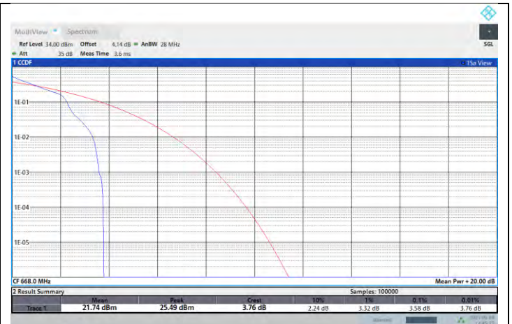
NTNV-N71-PC3-15-10-L-DFT-PI2BPSK-Edge_1RB_Left-PASS
