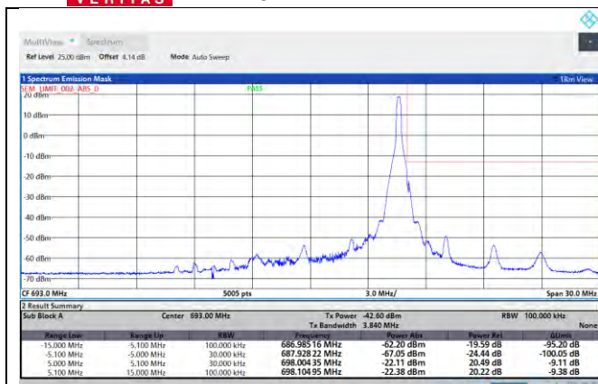
NTNV-N71-PC3-15-10-H-DFT-QPSK-Edge_1RB_Right-Ant1-PASS
