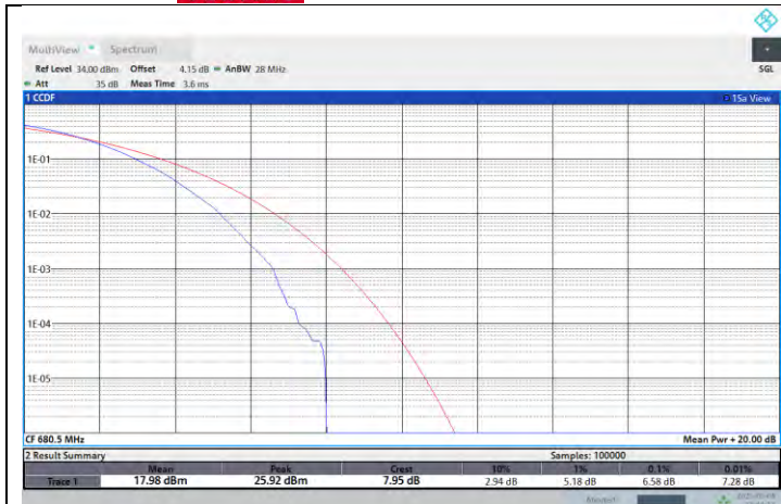
NTNV-N71-PC3-15-20-M-DFT-256QAM-Outer_Full-PASS
