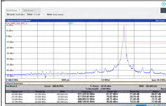
NTNV-N71-PC3-15-20-H-DFT-QPSK-Edge_1RB_Right-Ant1-PASS
