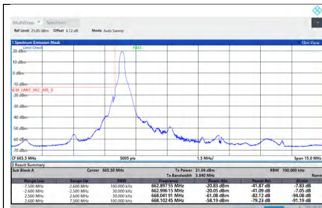
NTNV-N71-PC3-15-5-L-DFT-QPSK-Edge_1RB_Left-Ant1-PASS
