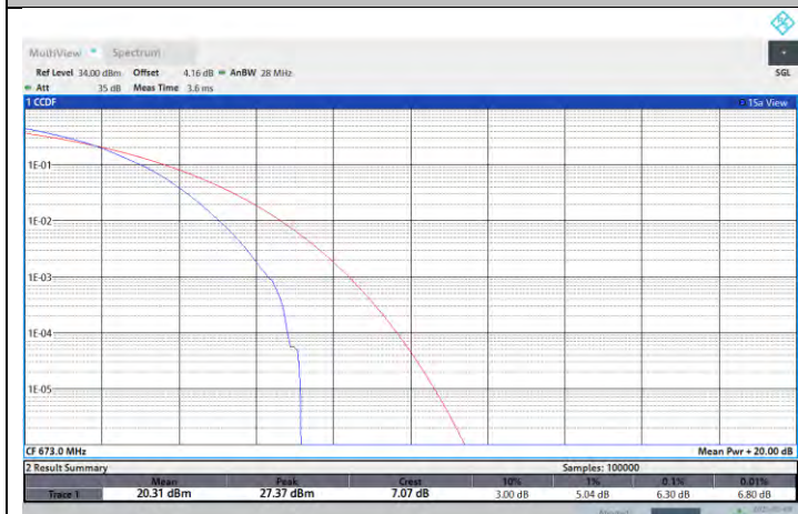
NTNV-N71-PC3-15-20-L-DFT-16QAM-Outer_Full-PASS
