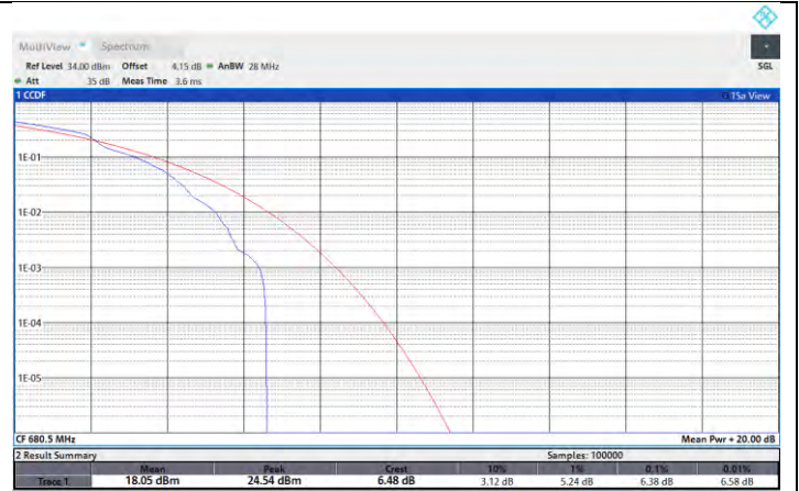
NTNV-N71-PC3-15-10-M-DFT-256QAM-Edge_1RB_Left-PASS
