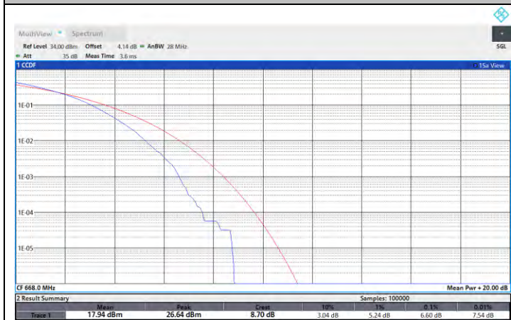
NTNV-N71-PC3-15-10-L-DFT-64QAM-Outer_Full-PASS
