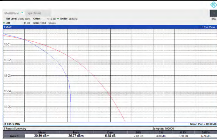
NTNV-N71-PC3-15-5-H-DFT-16QAM-Outer_Full-PASS
