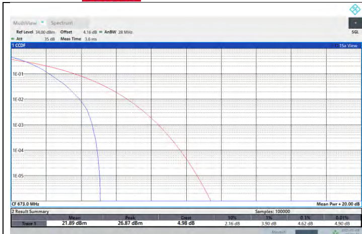
NTNV-N71-PC3-15-20-L-DFT-PI2BPSK-Outer_Full-PASS
