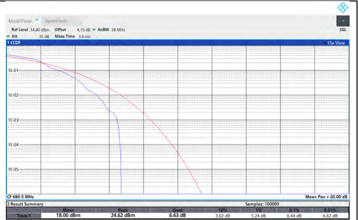
NTNV-N71-PC3-15-15-M-DFT-256QAM-Edge_1RB_Left-PASS
