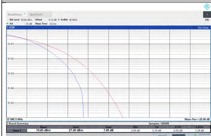
NTNV-N71-PC3-15-10-M-DFT-64QAM-Outer_Full-PASS
