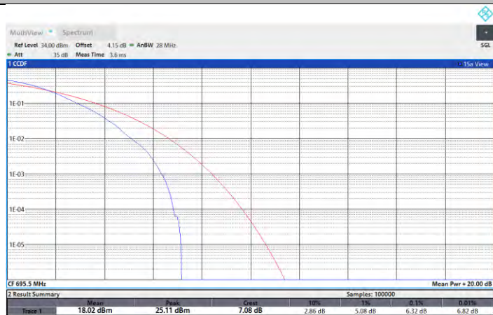
NTNV-N71-PC3-15-5-H-DFT-256QAM-Outer_Full-PASS
