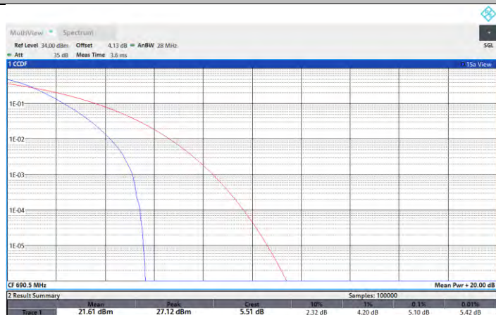
NTNV-N71-PC3-15-15-H-DFT-QPSK-Outer_Full-PASS
