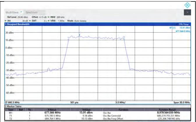
NTNV-N71-PC3-15-10-M-DFT-16QAM-Outet_Full-Ant1-PASS
