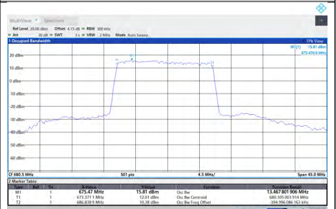
NTNV-N71-PC3-15-15-M-DFT-QPSK-Outet_Full-Ant1-PASS
