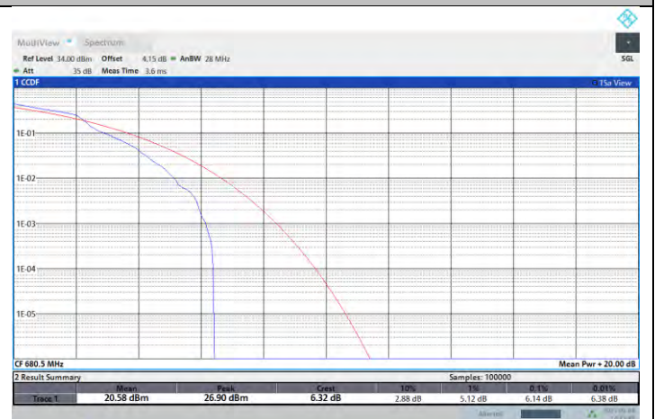
NTNV-N71-PC3-15-5-M-DFT-16QAM-Edge_1RB_Left-PASS
