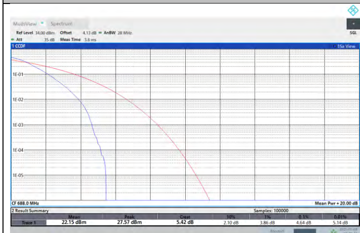
NTNV-N71-PC3-15-20-H-DFT-PI2BPSK-Outer_Full-PASS
