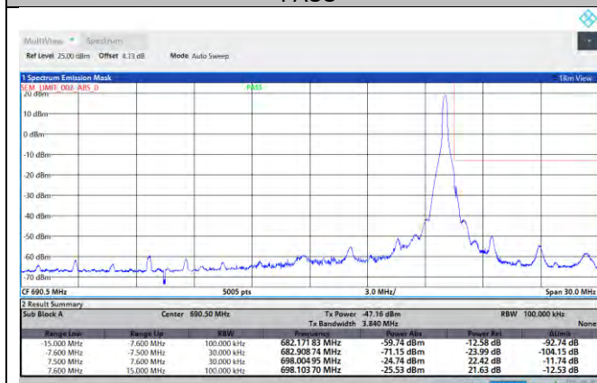
NTNV-N71-PC3-15-15-H-DFT-QPSK-Edge_1RB_Right-Ant1-PASS
