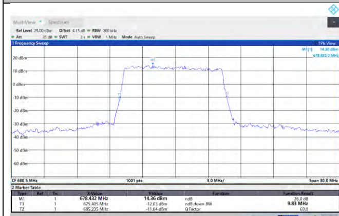
NTN-N71-PC3-15-10-M-DFT-64QAM-Outer_Full-Ant1-PASS
