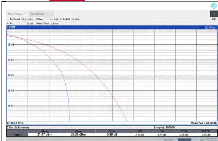
NTNV-N71-PC3-15-15-M-DFT-QPSK-Outer_Full-PASS
