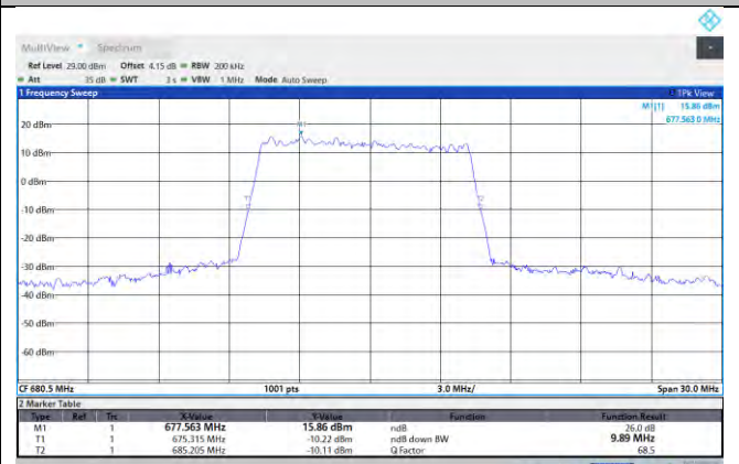
NTN-N71-PC3-15-10-M-DFT-16QAM-Outer_Full-Ant1-PASS
