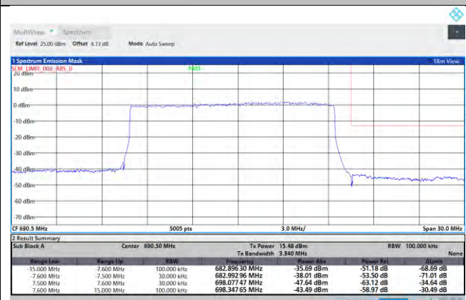
NTNV-N71-PC3-15-15-H-DFT-QPSK-Outer_Full-Ant1-PASS
