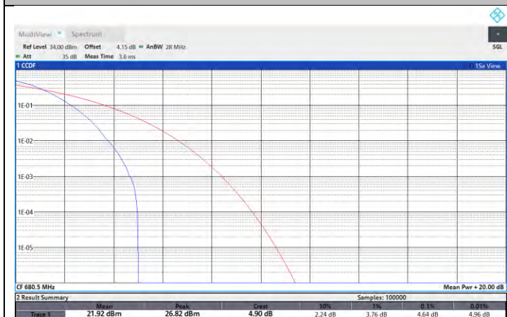
NTNV-N71-PC3-15-10-L-DFT-256QAM-Outer_Full-PASS
