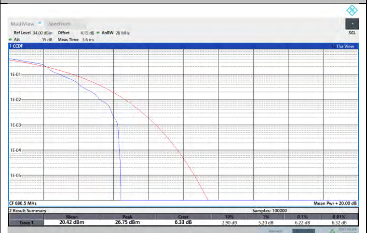
NTNV-N71-PC3-15-15-M-DFT-16QAM-Edge_1RB_Left-PASS
