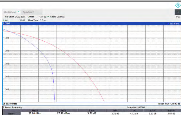
NTNV-N71-PC3-15-10-H-DFT-PI2BPSK-Outer_Full-PASS
