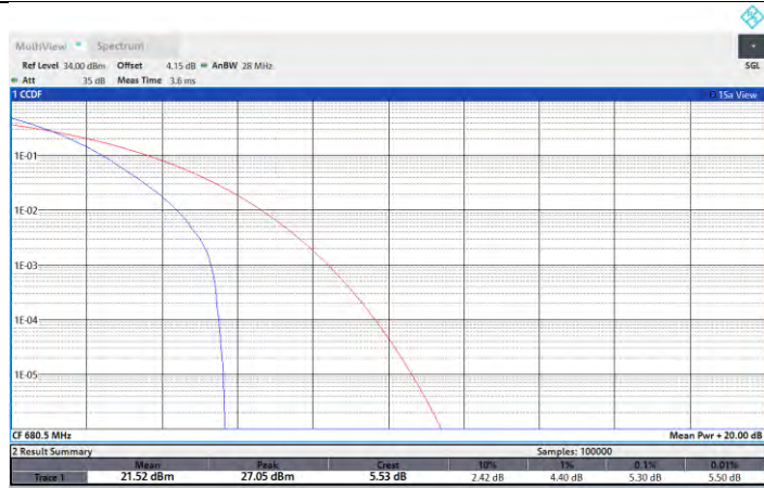
NTNV-N71-PC3-15-5-M-DFT-QPSK-Outer_Full-PASS
