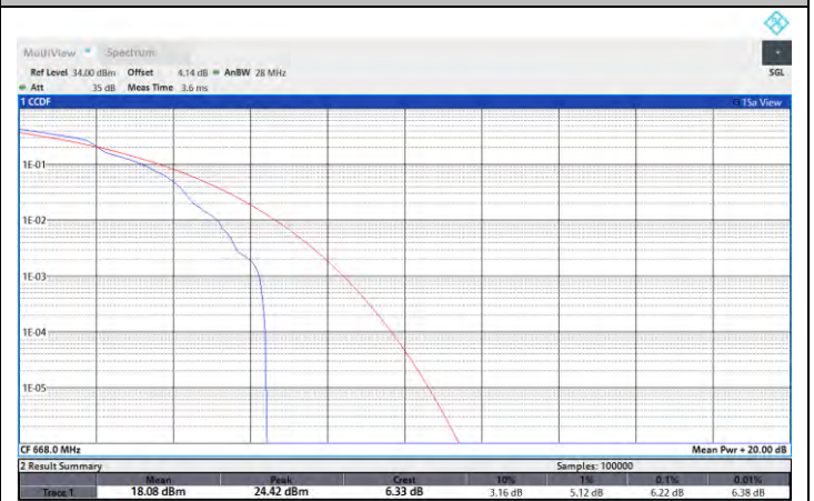
NTNV-N71-PC3-15-10-L-DFT-64QAM-Edge_1RB_Left-PASS
