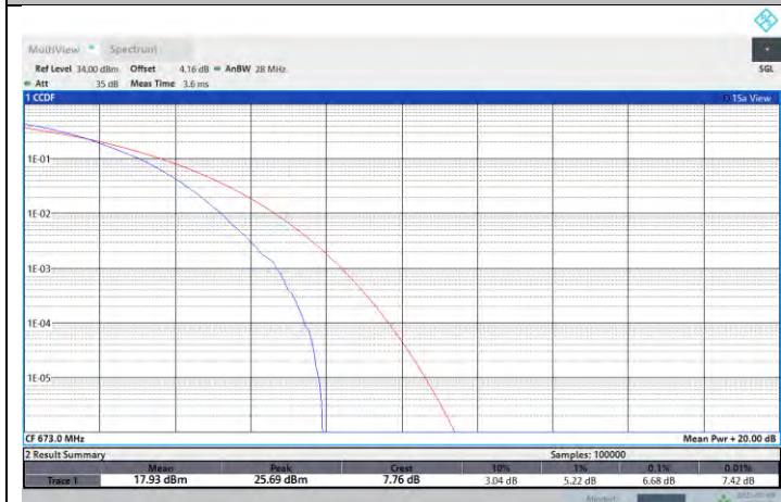
NTNV-N71-PC3-15-20-L-DFT-256QAM-Outer_Full-PASS
