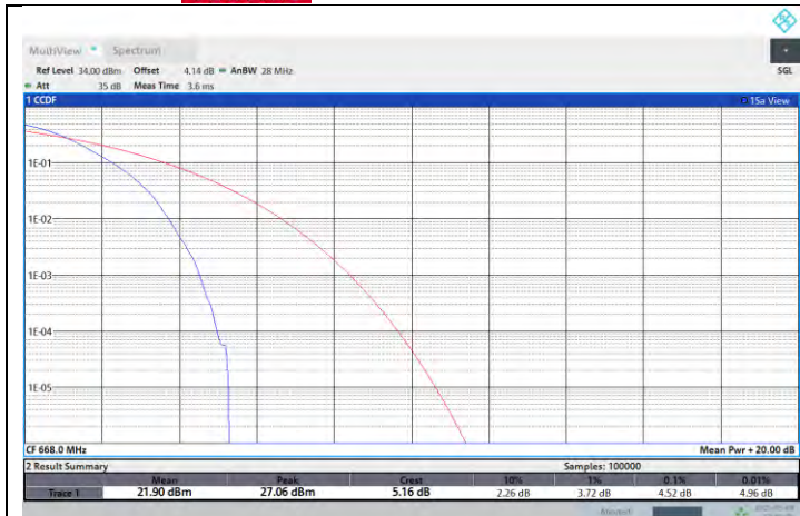
NTNV-N71-PC3-15-10-L-DFT-PI2BPSK-Outer_Full-PASS
