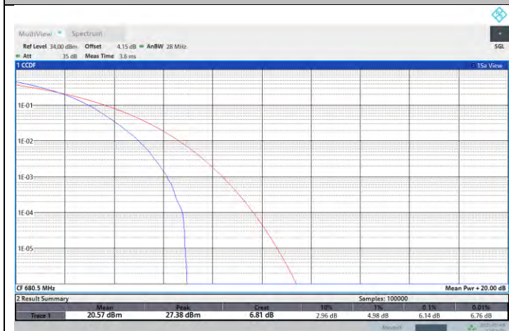
NTNV-N71-PC3-15-10-M-DFT-16QAM-Outer_Full-PASS
