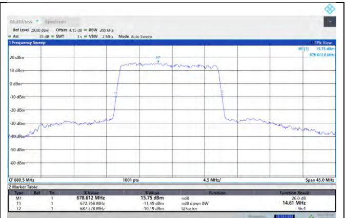
NTNV-N71-PC3-15-15-M-DFT-QPSK-Outter_Full-Ant1-PASS
