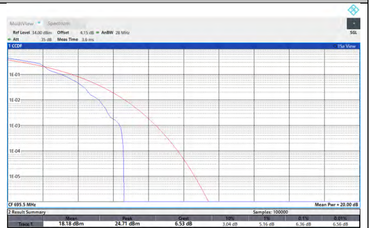
NTNV-N71-PC3-15-5-H-DFT-256QAM-Edge_1RB_Left-PASS
