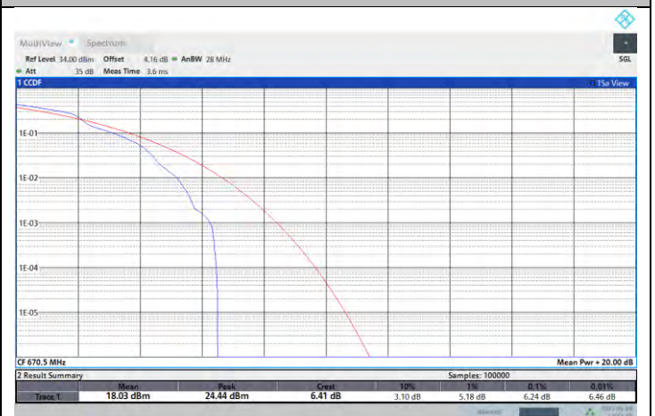
NTNV-N71-PC3-15-15-L-DFT-256QAM-Edge_1RB_Left-PASS
