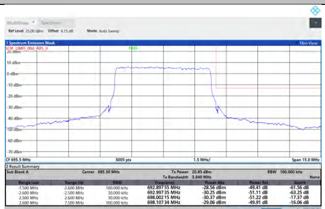
NTNV-N71-PC3-15-5-H-DFT-QPSK-Outer_Full-Ant1-PASS
