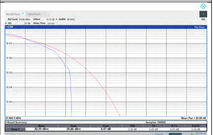
NTNV-N71-PC3-15-15-H-DFT-64QAM-Edge_1RB_Left-PASS
