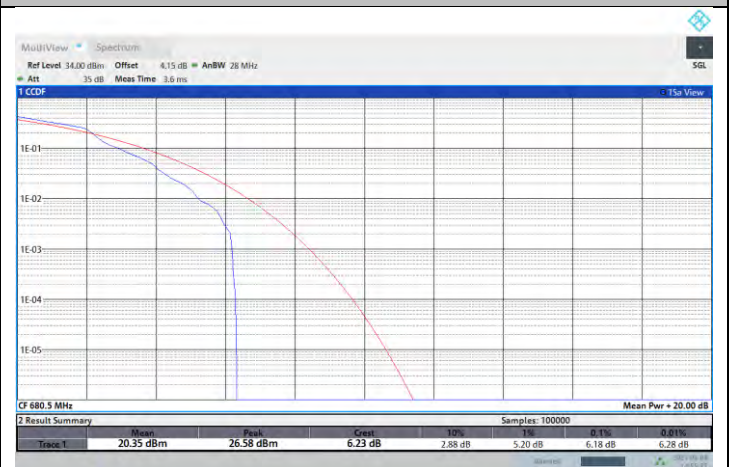
NTNV-N71-PC3-15-10-M-DFT-16QAM-Edge_1RB_Left-PASS
