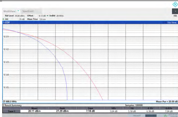
NTNV-N71-PC3-15-20-H-DFT-64QAM-Outer_Full-PASS
