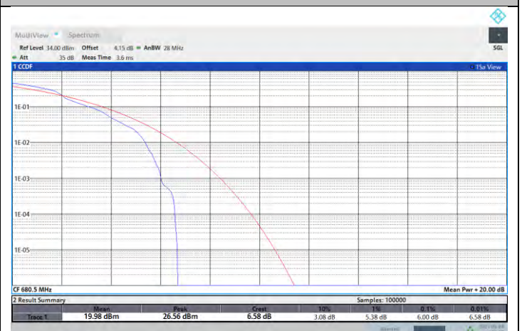
NTNV-N71-PC3-15-10-M-DFT-64QAM-Edge_1RB_Left-PASS
