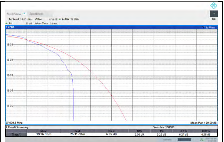
NTNV-N71-PC3-15-15-L-DFT-64QAM-Edge_1RB_Left-PASS
