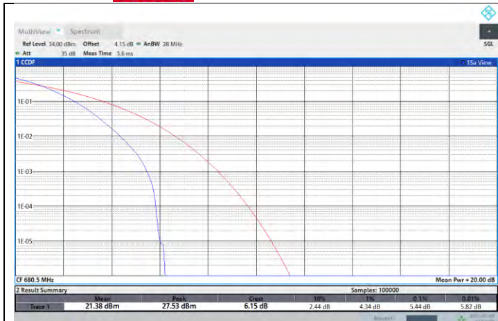
NTNV-N71-PC3-15-10-M-DFT-QPSK-Outer_Full-PASS
