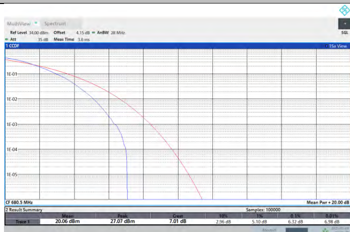
NTNV-N71-PC3-15-5-M-DFT-64QAM-Outer_Full-PASS
