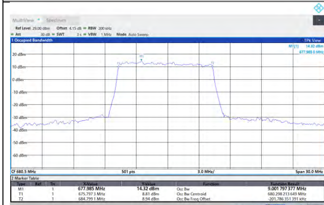
NTNV-N71-PC3-15-10-M-DFT-64QAM-Outet_Full-Ant1-PASS
