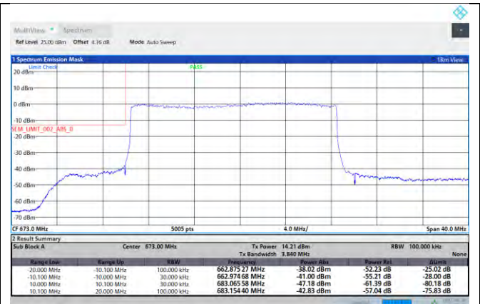
NTNV-N71-PC3-15-20-L-DFT-QPSK-Outer_Full-Ant1-PASS
