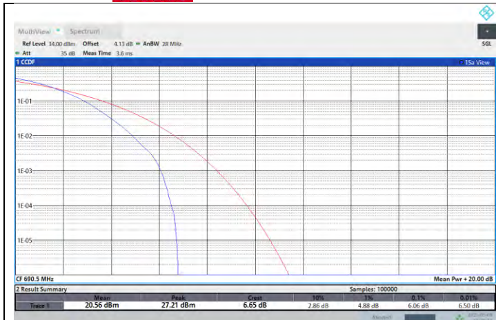
NTNV-N71-PC3-15-15-H-DFT-16QAM-Outer_Full-PASS
