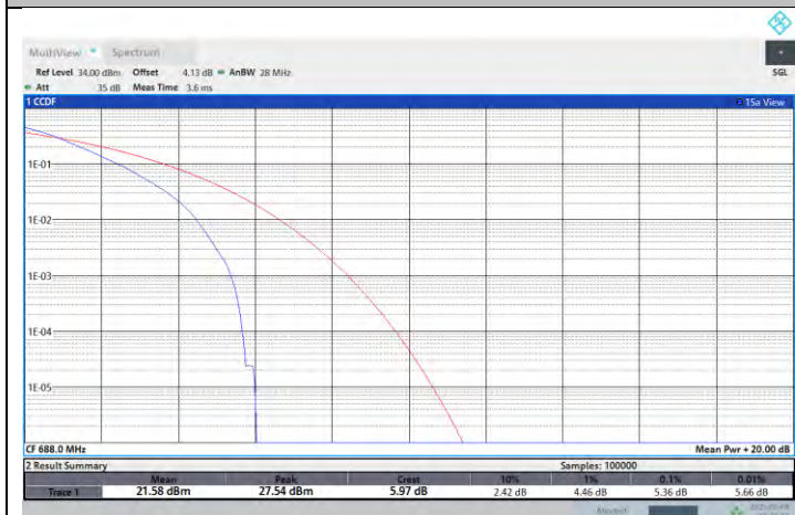
NTNV-N71-PC3-15-20-H-DFT-QPSK-Outer_Full-PASS
