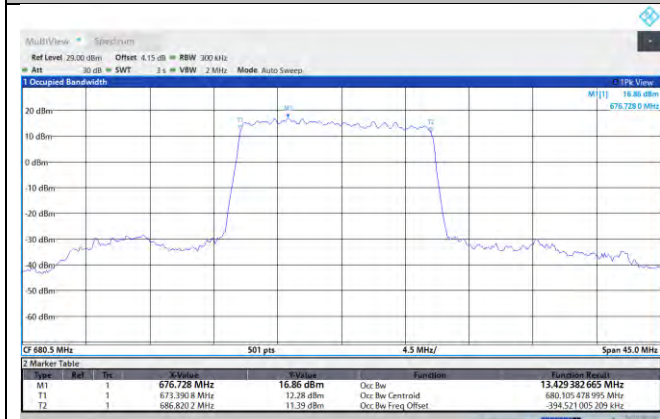
NTNV-N71-PC3-15-15-M-DFT-PI2BPSK-Outet_Full-Ant1-PASS
