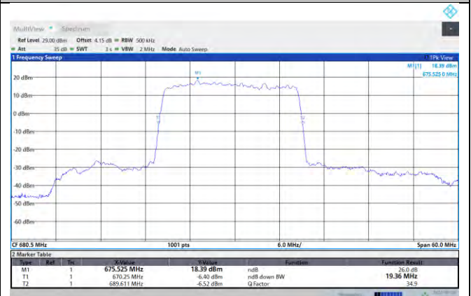
NTNV-N71-PC3-15-20-M-DFT-PI2BPSK-Outter_Full-Ant1-PASS
