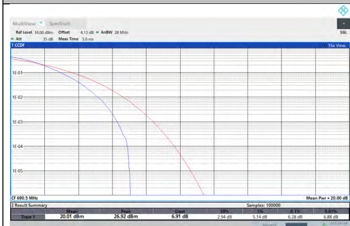
NTNV-N71-PC3-15-15-H-DFT-64QAM-Outer_Full-PASS
