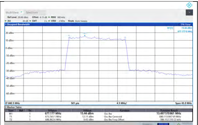
NTNV-N71-PC3-15-15-M-DFT-64QAM-Outer_Full-Ant1-PASS
