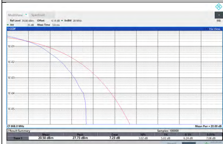
NTNV-N71-PC3-15-10-L-DFT-16QAM-Outer_Full-PASS
