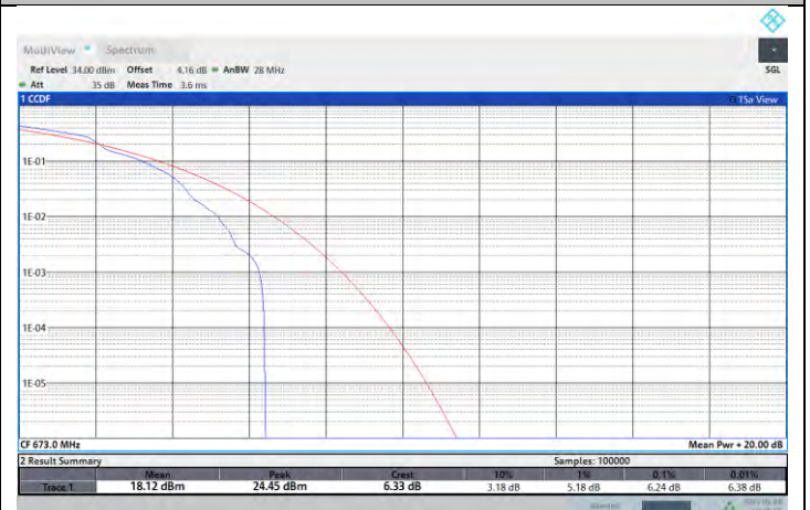
NTNV-N71-PC3-15-20-L-DFT-256QAM-Edge_1RB_Left-PASS
