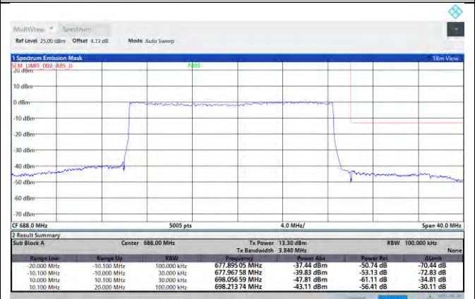
NTNV-N71-PC3-15-20-H-DFT-QPSK-Outer_Full-Ant1-PASS
