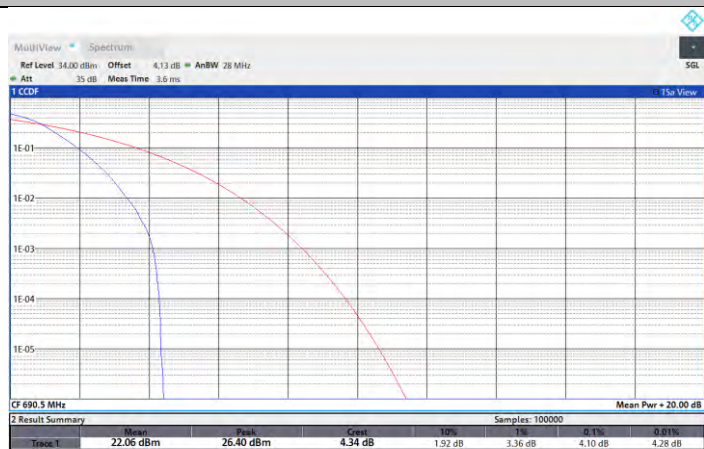
NTNV-N71-PC3-15-15-M-DFT-256QAM-Outer_Full-PASS
