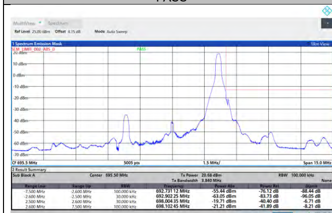
NTNV-N71-PC3-15-5-H-DFT-QPSK-Edge_1RB_Right-Ant1-PASS
