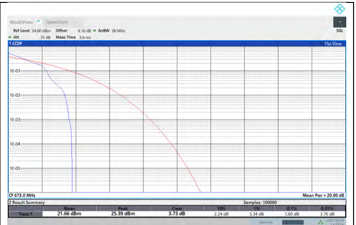
NTNV-N71-PC3-15-20-L-DFT-PI2BPSK-Edge_1RB_Left-PASS
