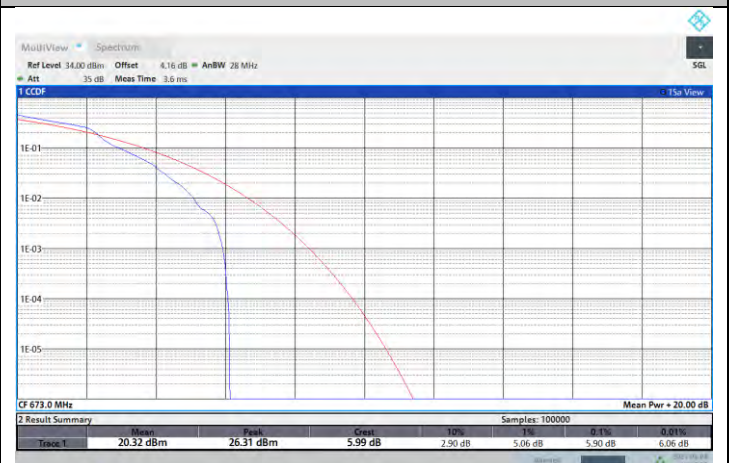
NTNV-N71-PC3-15-20-L-DFT-16QAM-Edge_1RB_Left-PASS
