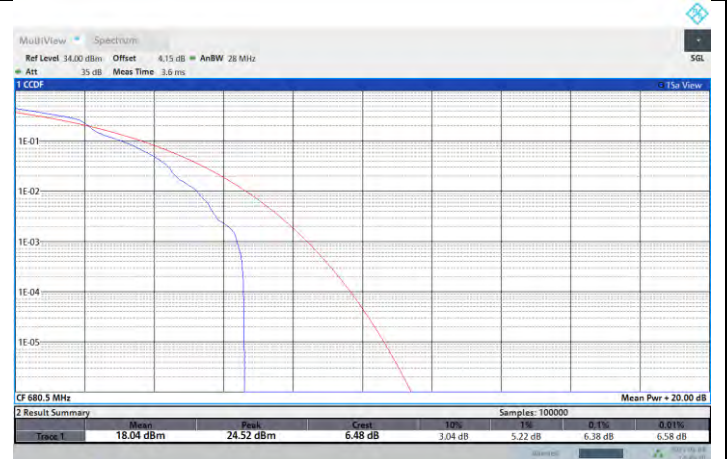
NTNV-N71-PC3-15-5-M-DFT-256QAM-Edge_1RB_Left-PASS
