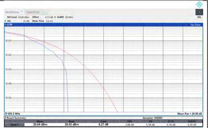
NTNV-N71-PC3-15-5-H-DFT-16QAM-Edge_1RB_Left-PASS
