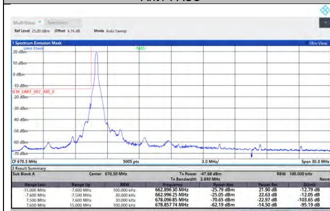
NTNV-N71-PC3-15-15-L-DFT-QPSK-Edge_1RB_Left-Ant1-PASS
