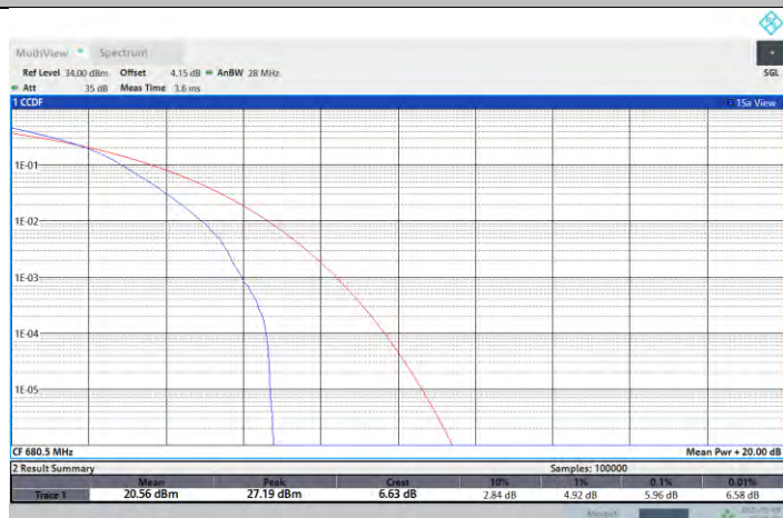
NTNV-N71-PC3-15-5-M-DFT-16QAM-Outer_Full-PASS
