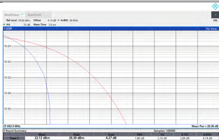
NTNV-N71-PC3-15-10-M-DFT-256QAM-Outer_Full-PASS
