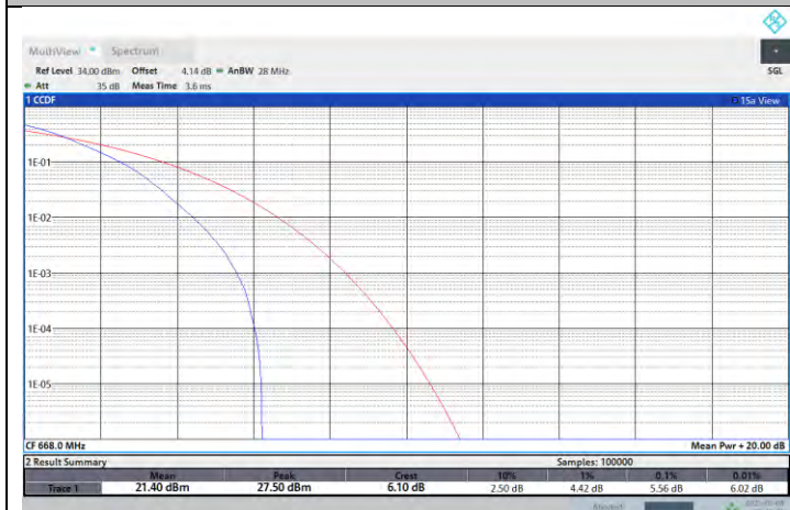
NTNV-N71-PC3-15-10-L-DFT-QPSK-Outer_Full-PASS
