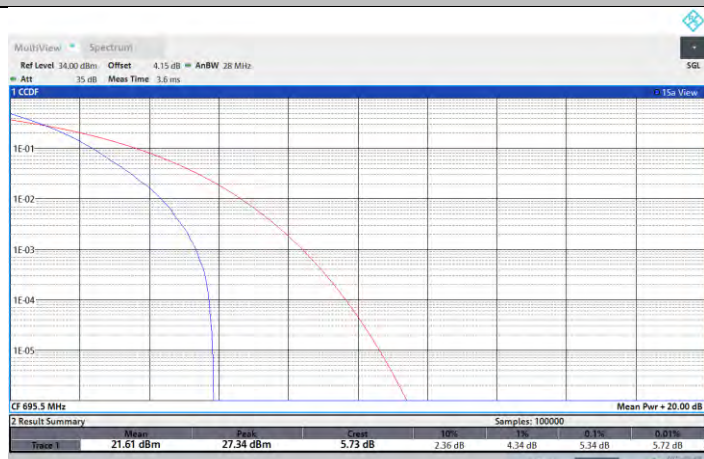
NTNV-N71-PC3-15-5-H-DFT-QPSK-Outer_Full-PASS
