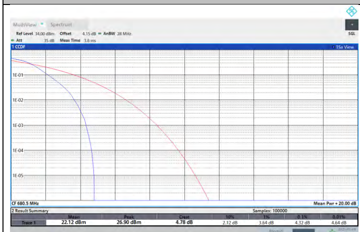
NTNV-N71-PC3-15-15-M-DFT-PI2BPSK-Outer_Full-PASS
