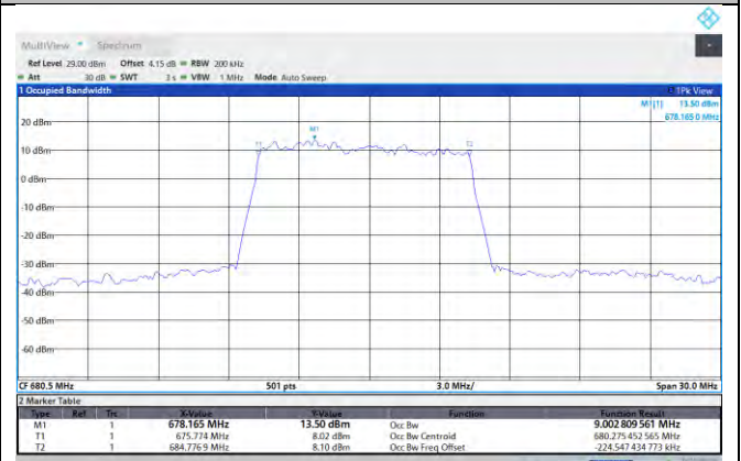
NTNV-N71-PC3-15-10-M-DFT-256QAM-Outet_Full-Ant1-PASS
