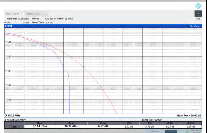
NTNV-N71-PC3-15-5-M-DFT-64QAM-Edge_1RB_Left-PASS
