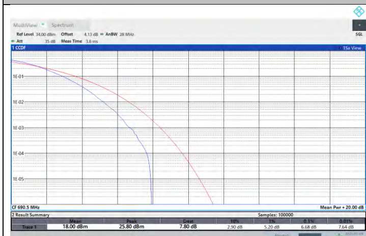
NTNV-N71-PC3-15-15-H-DFT-256QAM-Outer_Full-PASS
