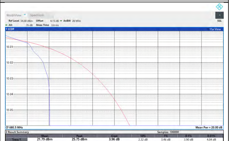
NTNV-N71-PC3-15-10-L-DFT-256QAM-Edge_1RB_Left-PASS
