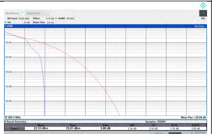
NTNV-N71-PC3-15-5-H-DFT-PI2BPSK-Edge_1RB_Left-PASS
