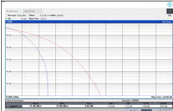
NTNV-N71-PC3-15-20-M-DFT-PI2BPSK-Outer_Full-PASS
