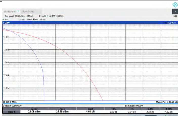
NTNV-N71-PC3-15-5-H-DFT-PI2BPSK-Outer_Full-PASS
