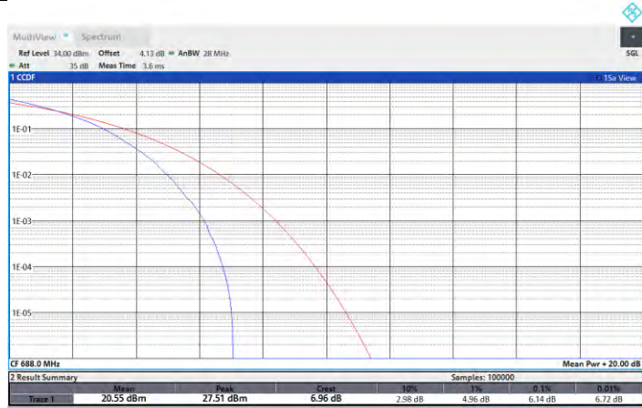
NTNV-N71-PC3-15-20-H-DFT-16QAM-Outer_Full-PASS
