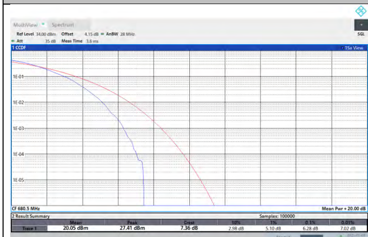
NTNV-N71-PC3-15-15-M-DFT-64QAM-Outer_Full-PASS
