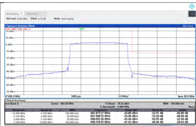
NTNV-N71-PC3-15-10-H-DFT-QPSK-Outer_Full-Ant1-PASS
