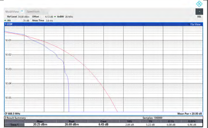
NTNV-N71-PC3-15-20-H-DFT-16QAM-Edge_1RB_Left-PASS
