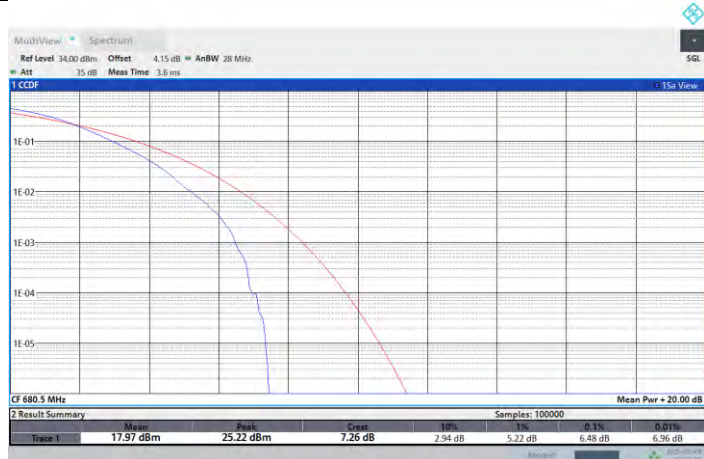
NTNV-N71-PC3-15-5-M-DFT-256QAM-Outer_Full-PASS
