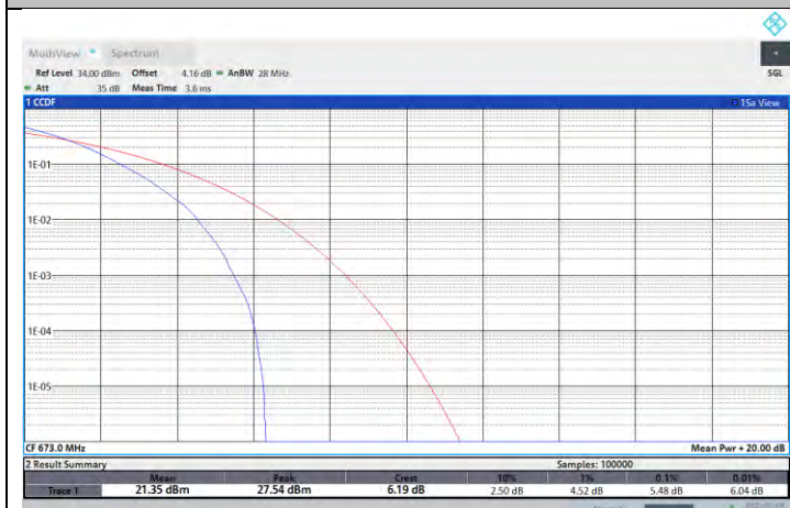
NTNV-N71-PC3-15-20-L-DFT-QPSK-Outer_Full-PASS
