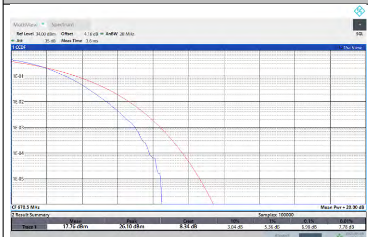
NTNV-N71-PC3-15-15-L-DFT-256QAM-Outer_Full-PASS
