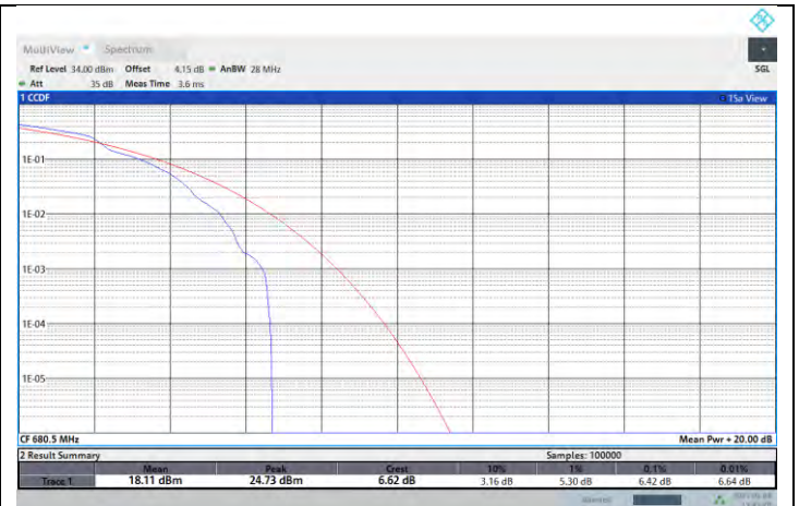
NTNV-N71-PC3-15-20-M-DFT-256QAM-Edge_1RB_Left-PASS
