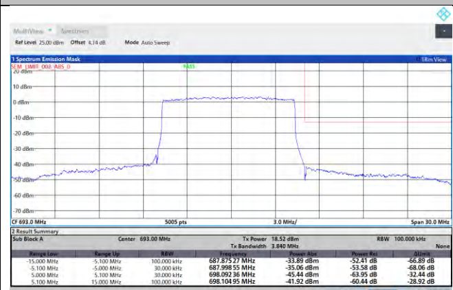
NTNV-N71-PC3-15-15-L-DFT-QPSK-Outer_Full-Ant1-PASS
