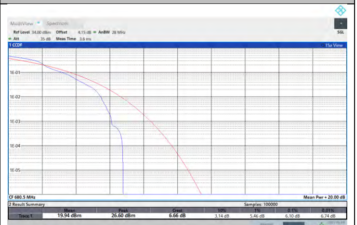
NTNV-N71-PC3-15-15-M-DFT-64QAM-Edge_1RB_Left-PASS
