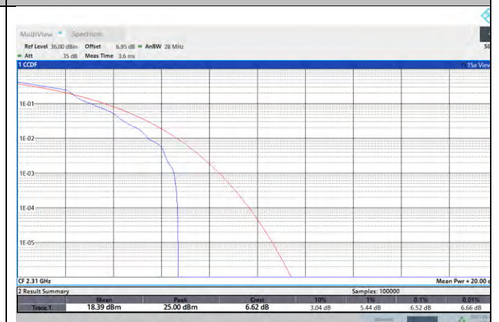
NTNV-N30-PC3-15-10-M-DFT-16QAM-Edge_1RB_Left-PASS
