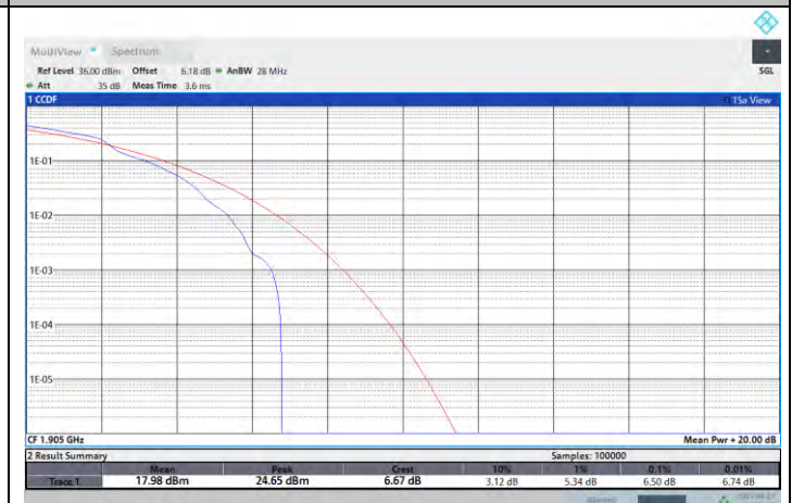
NTNV-N25-PC3-15-20-H-DFT-256QAM-Edge_1RB_Left-PASS
