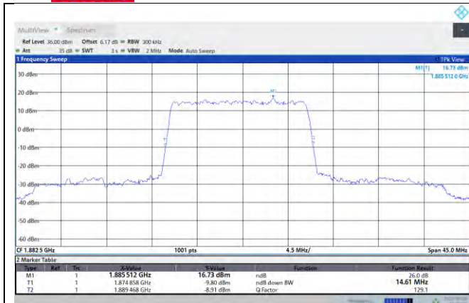
NTNV-N25-PC3-15-15-M-DFT-PI2BPSK-Outet_Full-Ant1-PASS
