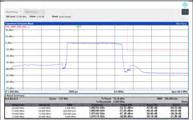
NTNV-N25-PC3-15-20-H-DFT-QPSK-Outer_Full-Ant1-PASS
