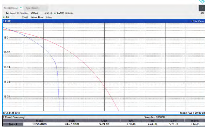
NTNV-N30-PC3-15-5-H-DFT-QPSK-Outer_Full-PASS
