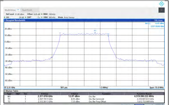
NTNV-N30-PC3-15-5-M-DFT-QPSK-Outet_Full-Ant1-PASS
