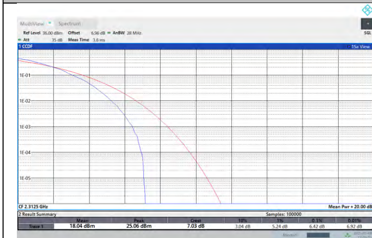
NTNV-N30-PC3-15-5-H-DFT-64QAM-Outer_Full-PASS
