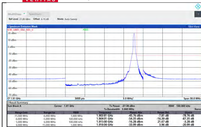
NTNV-N25-PC3-15-10-H-DFT-QPSK-Edge_1RB_Right-Ant1-PASS
