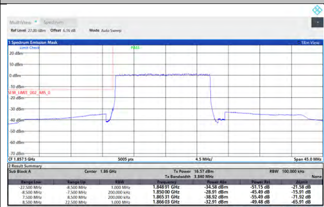
NTNV-N25-PC3-15-15-L-DFT-QPSK-Outer_Full-Ant1-PASS
