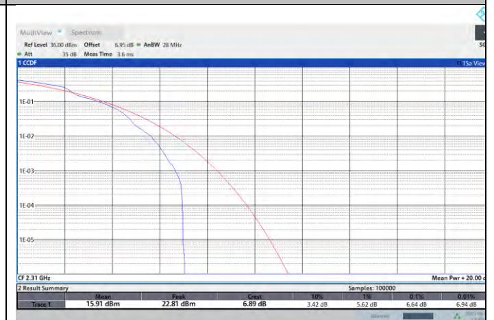
NTNV-N30-PC3-15-10-M-DFT-256QAM-Edge_1RB_Left-PASS
