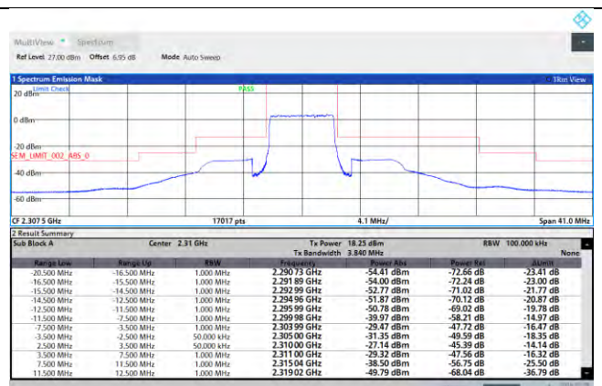
NTNV-N30-PC3-15-5-L-DFT-QPSK-Outer_Full-Ant1-PASS
