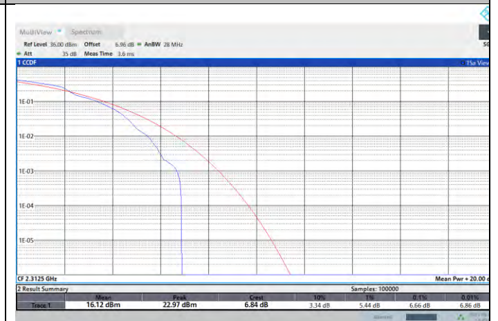
NTNV-N30-PC3-15-5-H-DFT-256QAM-Edge_1RB_Left-PASS
