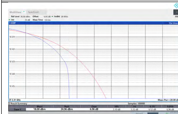
NTNV-N30-PC3-15-5-M-DFT-64QAM-Outer_Full-PASS
