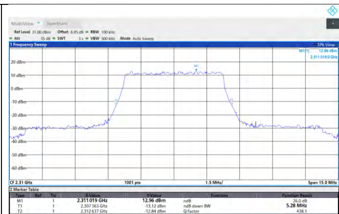
NTNV-N30-PC3-15-5-M-DFT-QPSK-Outer_Full-Ant1-PASS
