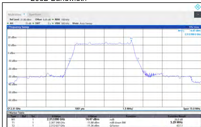
NTNV-N30-PC3-15-5-M-DFT-PI2BPSK-Outer_Full-Ant1-PASS
