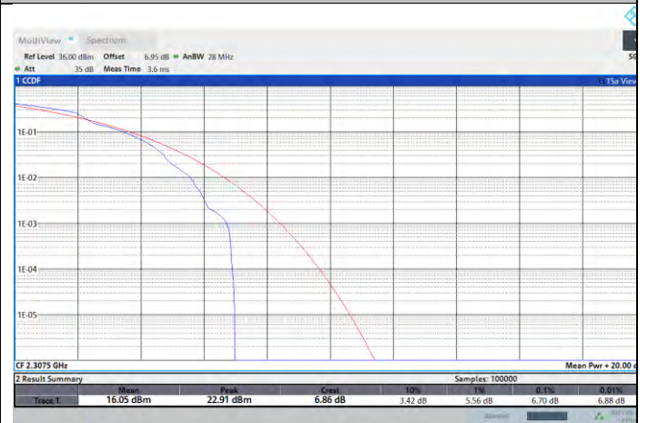
NTNV-N30-PC3-15-5-L-DFT-256QAM-Edge_1RB_Left-PASS
