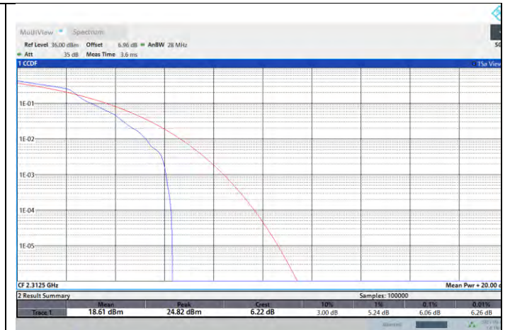
NTNV-N30-PC3-15-5-H-DFT-16QAM-Edge_1RB_Left-PASS
