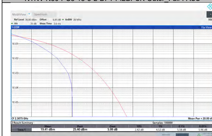
NTNV-N30-PC3-15-5-L-DFT-QPSK-Outer_Full-PASS
