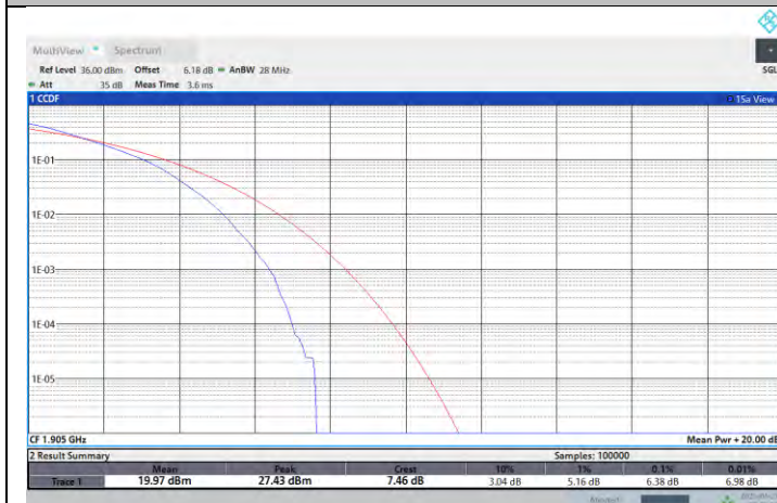
NTNV-N25-PC3-15-20-H-DFT-64QAM-Outer_Full-PASS
