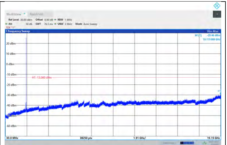
NTN-N25-PC3-15-15-M-DFT-QPSK-Edge_1RB_Left-Ant1-PASS
