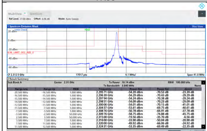
NTNV-N30-PC3-15-5-H-DFT-QPSK-Edge_1RB_Right-Ant1-PASS
