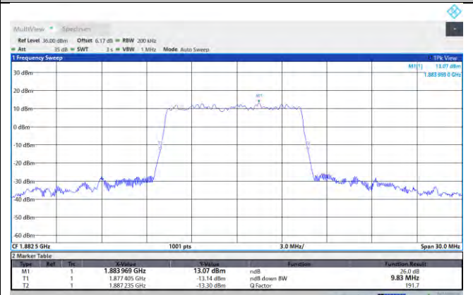
NTN-N25-PC3-15-10-M-DFT-256QAM-Outer_Full-Ant1-PASS
