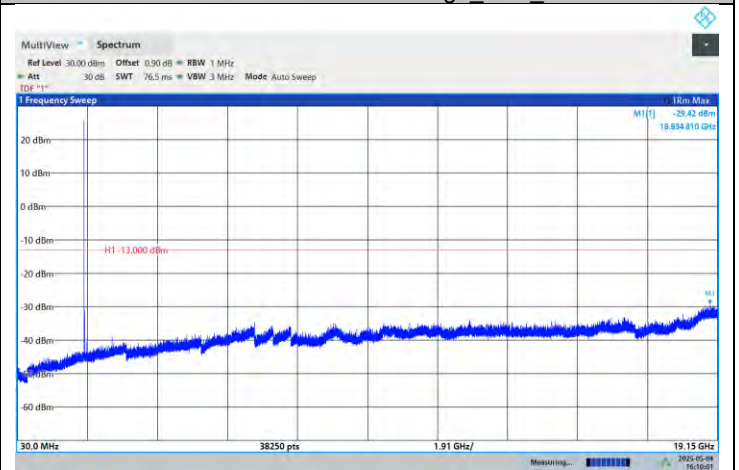
NTV-N25-PC3-15-10-L-DFT-QPSK-Edge_1RB_Left-Ant1-PASS
