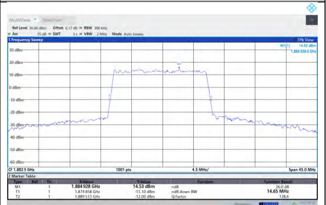
NTNV-N25-PC3-15-15-M-DFT-64QAM-Outet_Full-Ant1-PASS
