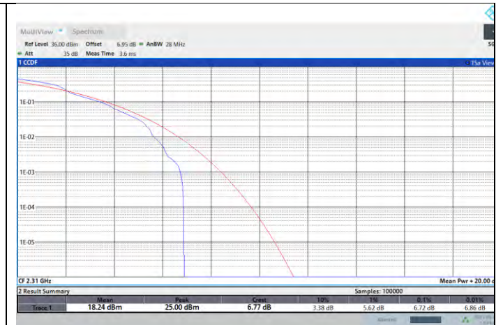
NTNV-N30-PC3-15-10-M-DFT-64QAM-Edge_1RB_Left-PASS
