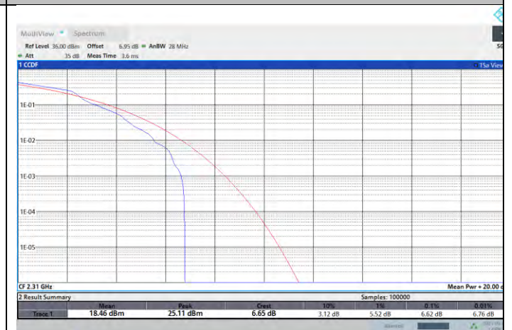
NTNV-N30-PC3-15-5-M-DFT-16QAM-Edge_1RB_Left-PASS
