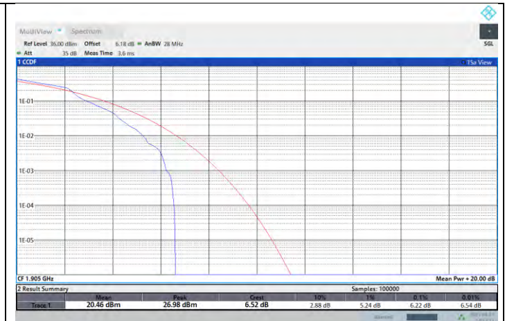
NTNV-N25-PC3-15-20-H-DFT-16QAM-Edge_1RB_Left-PASS
