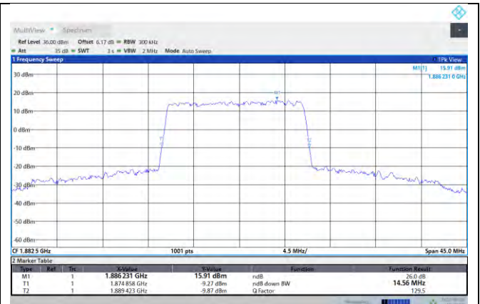
NTNV-N25-PC3-15-15-M-DFT-QPSK-Outet_Full-Ant1-PASS
