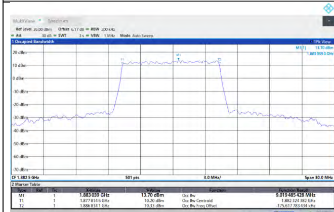
NTNV-N25-PC3-15-10-M-DFT-64QAM-Outet_Full-Ant1-PASS
