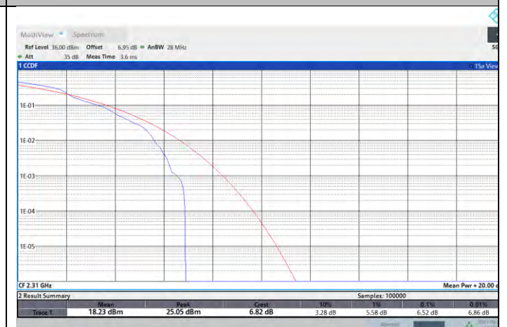
NTNV-N30-PC3-15-5-M-DFT-64QAM-Edge_1RB_Left-PASS
