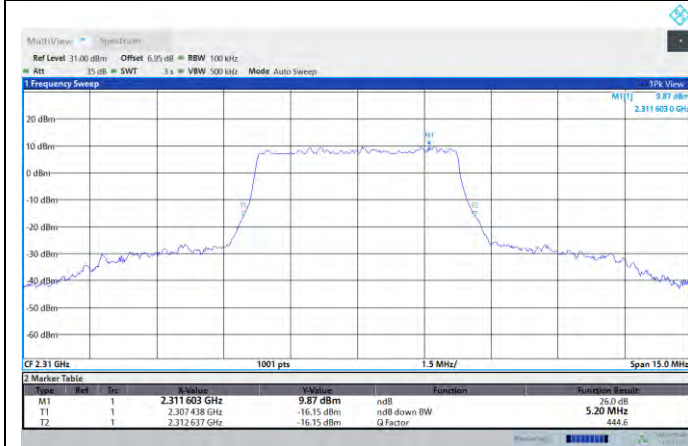
NTNV-N30-PC3-15-5-M-DFT-256QAM-Outer_Full-Ant1-PASS
