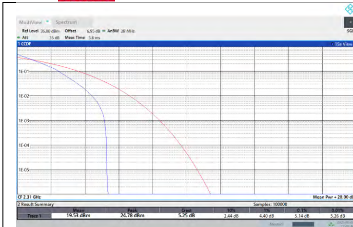
NTNV-N30-PC3-15-5-M-DFT-QPSK-Outer_Full-PASS
