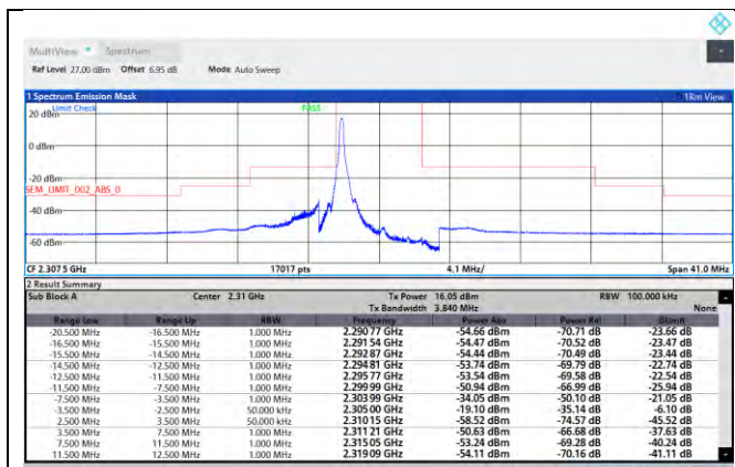
NTNV-N30-PC3-15-5-L-DFT-QPSK-Edge_1RB_Left-Ant1-PASS
