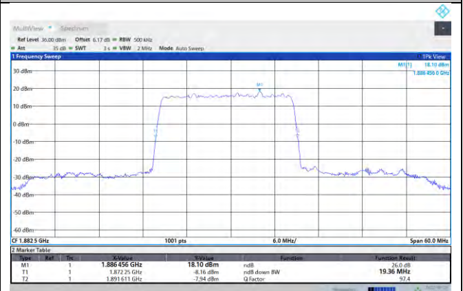
NTNV-N25-PC3-15-20-M-DFT-PI2BPSK-Outet_Full-Ant1-PASS
