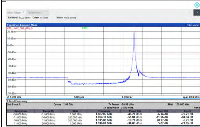
NTNV-N25-PC3-15-20-H-DFT-QPSK-Edge_1RB_Right-Ant1-PASS
