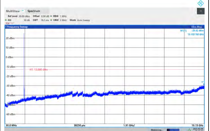
NTN-N25-PC3-15-20-L-DFT-QPSK-Edge_1RB_Left-Ant1-PASS
