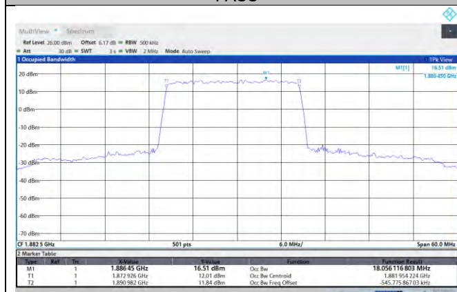
NTNV-N25-PC3-15-20-M-DFT-QPSK-Outer_Full-Ant1-PASS
