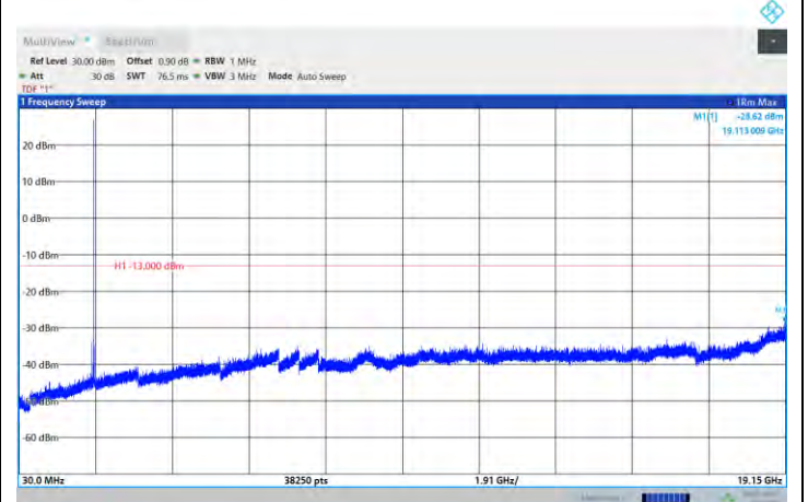
NTN-N25-PC3-15-20-H-DFT-QPSK-Edge_1RB_Left-Ant1-PASS
