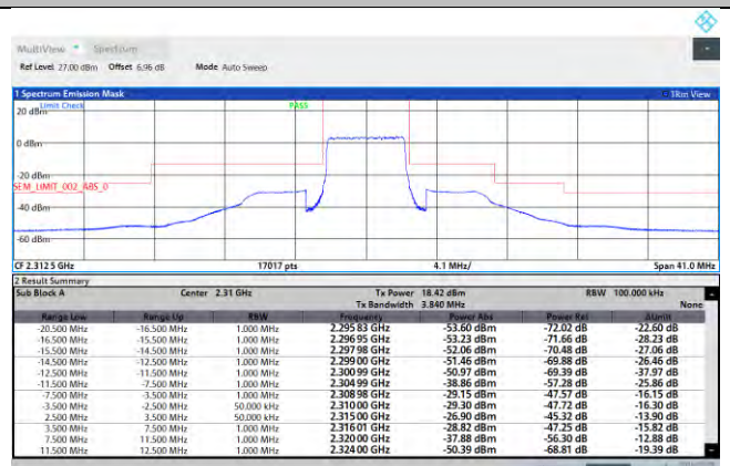
NTNV-N30-PC3-15-5-H-DFT-QPSK-Outer_Full-Ant1-PASS
