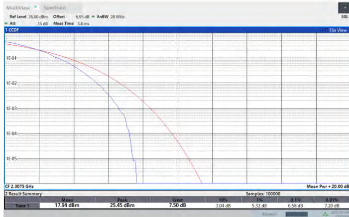
NTNV-N30-PC3-15-5-L-DFT-64QAM-Outer_Full-PASS
