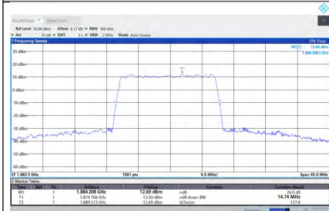
NTNV-N25-PC3-15-15-M-DFT-256QAM-Outet_Full-Ant1-PASS
