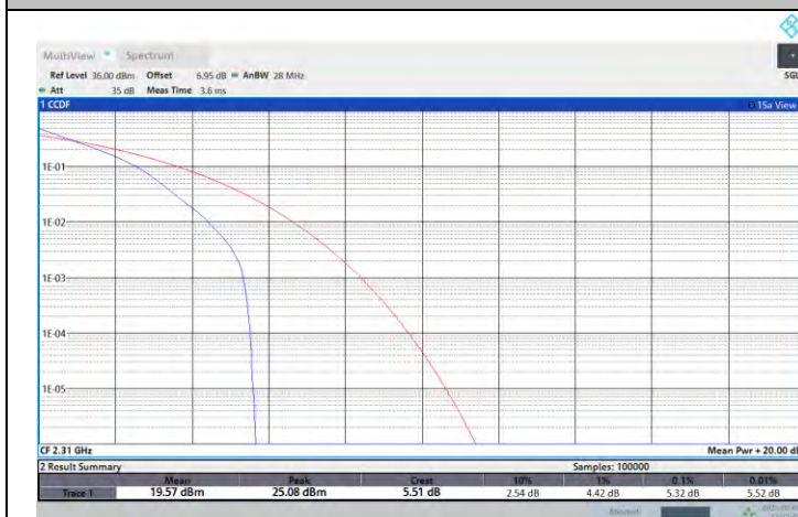
NTNV-N30-PC3-15-10-M-DFT-QPSK-Outer_Full-PASS
