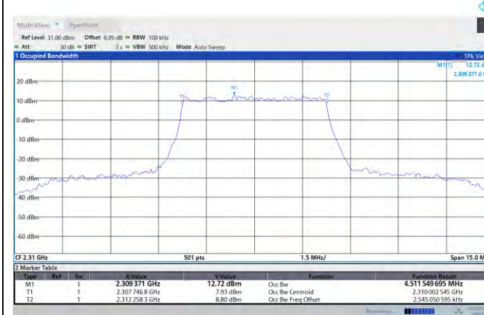
NTNV-N30-PC3-15-5-M-DFT-16QAM-Outet_Full-Ant1-PASS
