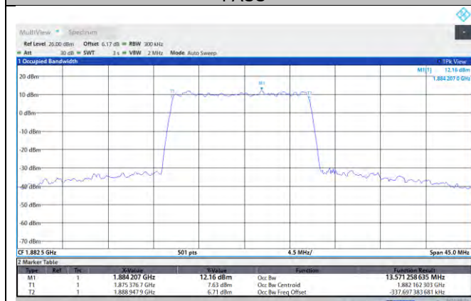
NTNV-N25-PC3-15-15-M-DFT-256QAM-Outer_Full-Ant1-PASS
