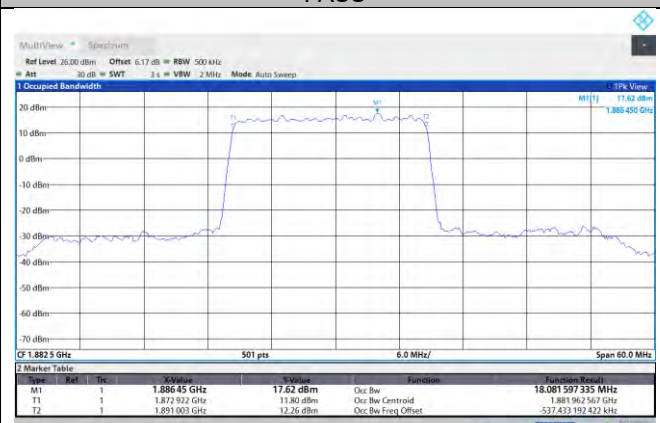
NTNV-N25-PC3-15-20-M-DFT-PI2BPSK-Outer_Full-Ant1-PASS
