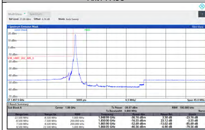
NTNV-N25-PC3-15-15-L-DFT-QPSK-Edge_1RB_Left-Ant1-PASS
