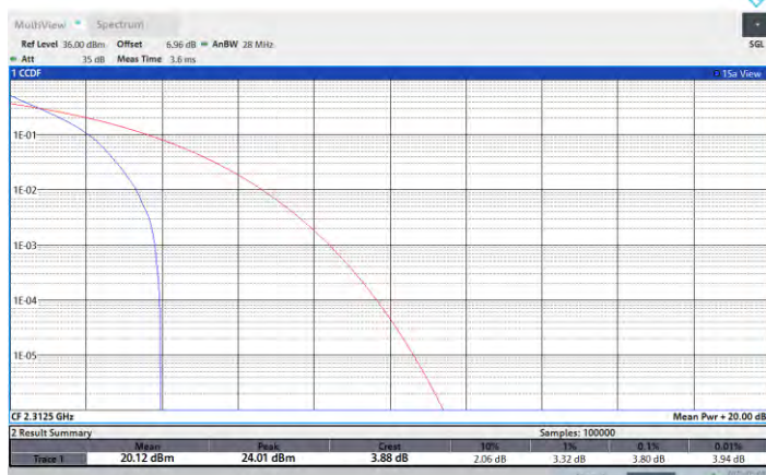
NTNV-N30-PC3-15-5-H-DFT-PI2BPSK-Outer_Full-PASS
