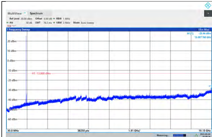
NTV-N25-PC3-15-5-L-DFT-QPSK-Edge_1RB_Left-Ant1-PASS
