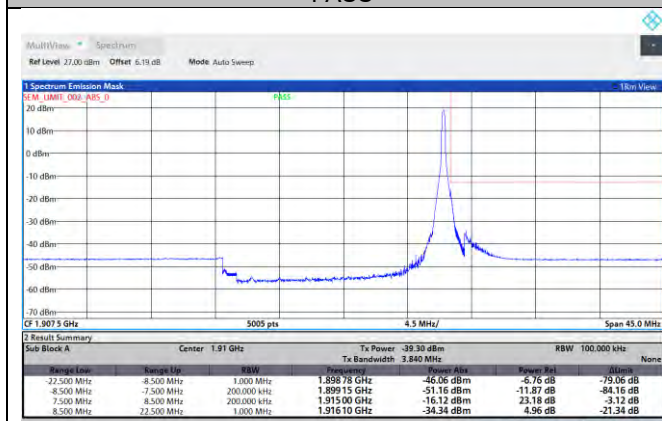
NTNV-N25-PC3-15-15-H-DFT-QPSK-Edge_1RB_Right-Ant1-PASS
