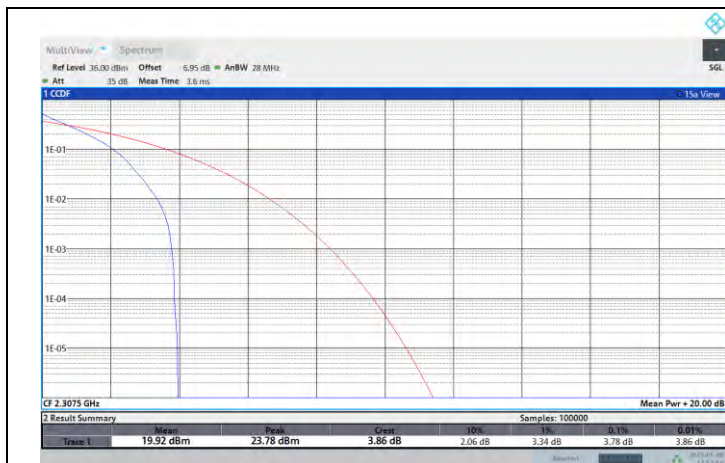
NTNV-N30-PC3-15-5-L-DFT-PI2BPSK-Outer_Full-PASS
