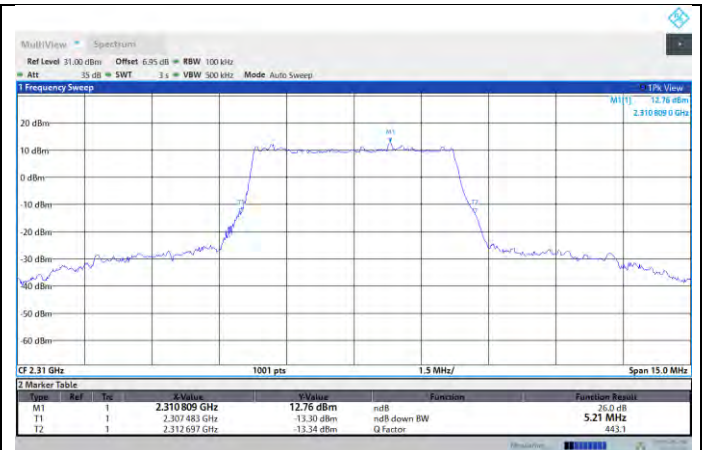
NTNV-N30-PC3-15-5-M-DFT-64QAM-Outer_Full-Ant1-PASS
