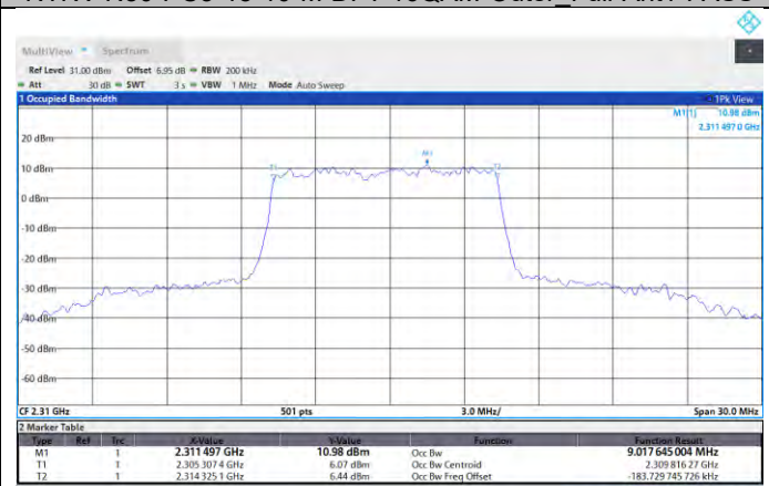
NTNV-N30-PC3-15-10-M-DFT-256QAM-Outer_Full-Ant1-PASS
