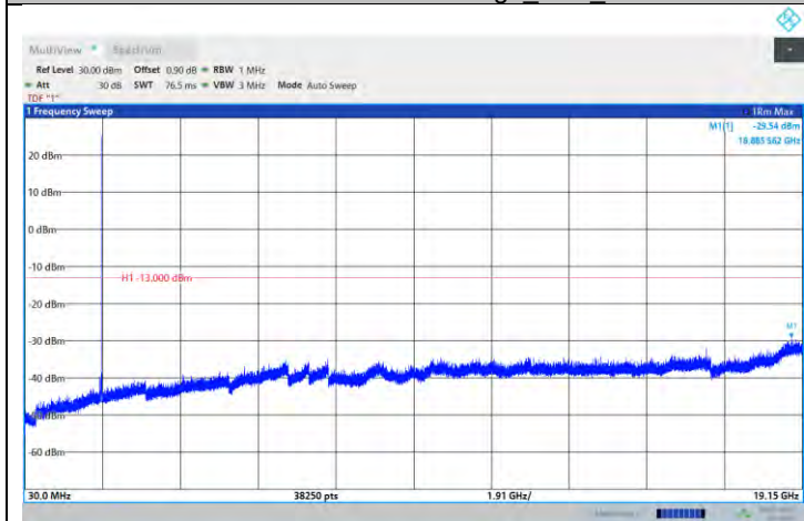
NTV-N25-PC3-15-5-H-DFT-QPSK-Edge_1RB_Left-Ant1-PASS
