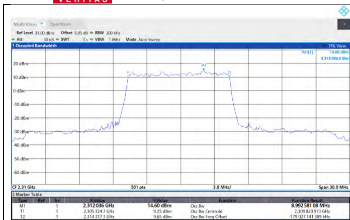
NTNV-N30-PC3-15-10-M-DFT-QPSK-Outer_Full-Ant1-PASS
