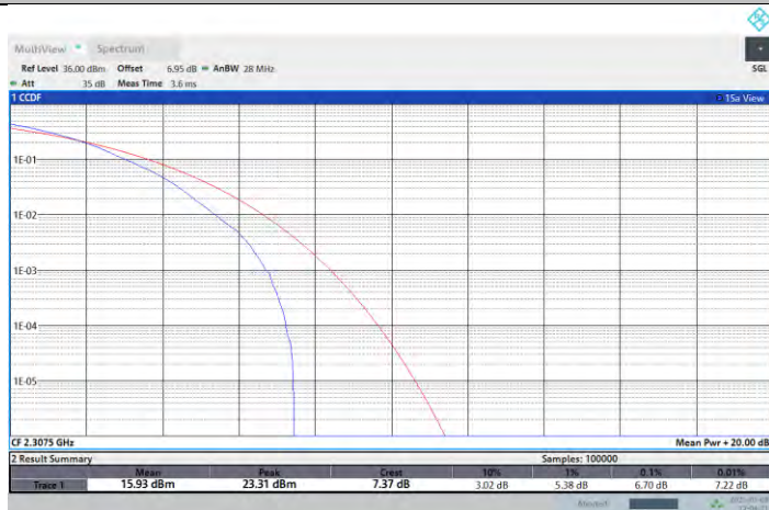
NTNV-N30-PC3-15-5-L-DFT-256QAM-Outer_Full-PASS
