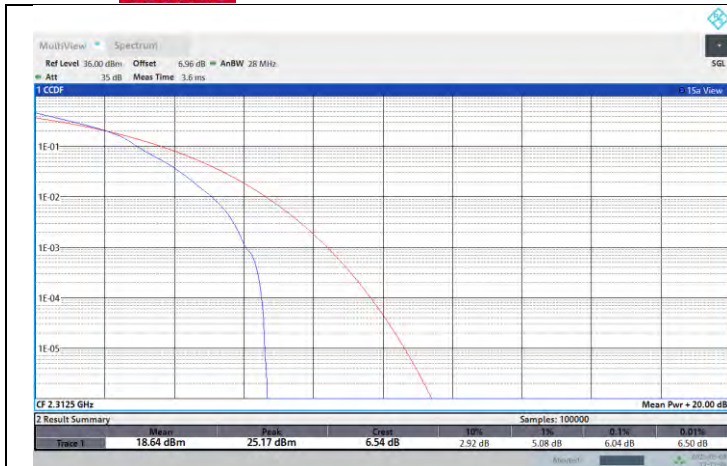
NTNV-N30-PC3-15-5-H-DFT-16QAM-Outer_Full-PASS
