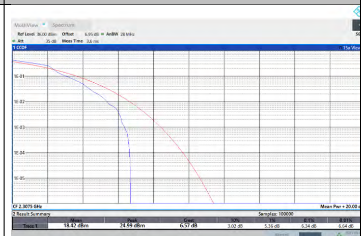
NTNV-N30-PC3-15-5-L-DFT-16QAM-Edge_1RB_Left-PASS
