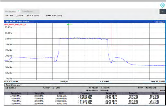
NTNV-N25-PC3-15-15-H-DFT-QPSK-Outer_Full-Ant1-PASS
