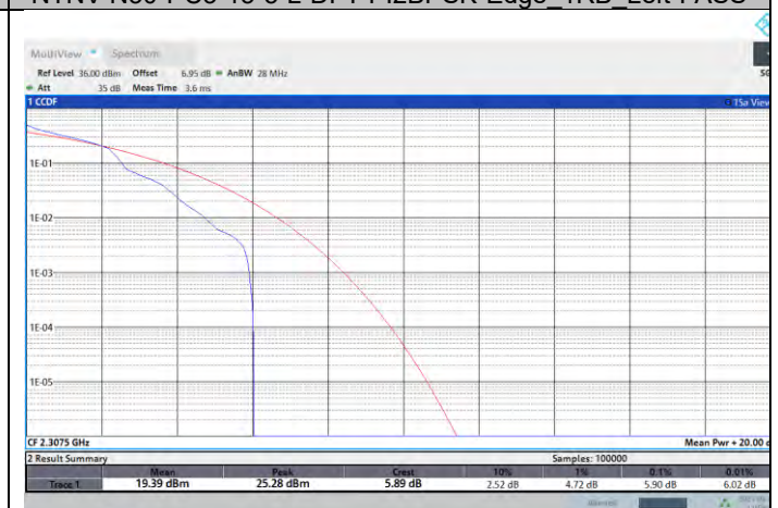
NTNV-N30-PC3-15-5-L-DFT-QPSK-Edge_1RB_Left-PASS
