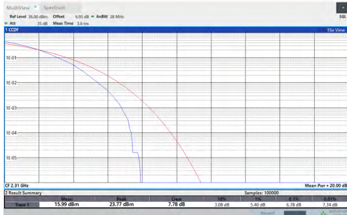
NTNV-N30-PC3-15-5-M-DFT-256QAM-Outer_Full-PASS
