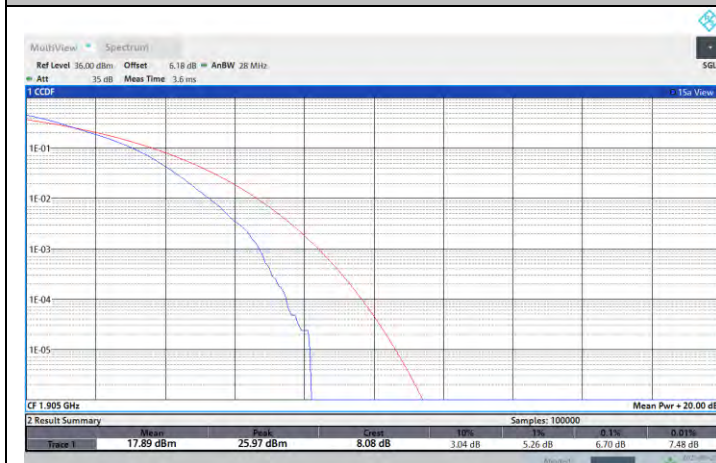
NTNV-N25-PC3-15-20-H-DFT-256QAM-Outer_Full-PASS
