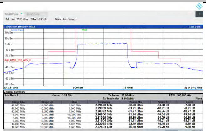
NTNV-N30-PC3-15-10-M-DFT-QPSK-Outer_Full-Ant1-PASS
