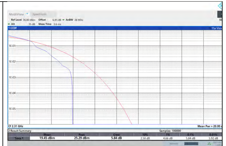
NTNV-N30-PC3-15-5-M-DFT-QPSK-Edge_1RB_Left-PASS
