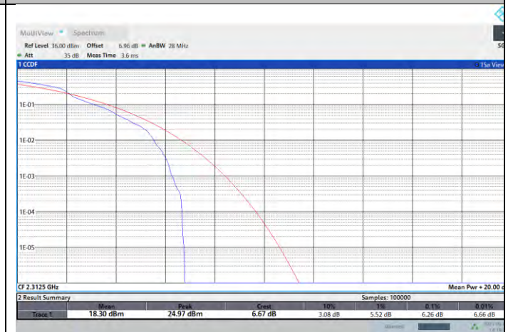
NTNV-N30-PC3-15-5-H-DFT-64QAM-Edge_1RB_Left-PASS
