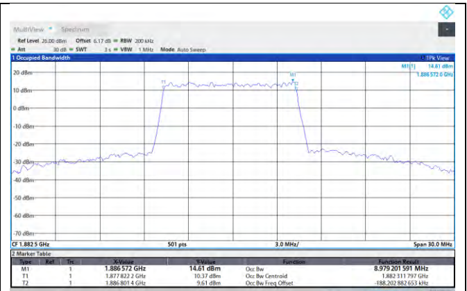
NTNV-N25-PC3-15-10-M-DFT-16QAM-Outet_Full-Ant1-PASS
