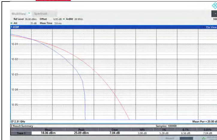
NTNV-N30-PC3-15-10-M-DFT-64QAM-Outer_Full-PASS
