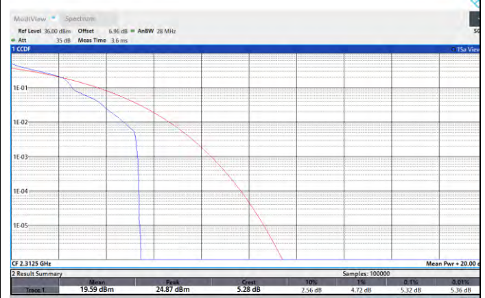
NTNV-N30-PC3-15-5-H-DFT-QPSK-Edge_1RB_Left-PASS
