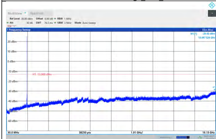
NTV-N25-PC3-15-10-M-DFT-QPSK-Edge_1RB_Left-Ant1-PASS
