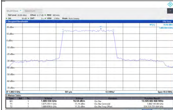
NTNV-N25-PC3-15-15-M-DFT-PI2BPSK-Outet_Full-Ant1-PASS
