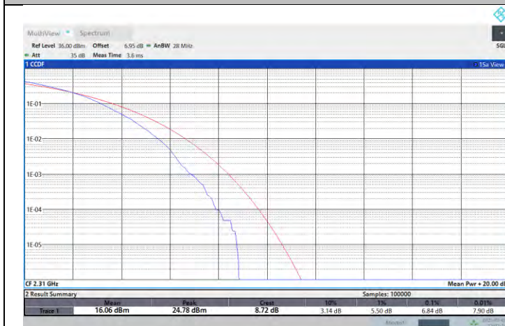
NTNV-N30-PC3-15-10-M-DFT-256QAM-Outer_Full-PASS
