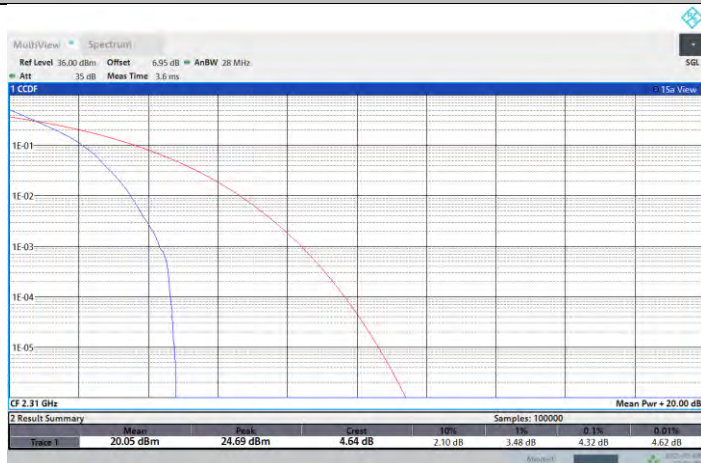
NTNV-N30-PC3-15-5-M-DFT-PI2BPSK-Outer_Full-PASS
