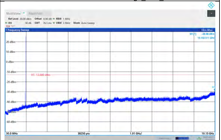
NTV-N25-PC3-15-10-H-DFT-QPSK-Edge_1RB_Left-Ant1-PASS
