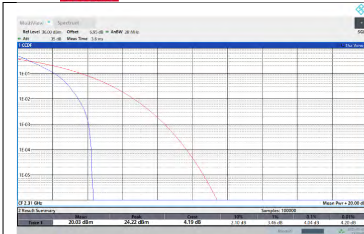
NTNV-N30-PC3-15-10-M-DFT-PI2BPSK-Outer_Full-PASS
