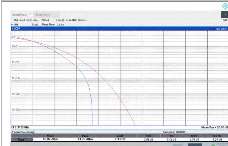
NTNV-N30-PC3-15-5-H-DFT-256QAM-Outer_Full-PASS
