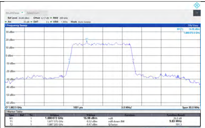
NTN-N25-PC3-15-10-M-DFT-PI2BPSK-Outer_Full-Ant1-PASS
