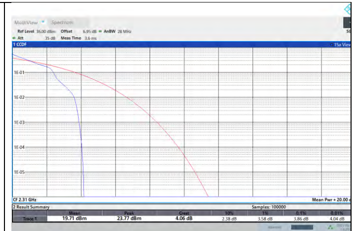
NTNV-N30-PC3-15-10-M-DFT-PI2BPSK-Edge_1RB_Left-PASS
