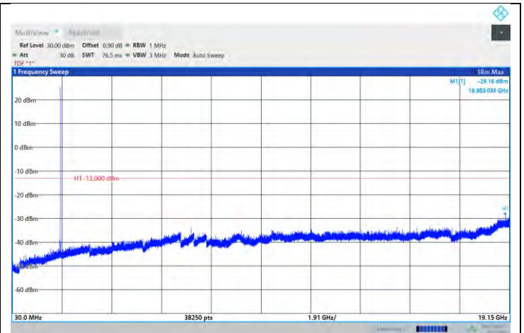
NTV-N25-PC3-15-5-M-DFT-QPSK-Edge_1RB_Left-Ant1-PASS
