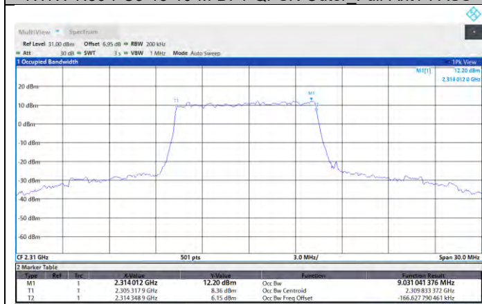
NTNV-N30-PC3-15-10-M-DFT-64QAM-Outer_Full-Ant1-PASS
