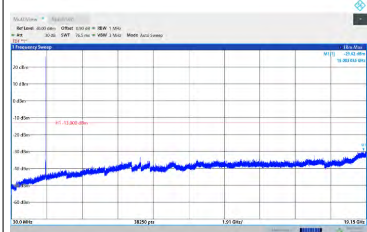
NTN-N25-PC3-15-20-M-DFT-QPSK-Edge_1RB_Left-Ant1-PASS
