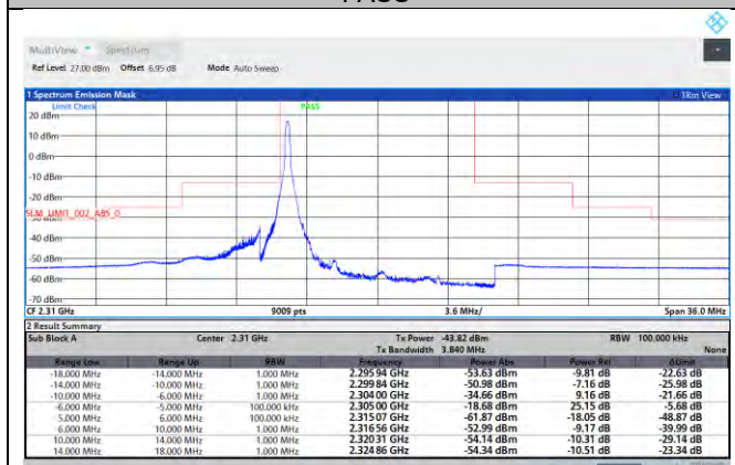
NTNV-N30-PC3-15-10-M-DFT-QPSK-Edge_1RB_Left-Ant1-PASS
