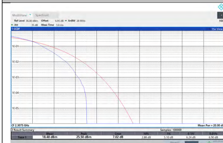
NTNV-N30-PC3-15-5-L-DFT-16QAM-Outer_Full-PASS
