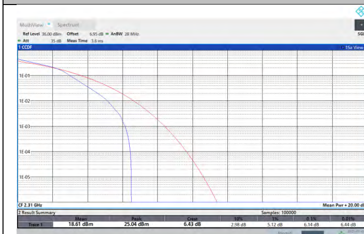
NTNV-N30-PC3-15-10-M-DFT-16QAM-Outer_Full-PASS
