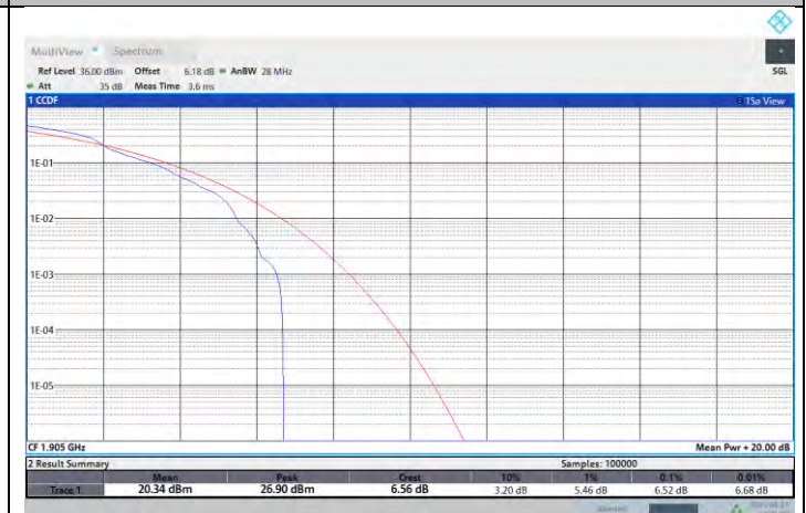
NTNV-N25-PC3-15-20-H-DFT-64QAM-Edge_1RB_Left-PASS
