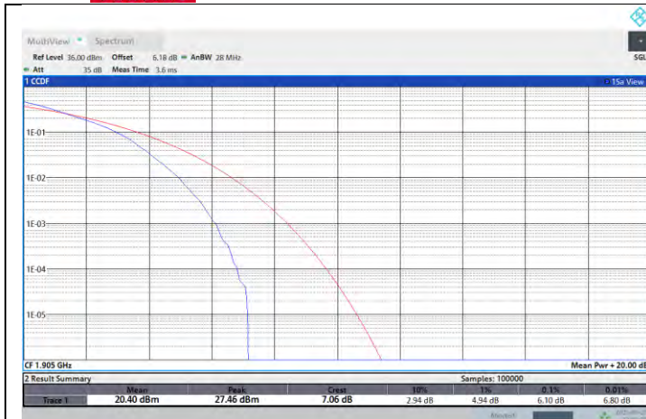
NTNV-N25-PC3-15-20-H-DFT-16QAM-Outer_Full-PASS
