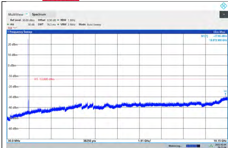
NTN-N25-PC3-15-15-L-DFT-QPSK-Edge_1RB_Left-Ant1-PASS
