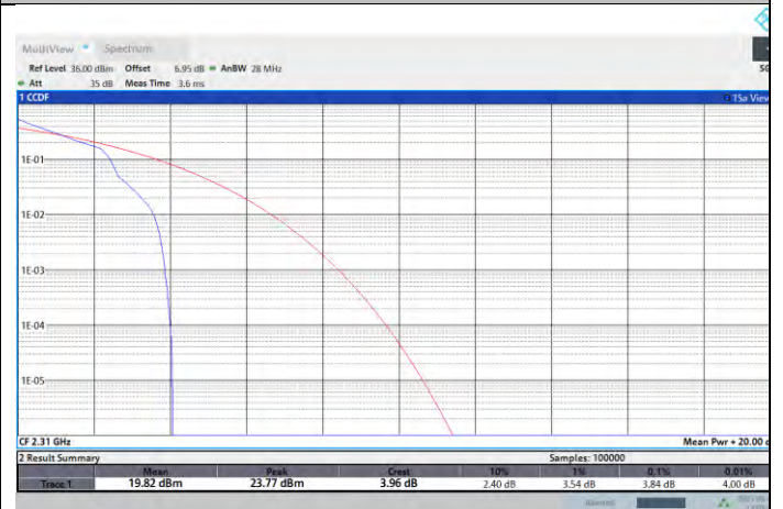
NTNV-N30-PC3-15-5-M-DFT-PI2BPSK-Edge_1RB_Left-PASS
