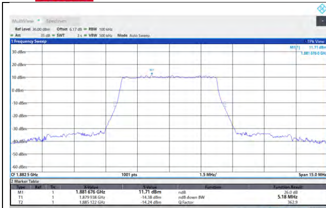
NTN-N25-PC3-15-5-M-DFT-256QAM-Outer_Full-Ant1-PASS
