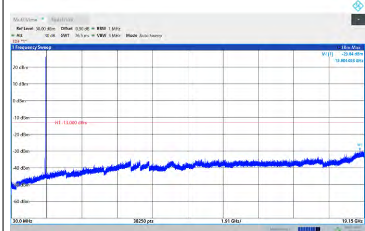
NTN-N25-PC3-15-15-H-DFT-QPSK-Edge_1RB_Left-Ant1-PASS
