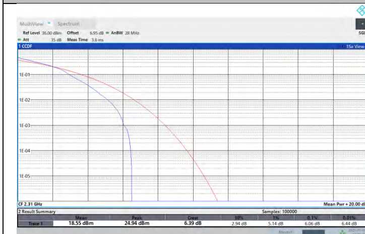
NTNV-N30-PC3-15-5-M-DFT-16QAM-Outer_Full-PASS
