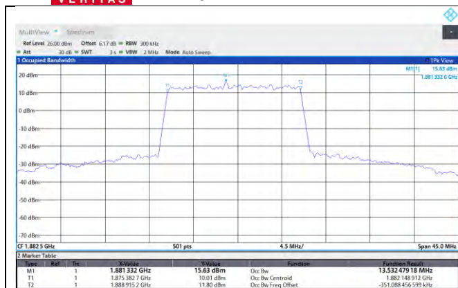
NTNV-N25-PC3-15-15-M-DFT-16QAM-Outer_Full-Ant1-PASS
