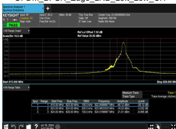
N5(20M)_DFT-s- OFDM_BPSK_Edge_1RB_Left_Low_CH
