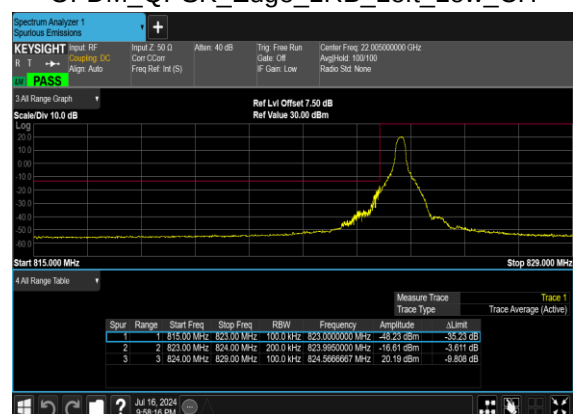
N5(20M)_DFT-s- OFDM_QPSK_Edge_1RB_Left_Low_CH
