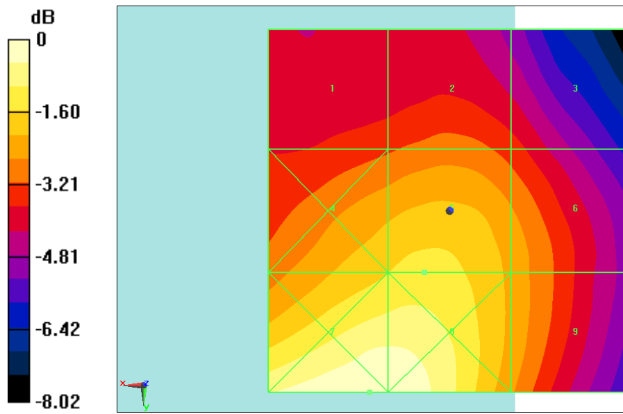
Fig B.3 HAC RF E-Field LTE Band41 QPSK CH41490
