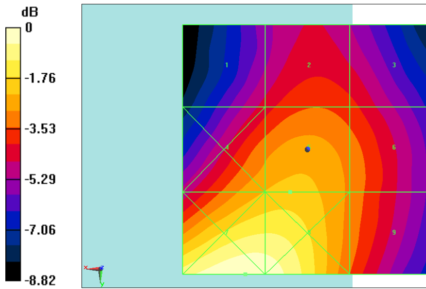
Fig B.4 HAC RF E-Field LTE Band41 QPSK CH41055
