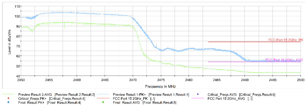
Fig.A.6.2.8 Transmitter Spurious Emission - Radiated (Power): 802.11n-HT40, ch9, 2.45 GHz - 2.50GHz
