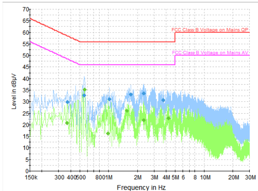
Fig.B.11.2 AC Powerline Conducted Emission-Idle
