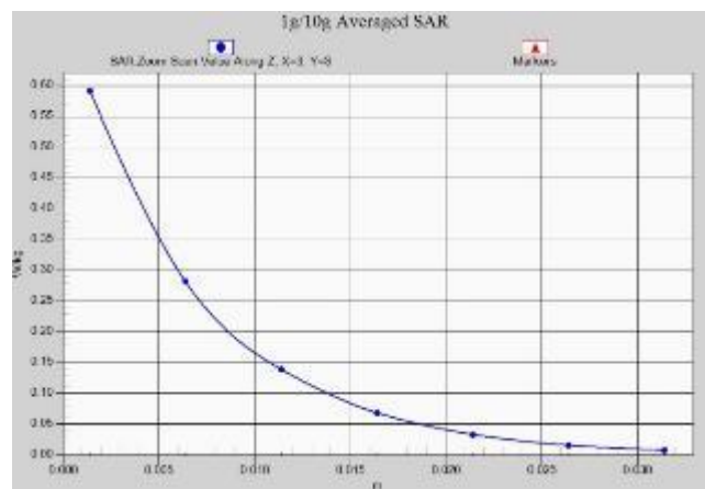
Fig. 1-30 Z-Scan at power reference point mimo (wifi2450)
