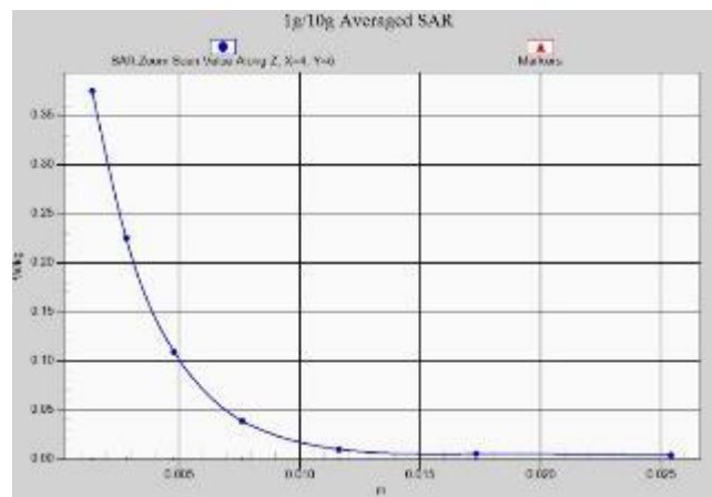
Fig. 1-36 Z-Scan at power reference point (wifi5G)
