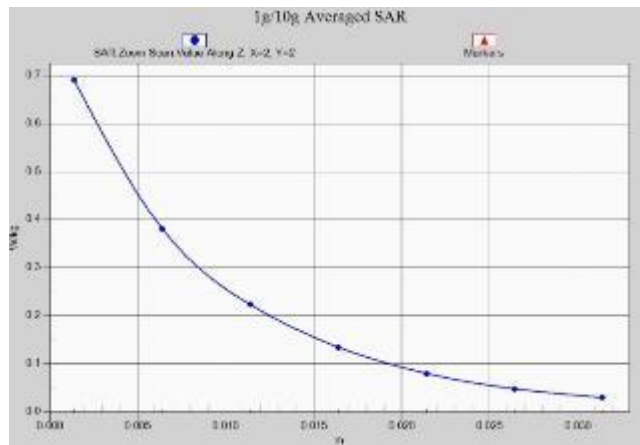
Fig. 1-18 Z-Scan at power reference point (LTE Band66)
