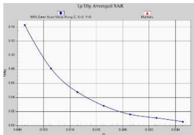
Fig. 1-24 Z-Scan at power reference point (N7 Antenna1)
