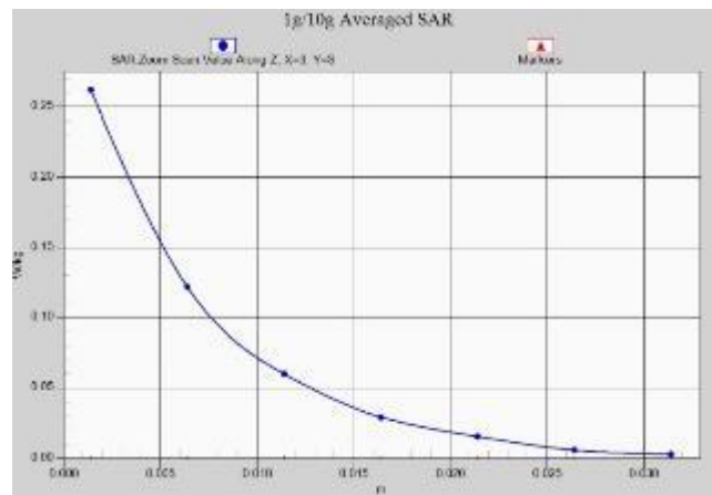
Fig. 1-28 Z-Scan at power reference point (wifi2450)
