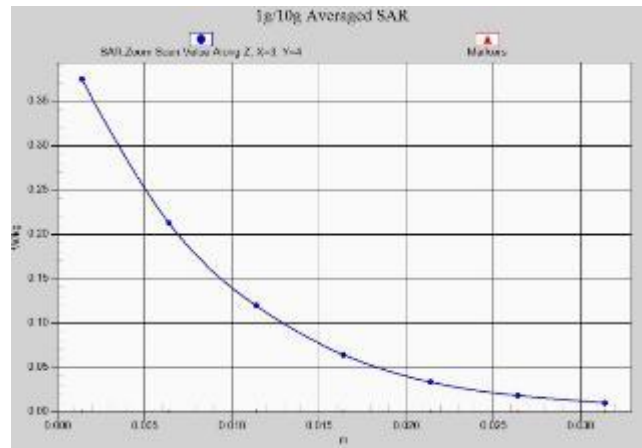
Fig. 1-25 Z-Scan at power reference point (N7 Antenna1)
