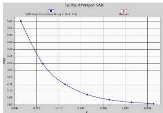
Fig. 1-23 Z-Scan at power reference point (N7 Antenna2)
