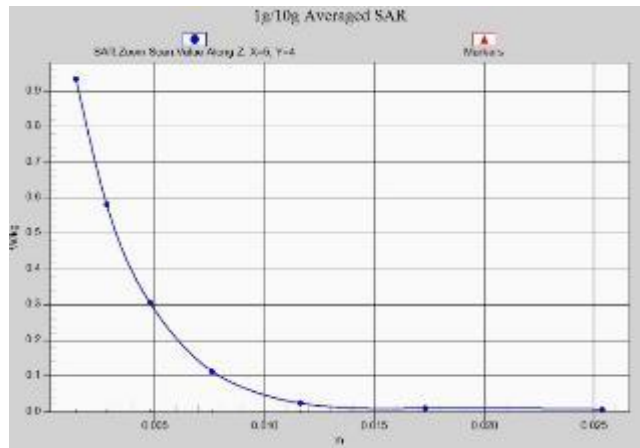
Fig. 1-31 Z-Scan at power reference point (wifi5G)
