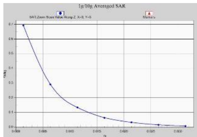
Fig. 1-29 Z-Scan at power reference point mimo (wifi2450 )
