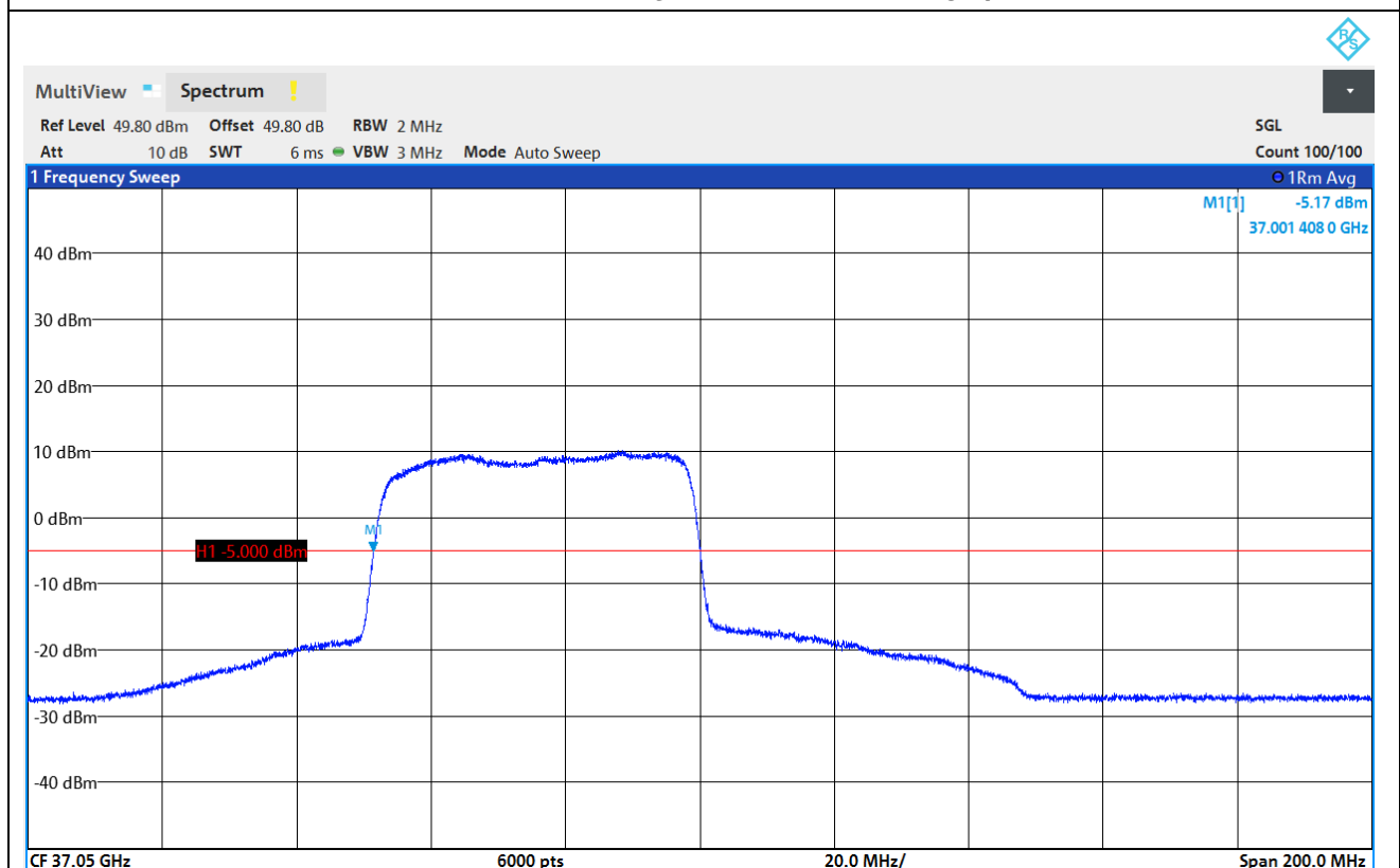
Worst case 100MHz QPSK Low channel edge plot
