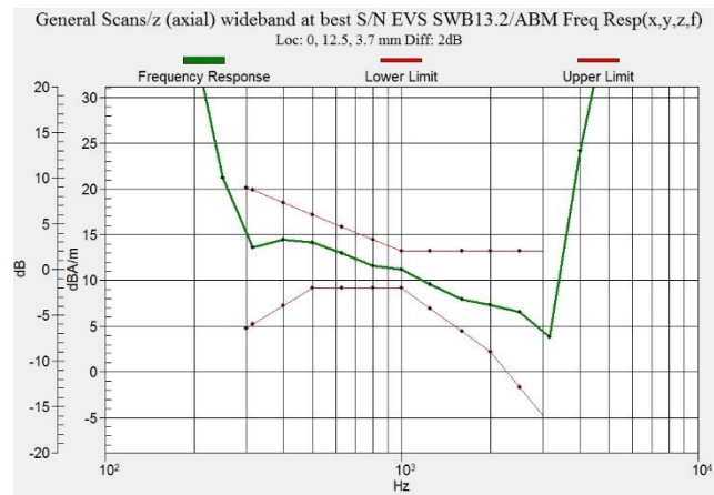
Figure C.4 Frequency Response of LTE B41 PC2
