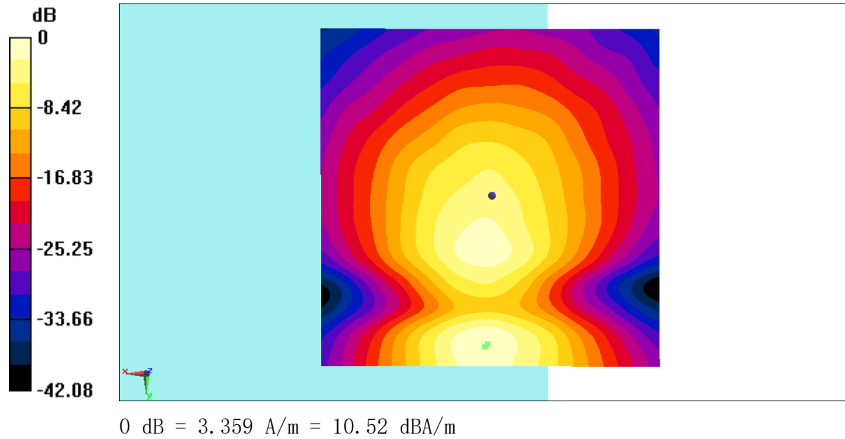
Fig B.7 T-Coil LTE B41 PC3
