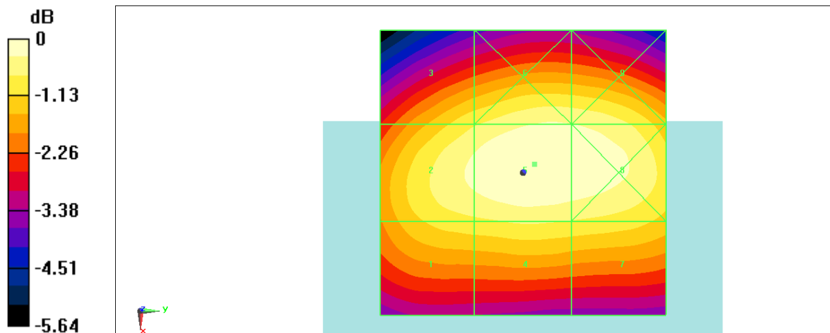
Fig B.1 HAC RF E-Field GSM 850 Middle
