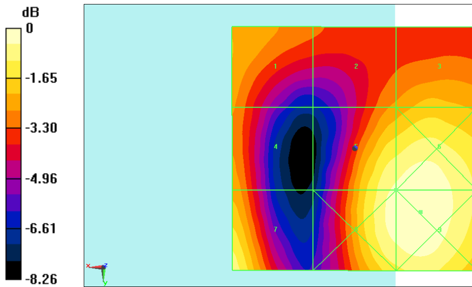
Fig B.3 HAC RF E-Field LTE Band41 Power Class 2 QPSK CH41490
