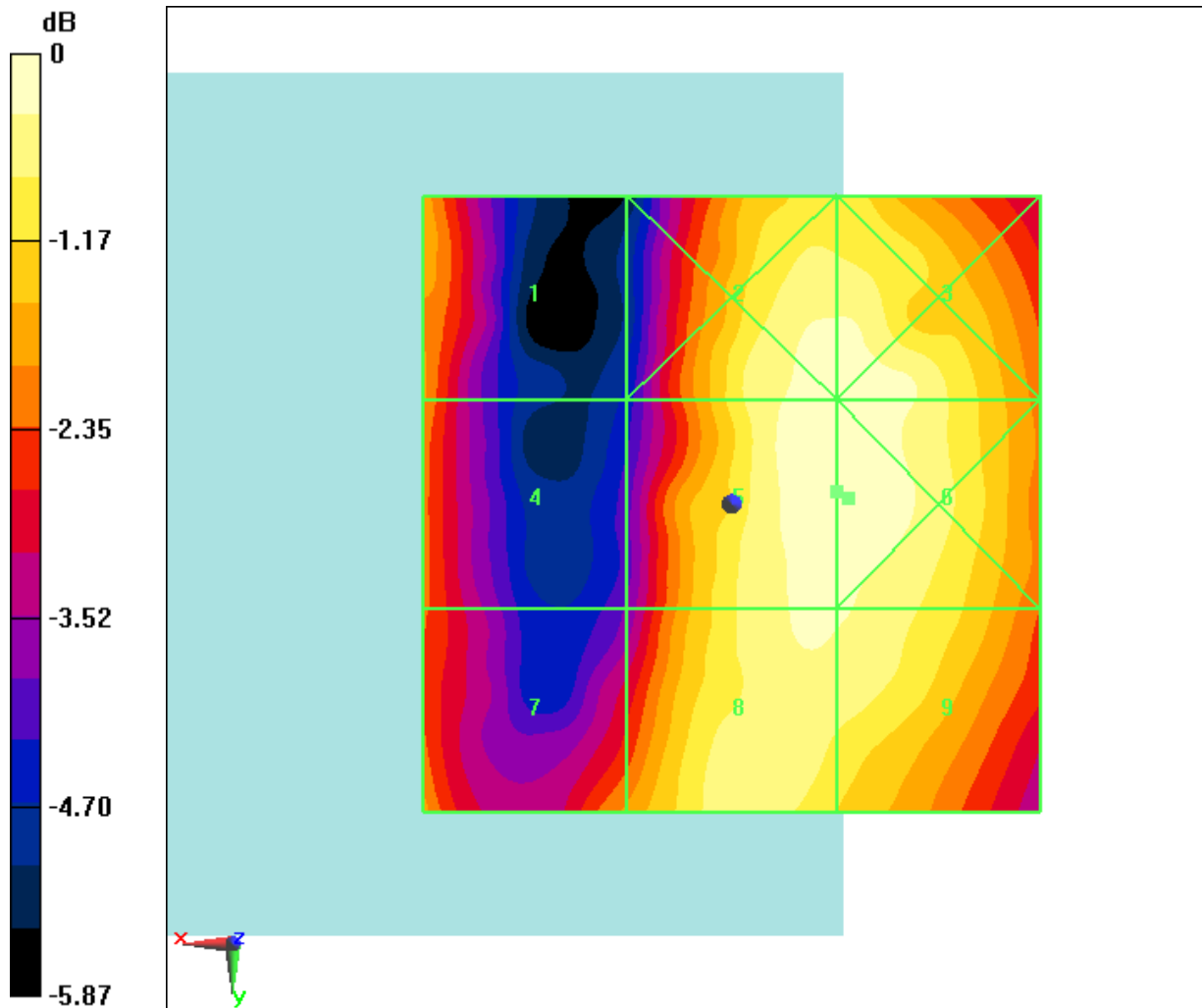
Fig B.21 HAC RF E-Field LTE Band41 64QAM CH39750
