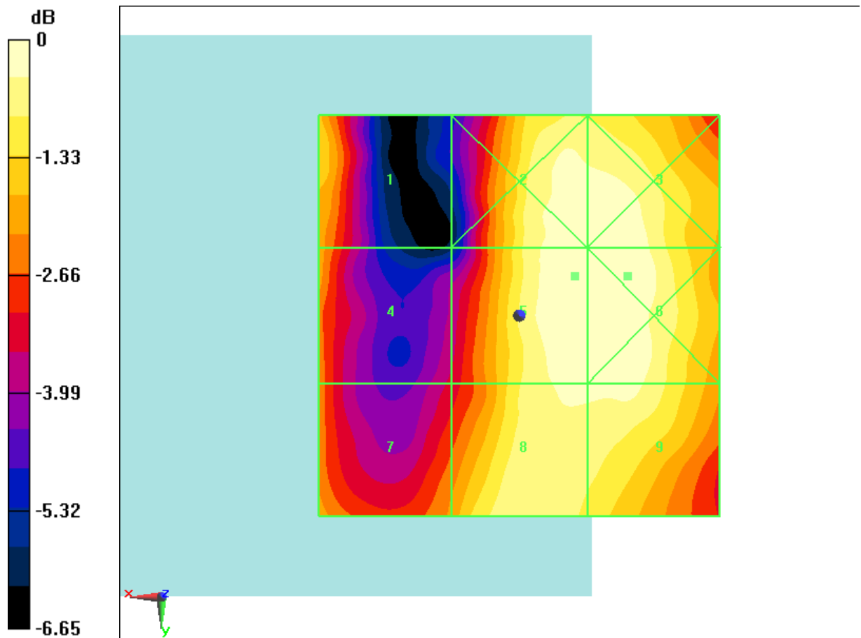
Fig B.16 HAC RF E-Field LTE Band41 16QAM CH39750
