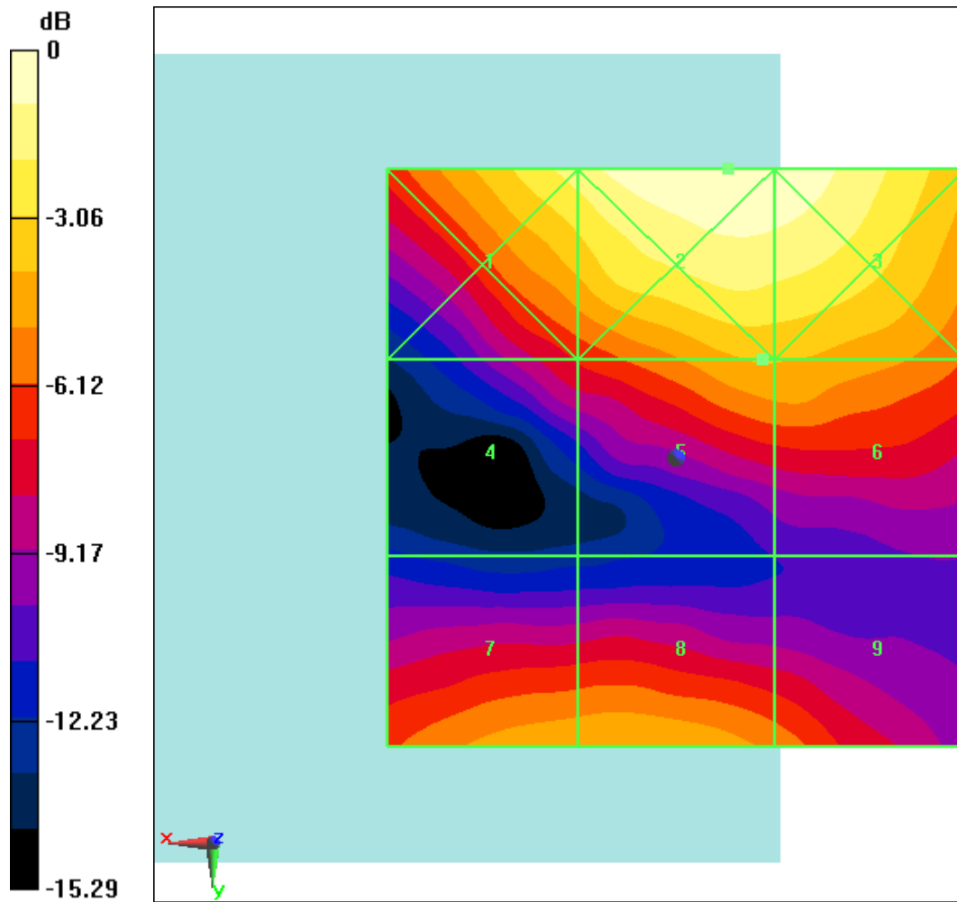
Fig B.6 HAC RF E-Field GSM 1900 Low
