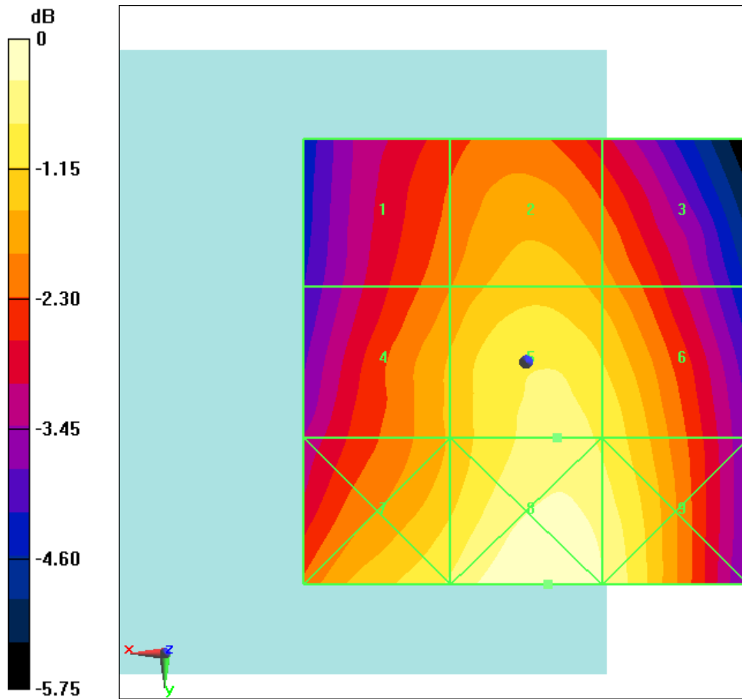
Fig B.3 HAC RF E-Field GSM 850 Low
