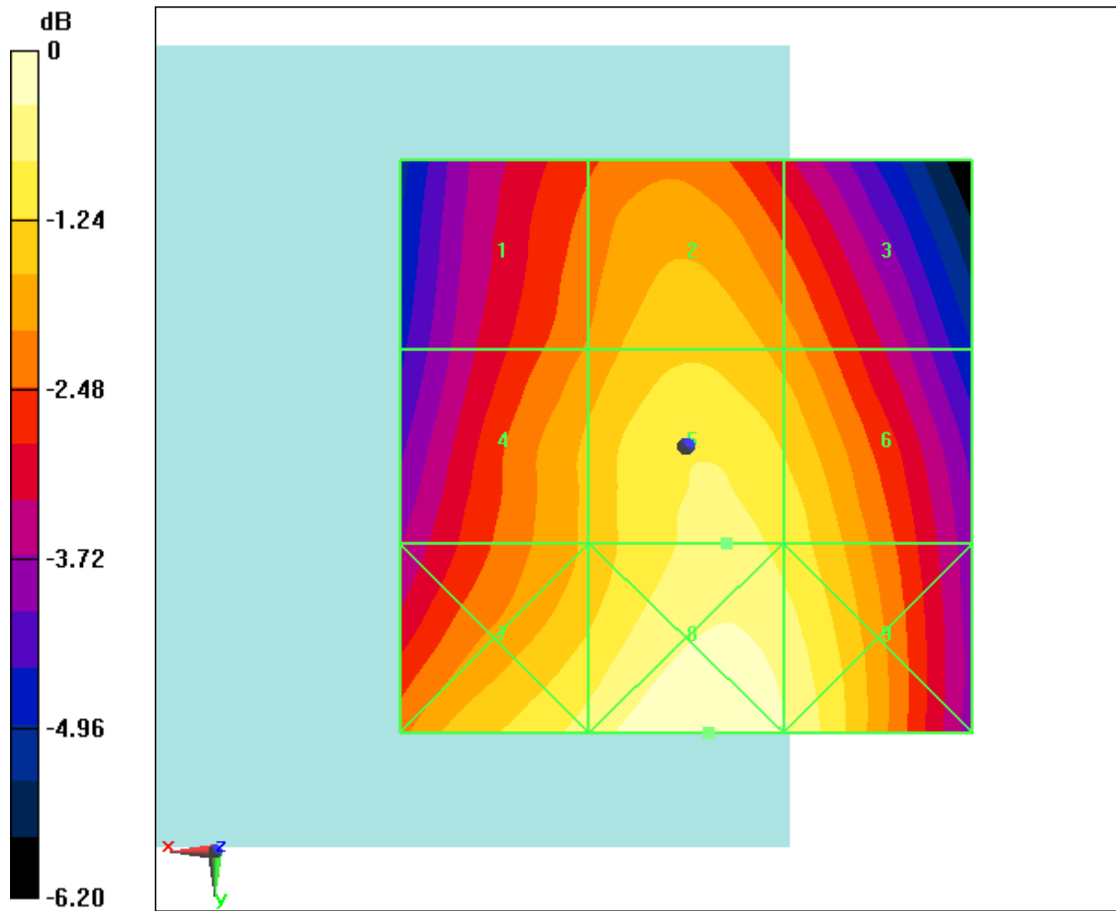
Fig B.1 HAC RF E-Field GSM 850 High
