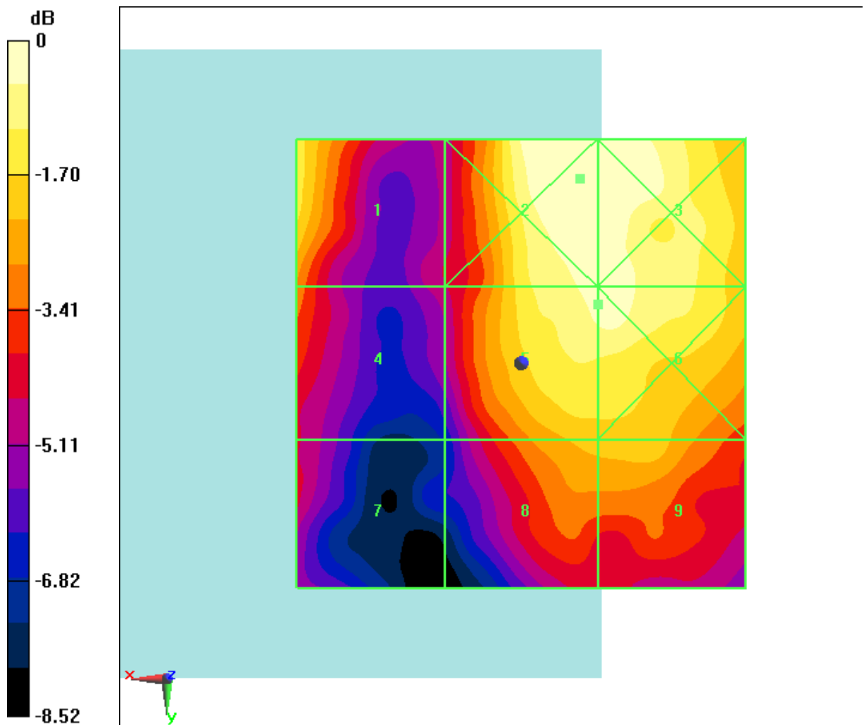
Fig B.19 HAC RF E-Field LTE Band41 64QAM CH40620
