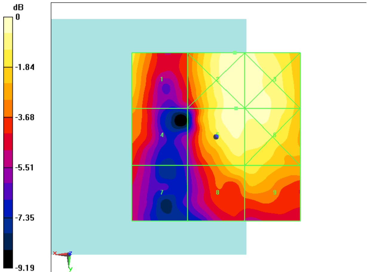
Fig B.14 HAC RF E-Field LTE Band41 16QAM CH40620
