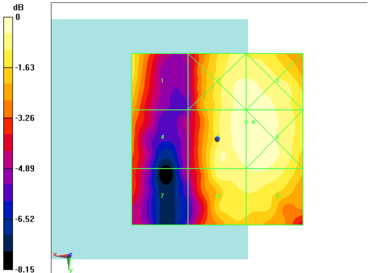
Fig B.15 HAC RF E-Field LTE Band41 16QAM CH40185
