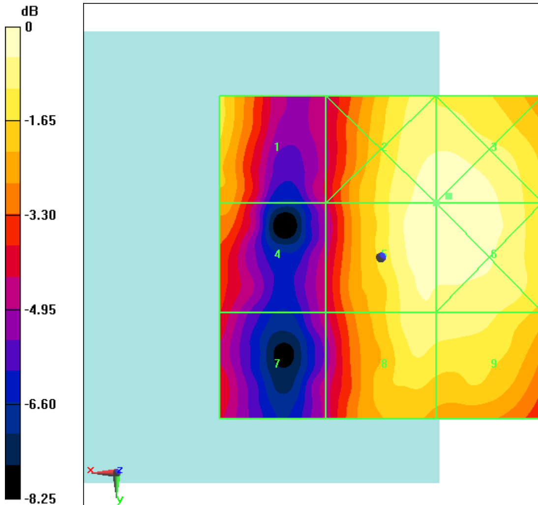
Fig B.20 HAC RF E-Field LTE Band41 64QAM CH40185
