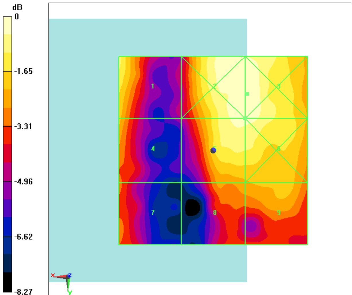
Fig B.18 HAC RF E-Field LTE Band41 64QAM CH41055
