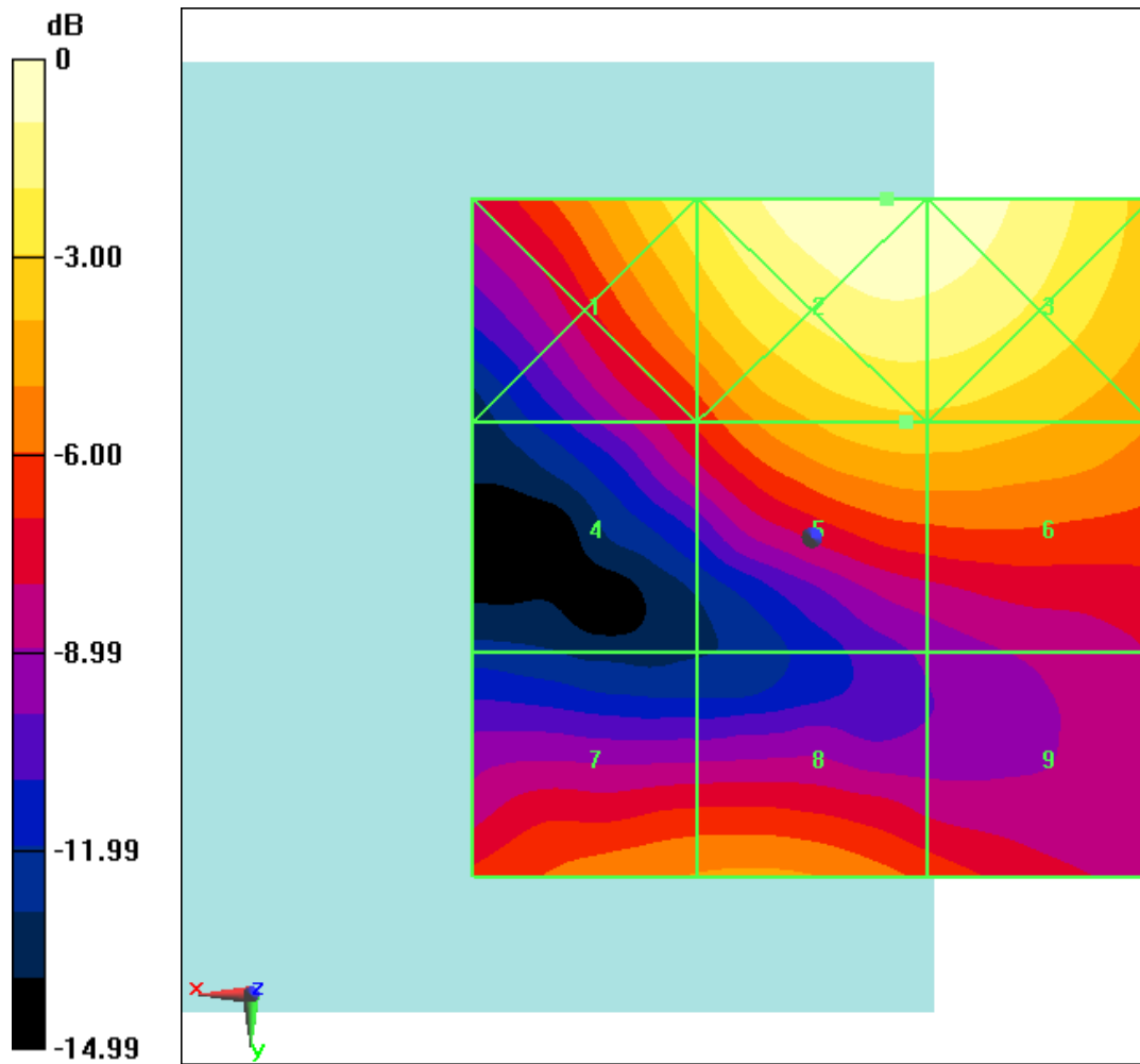
Fig B.4 HAC RF E-Field GSM 1900 High
