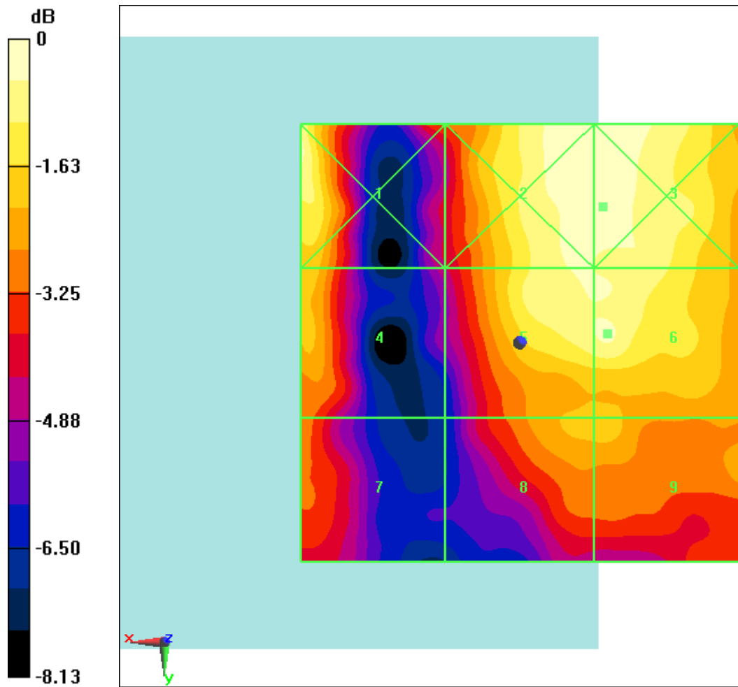
Fig B.13 HAC RF E-Field LTE Band41 16QAM CH41055
