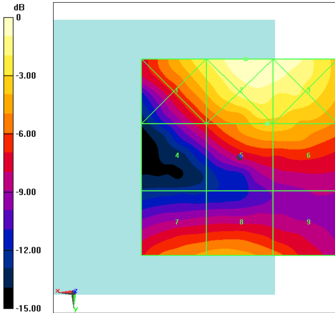
Fig B.5 HAC RF E-Field GSM 1900 Middle
