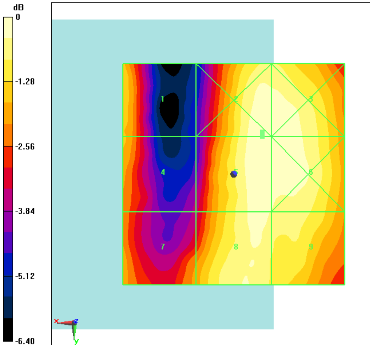
Fig B.11 HAC RF E-Field LTE Band41 QPSK CH39750
