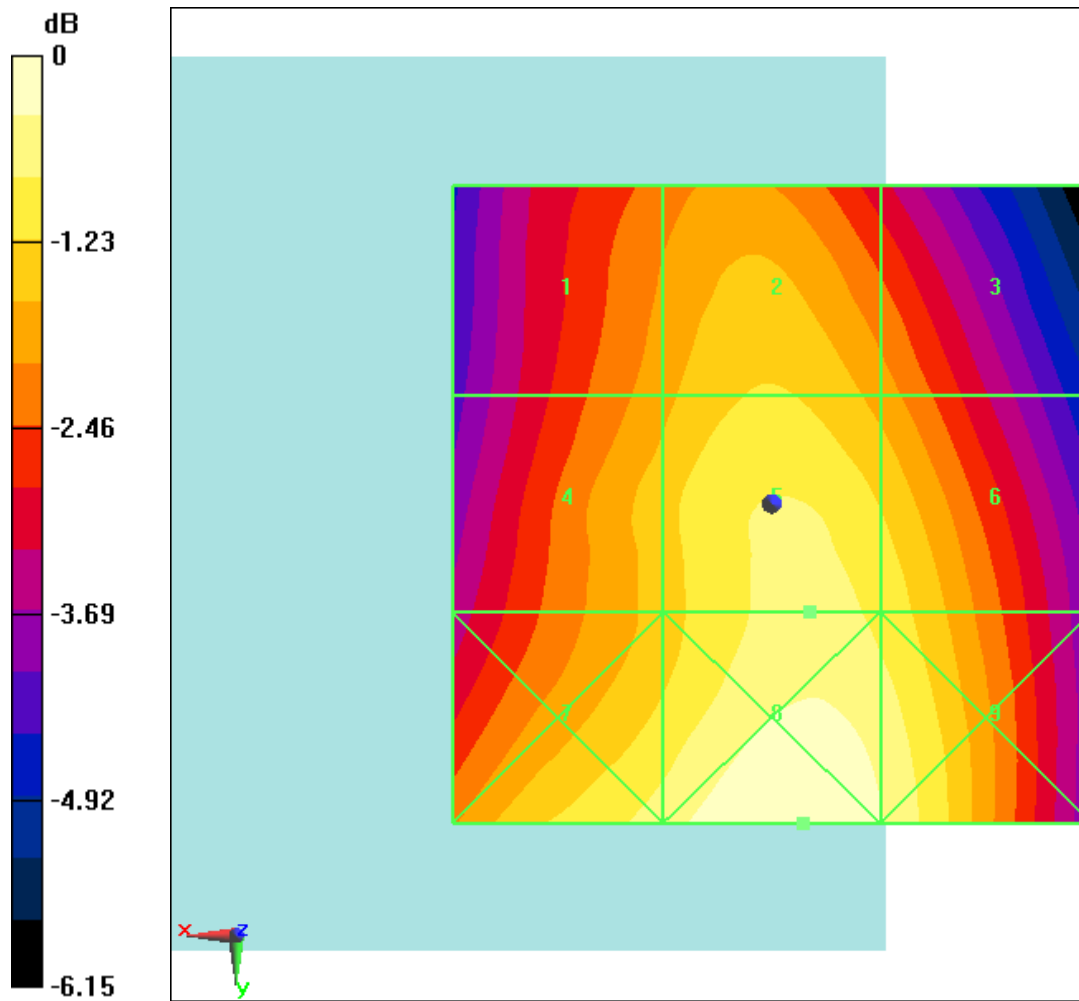
Fig B.2 HAC RF E-Field GSM 850 Middle
