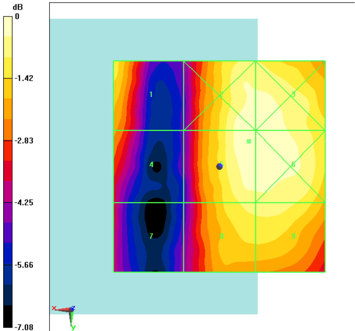
Fig B.10 HAC RF E-Field LTE Band41 QPSK CH40185
