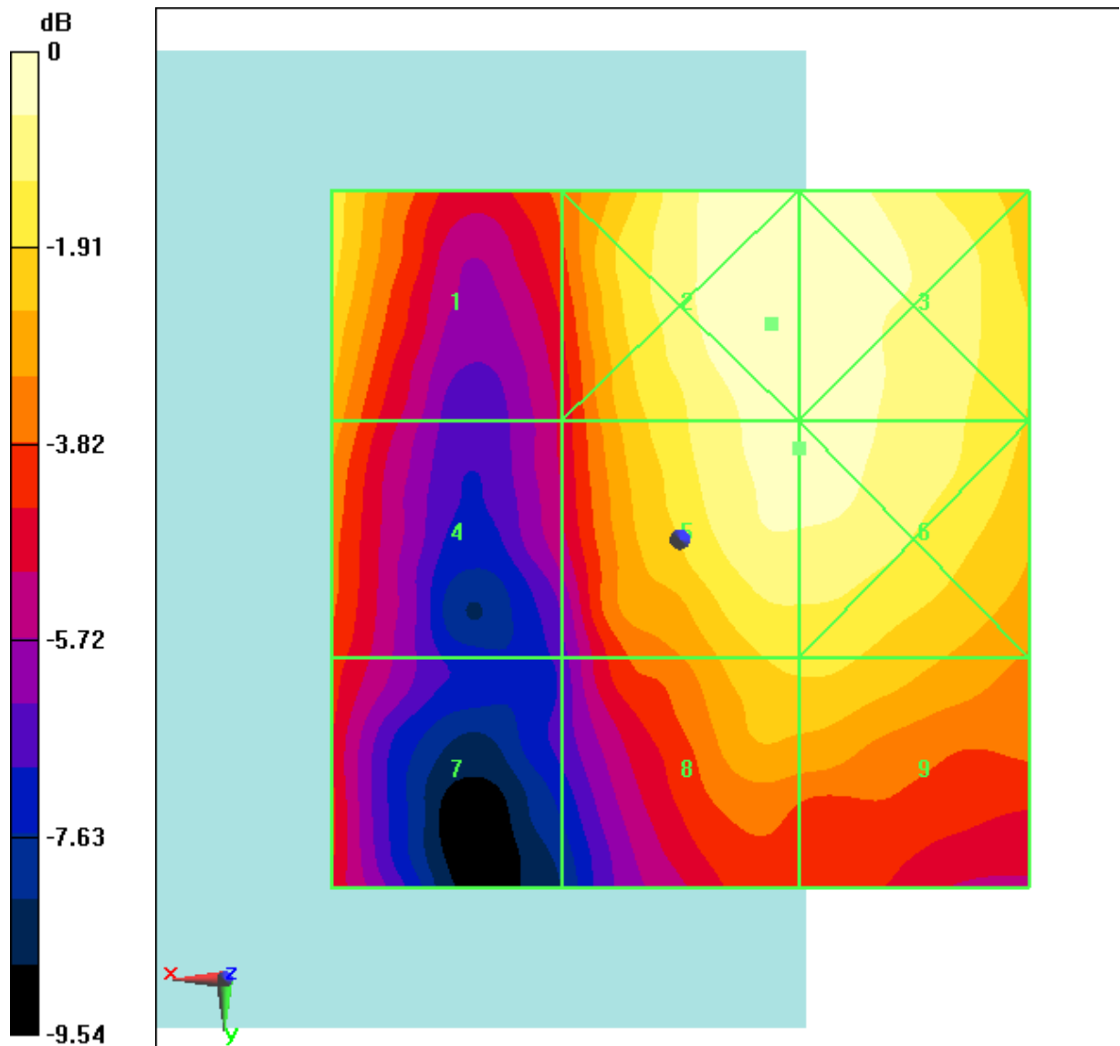
Fig B.9 HAC RF E-Field LTE Band41 QPSK CH40620
