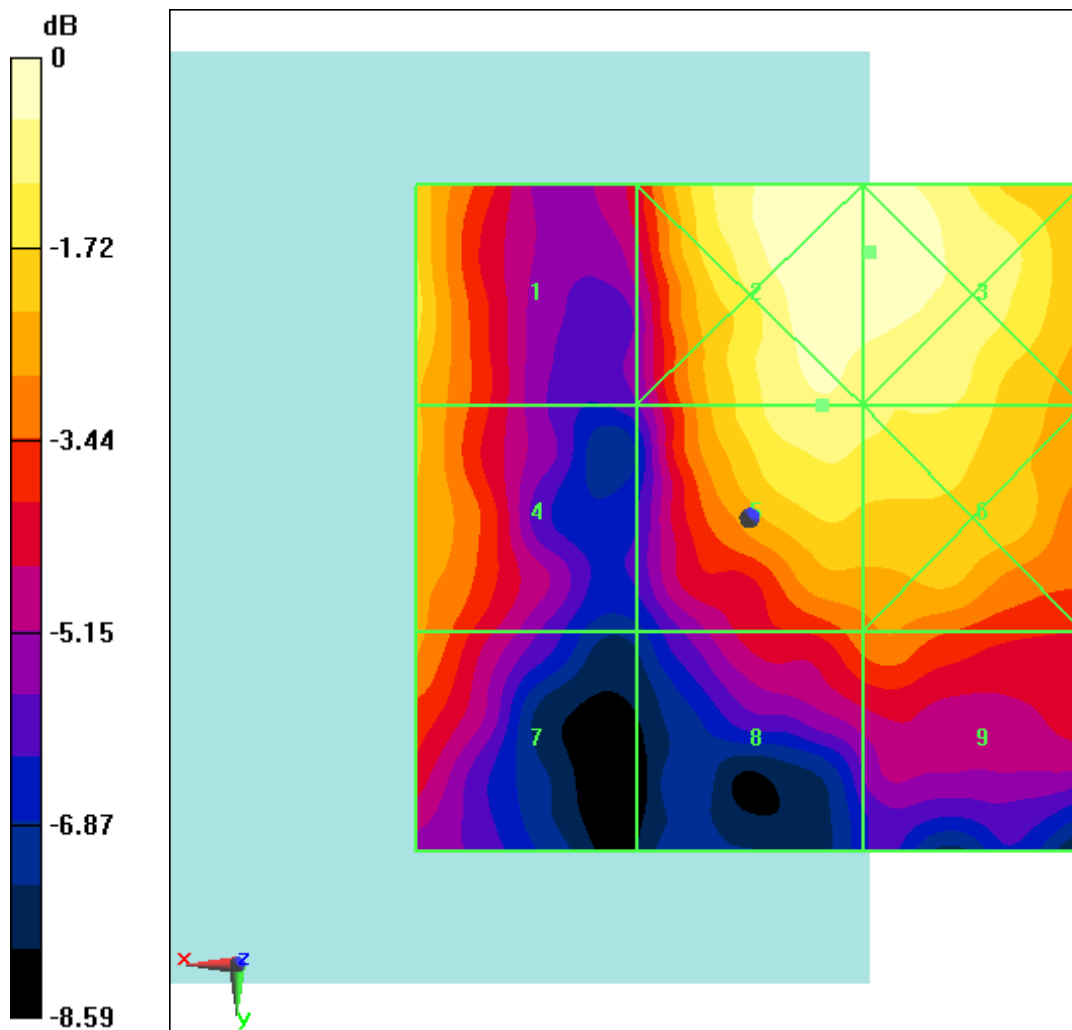
Fig B.17 HAC RF E-Field LTE Band41 64QAM CH41490
