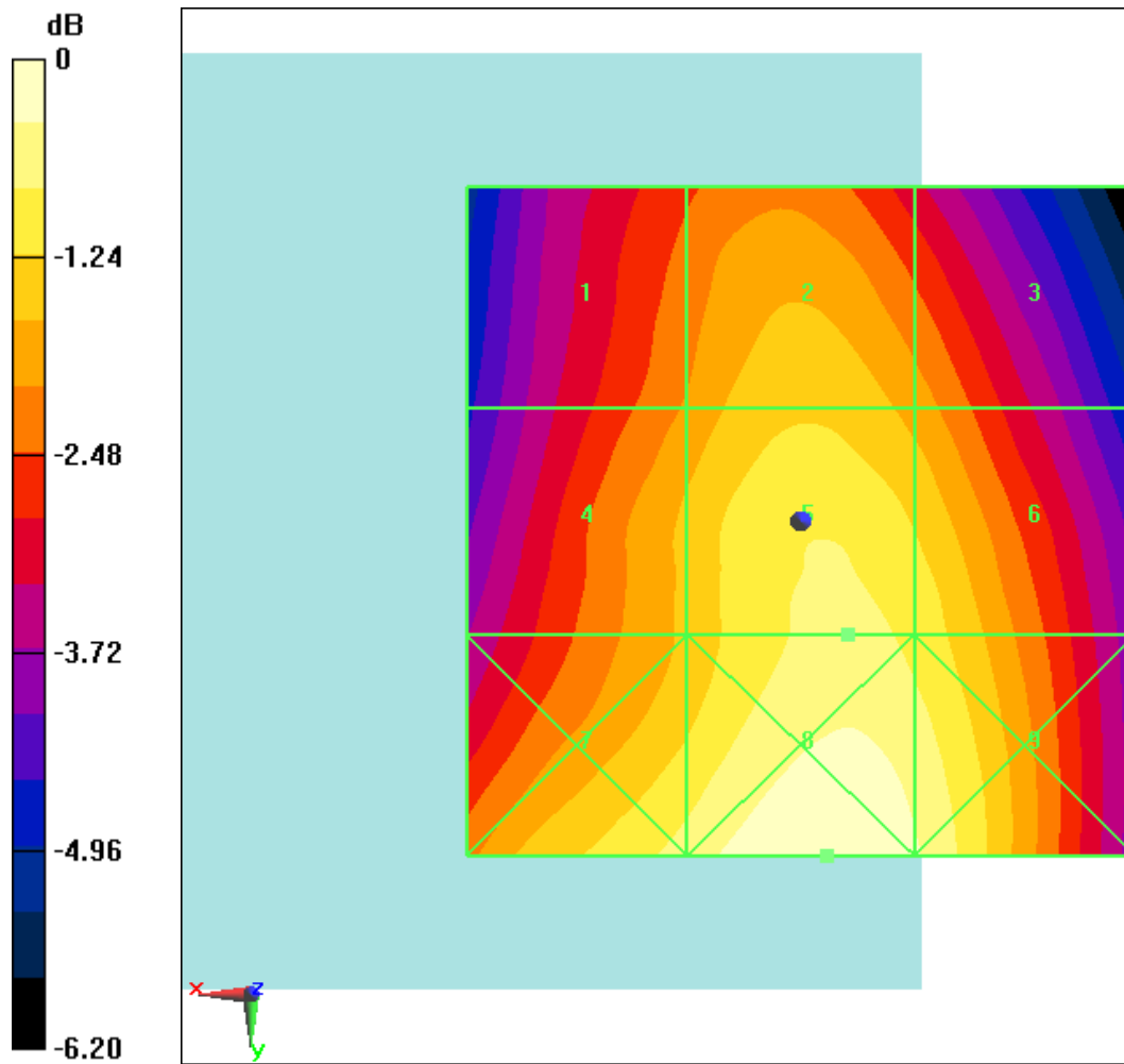
Fig B.1 HAC RF E-Field GSM 850 High
