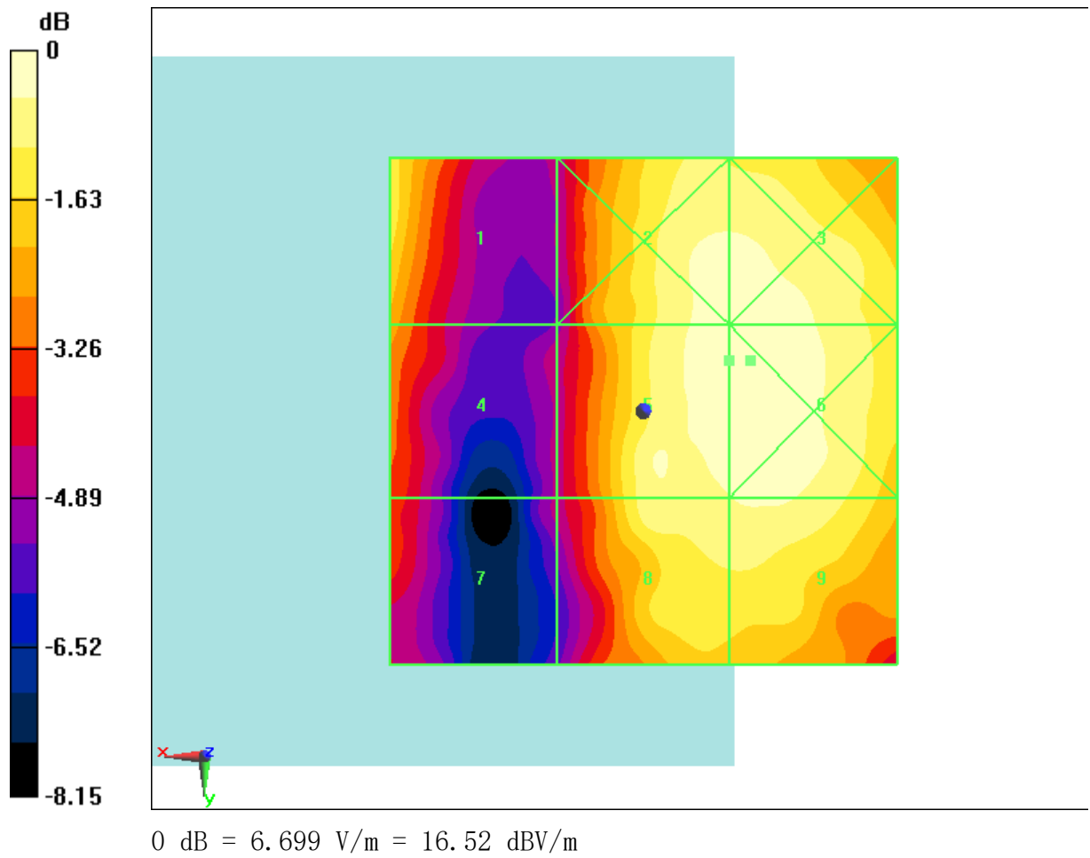
Fig B.15 HAC RF E-Field LTE Band41 16QAM CH40185
