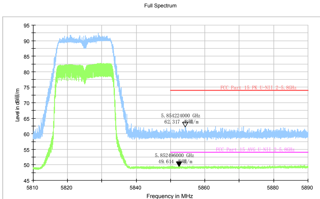
Fig. 84 Band Edges (802.11a, 5825MHz)
