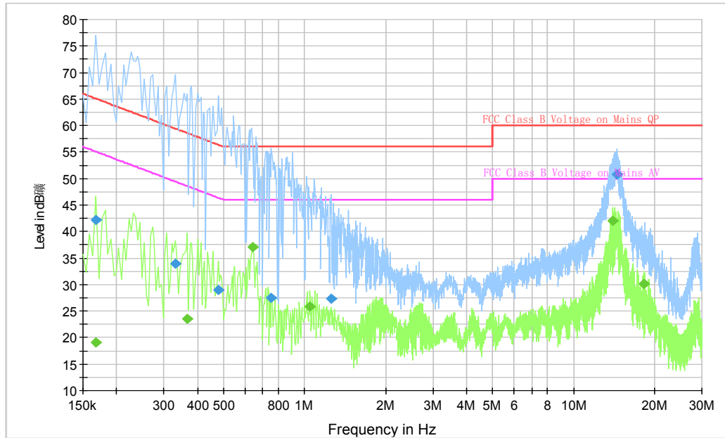
Fig. 96 AC Powerline Conducted Emission-802.11a
