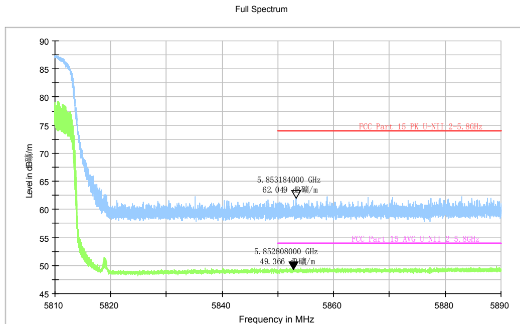
Fig. 88 Band Edges (802.11n-HT40, 5795MHz)
