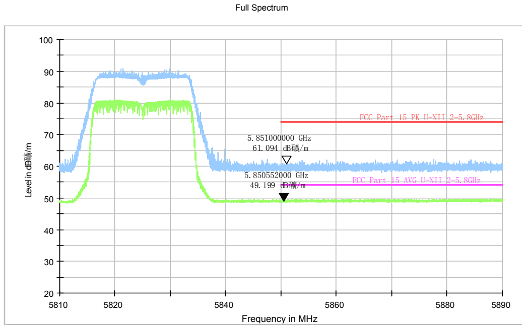
Fig. 86 Band Edges (802.11n-HT20, 5825MHz)
