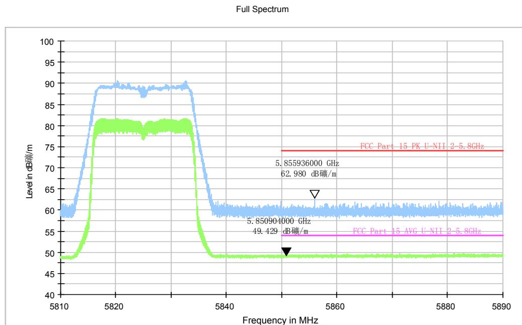
Fig. 90 Band Edges (802.11ac-HT20, 5825MHz)
