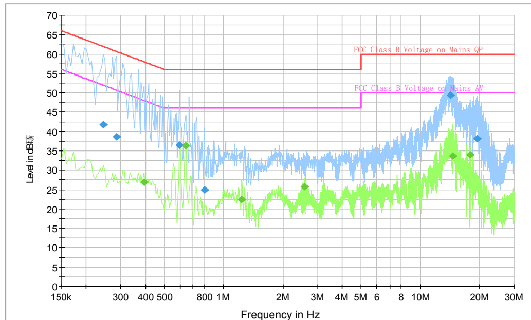
Fig. 93 AC Powerline Conducted Emission-802.11a
