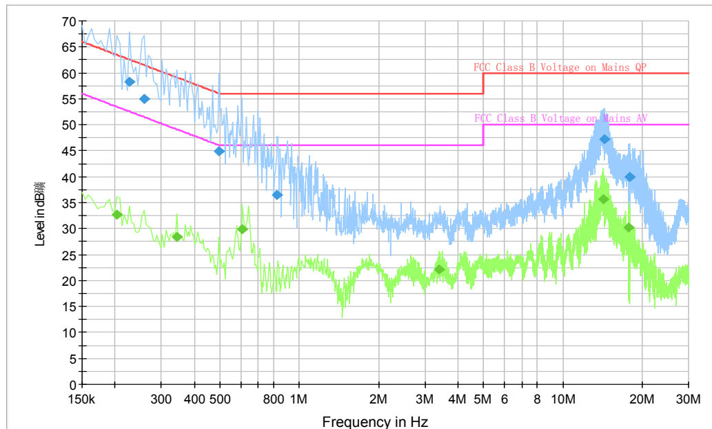
Fig. 94 AC Powerline Conducted Emission-Idle
