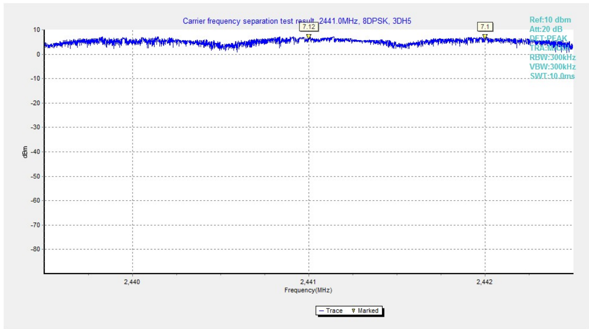
Fig.118. Carrier frequency separation measurement: 8DPSK, Channel 39
