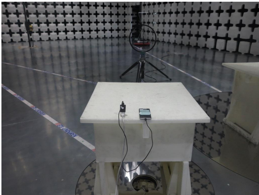
Picture C-2: Field Strength Measurements (Below 30MHz)
