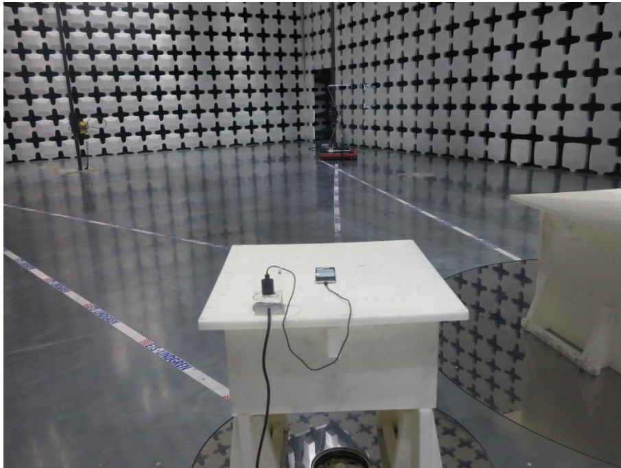
Picture C-3: Field Strength Measurements (Above 30MHz)
