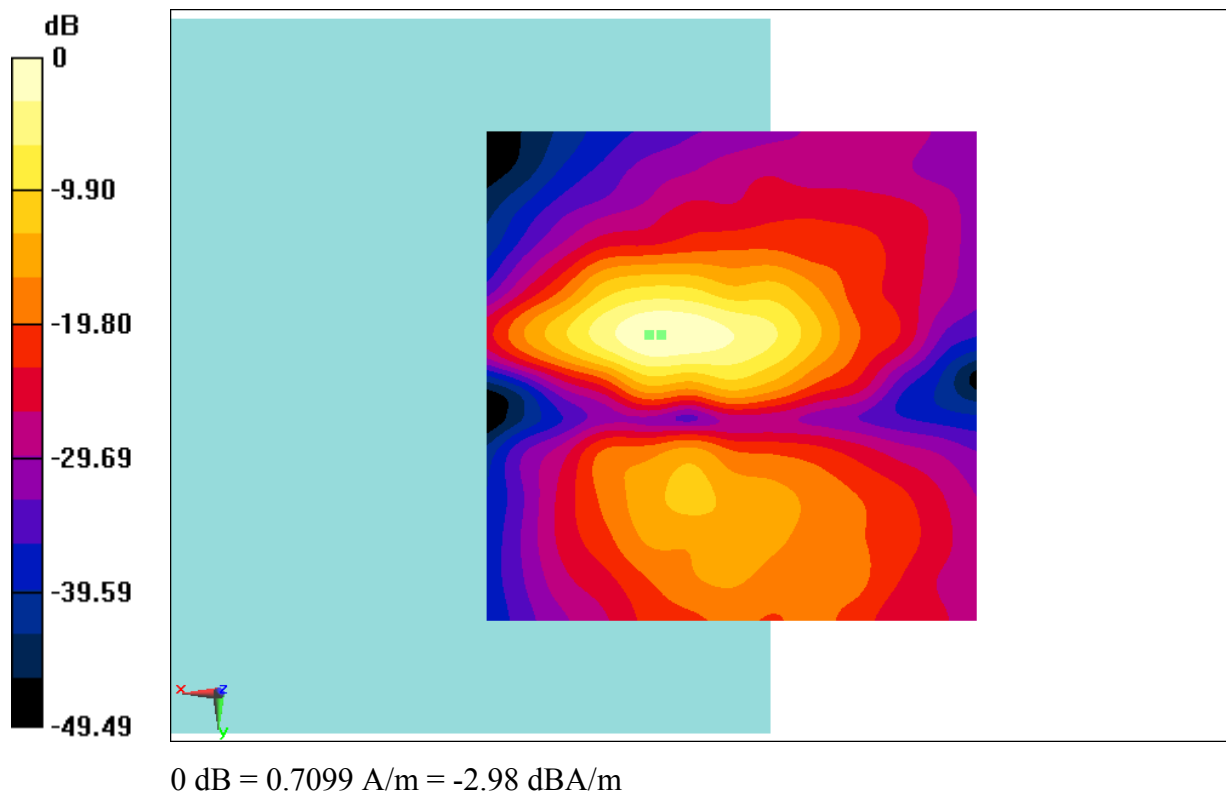
Fig B.15 T-Coil CDMA BC10_Channel 580
