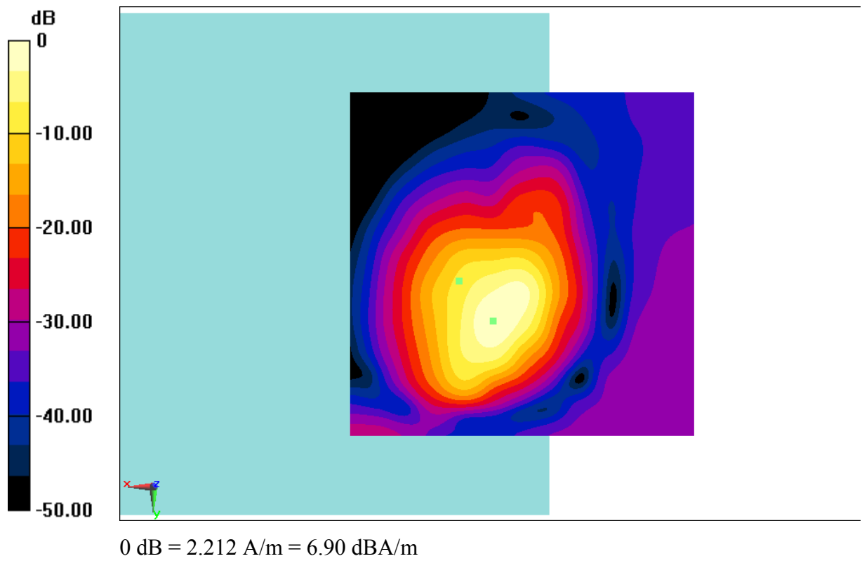
Fig B.12 T-Coil CDMA BC0_Channel 384
