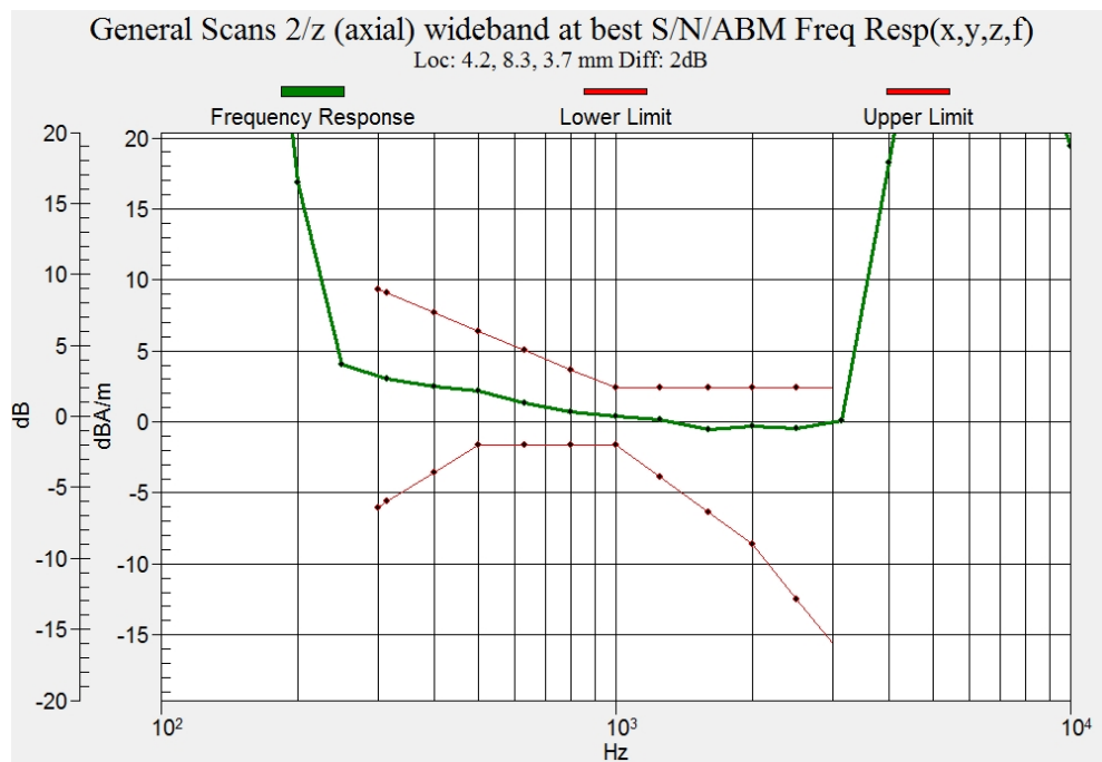
Figure C.6 Frequency Response of CDMA BC0_Channel 384
