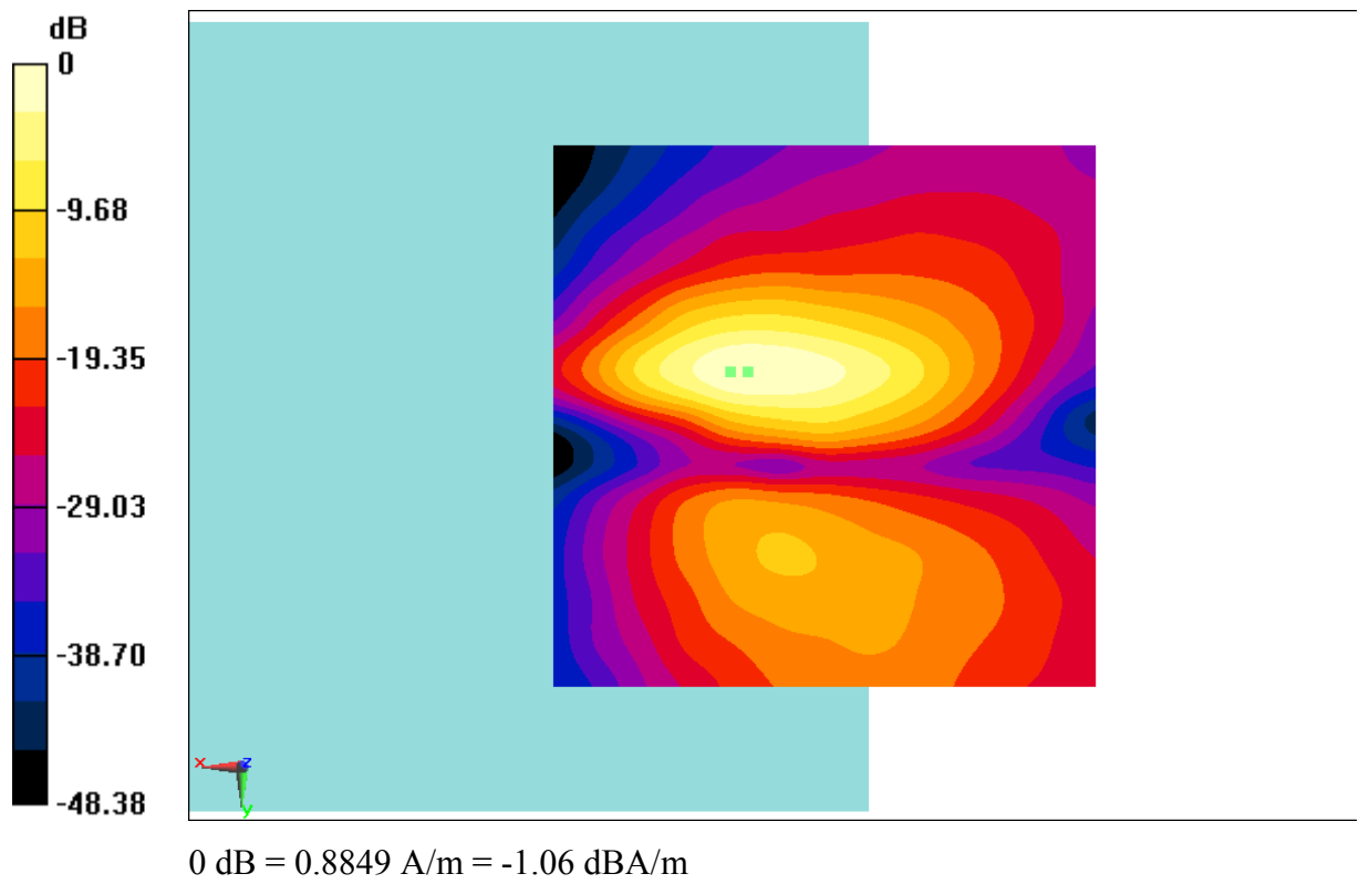
Fig B.11 T-Coil CDMA BC0_Channel 384
