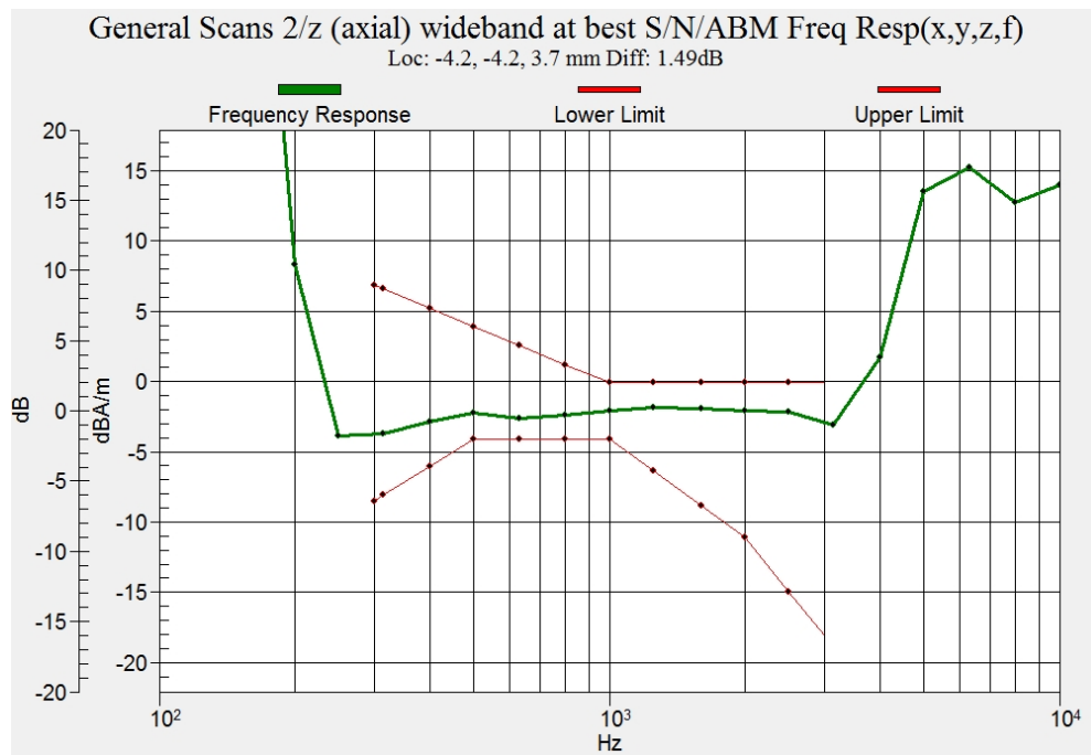
Figure C.7 Frequency Response of CDMA BC1_Channel 600
