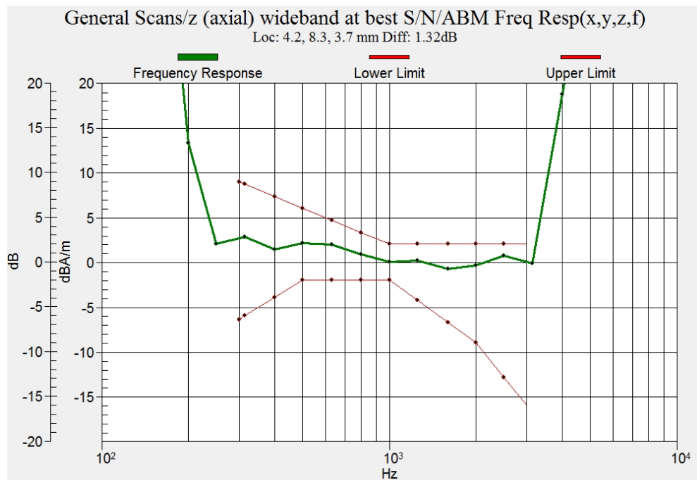
Figure C.8 Frequency Response of CDMA BC10_Channel 580
