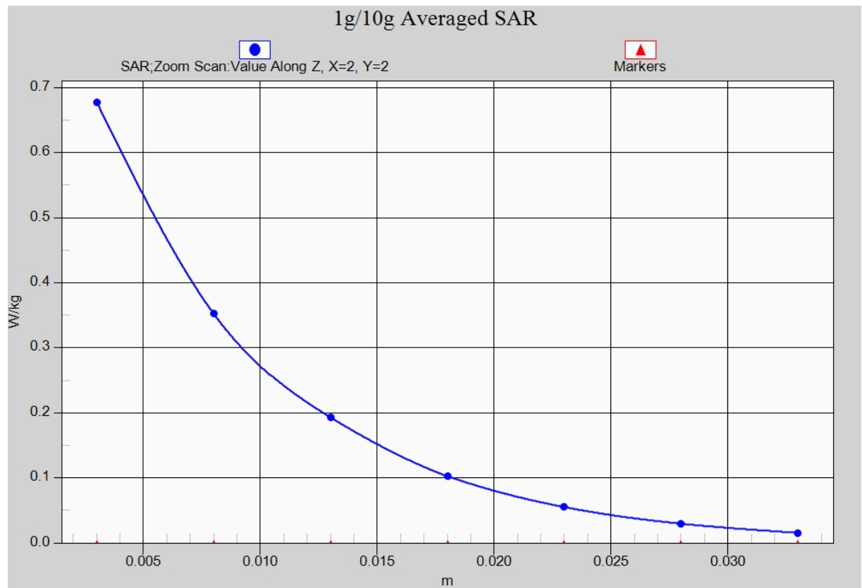
Fig. 54-1 Z-Scan at power reference point (2450 MHz)
