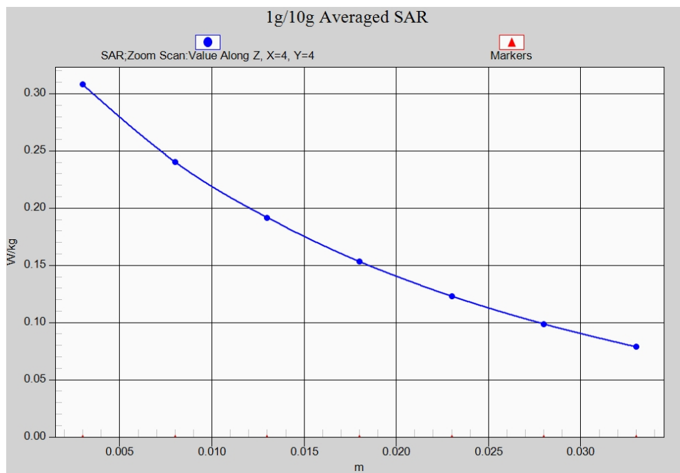
Fig. 45-1 Z-Scan at power reference point (CDMA BC0)
