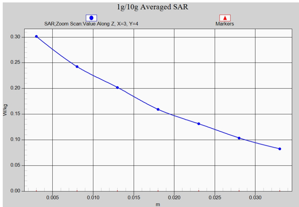
Fig. 40-1 Z-Scan at power reference point (LTE Band 26)
