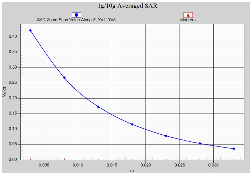
Fig. 47-1 Z-Scan at power reference point (CDMA BC1)
