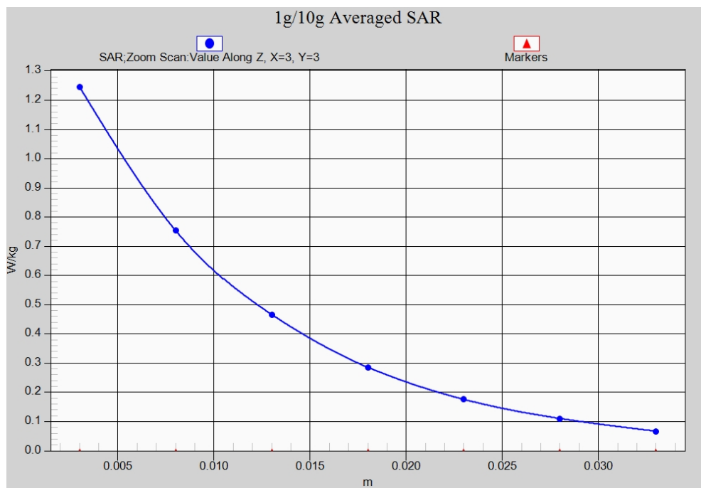
Fig. 48-1 Z-Scan at power reference point (CDMA BC1)
