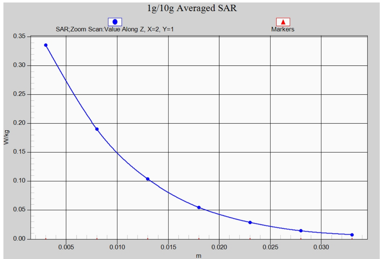
Fig. 53-1 Z-Scan at power reference point (2450 MHz)
