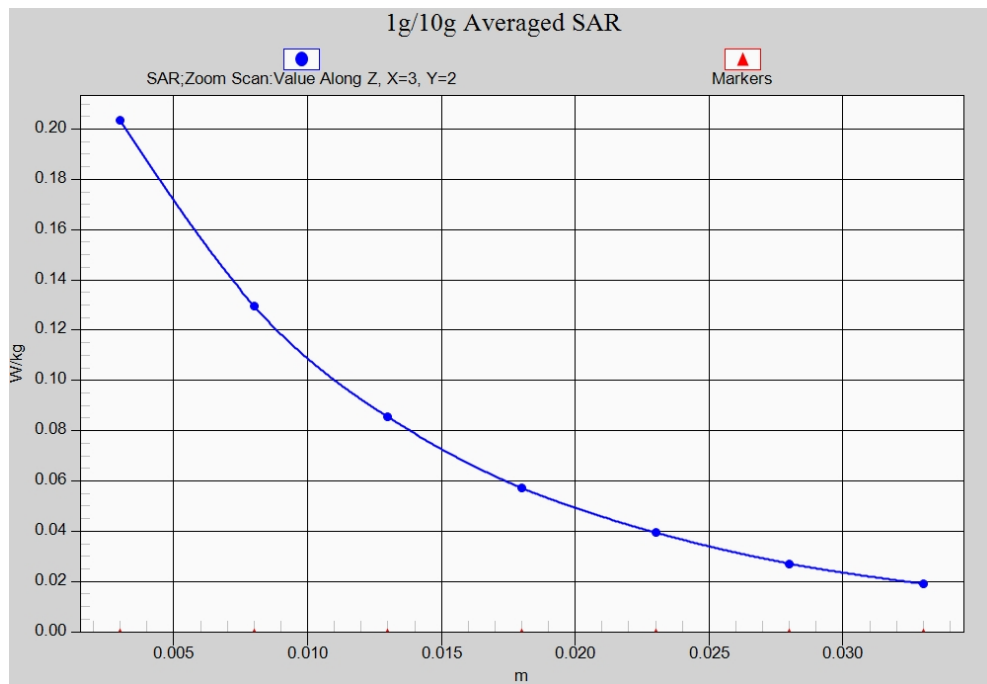
Fig. 52-1 Z-Scan at power reference point (CDMA BC10)
