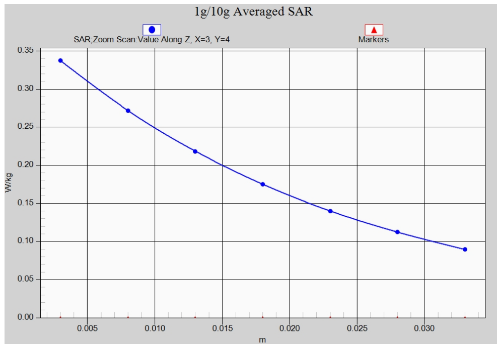
Fig. 49-1 Z-Scan at power reference point (CDMA BC10)
