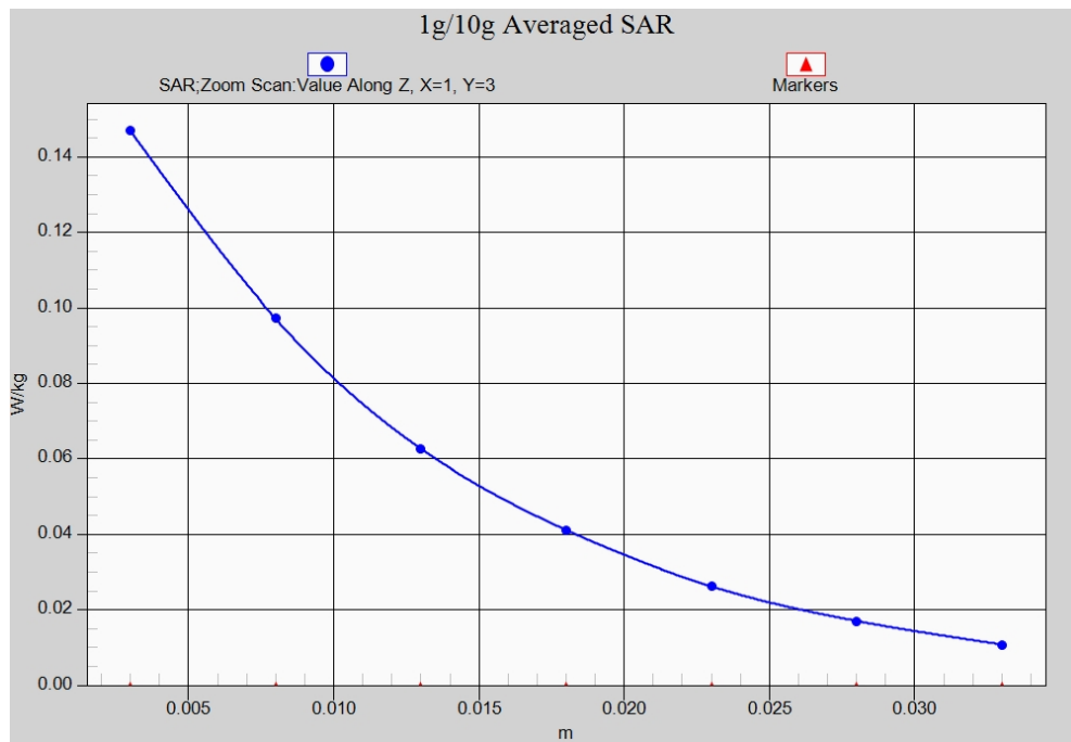
Fig. 37-1 Z-Scan at power reference point (LTE Band 25)
