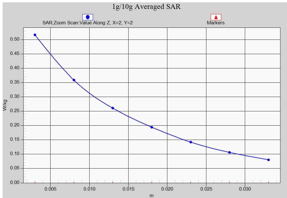
Fig. 42-1 Z-Scan at power reference point (LTE Band 26)
