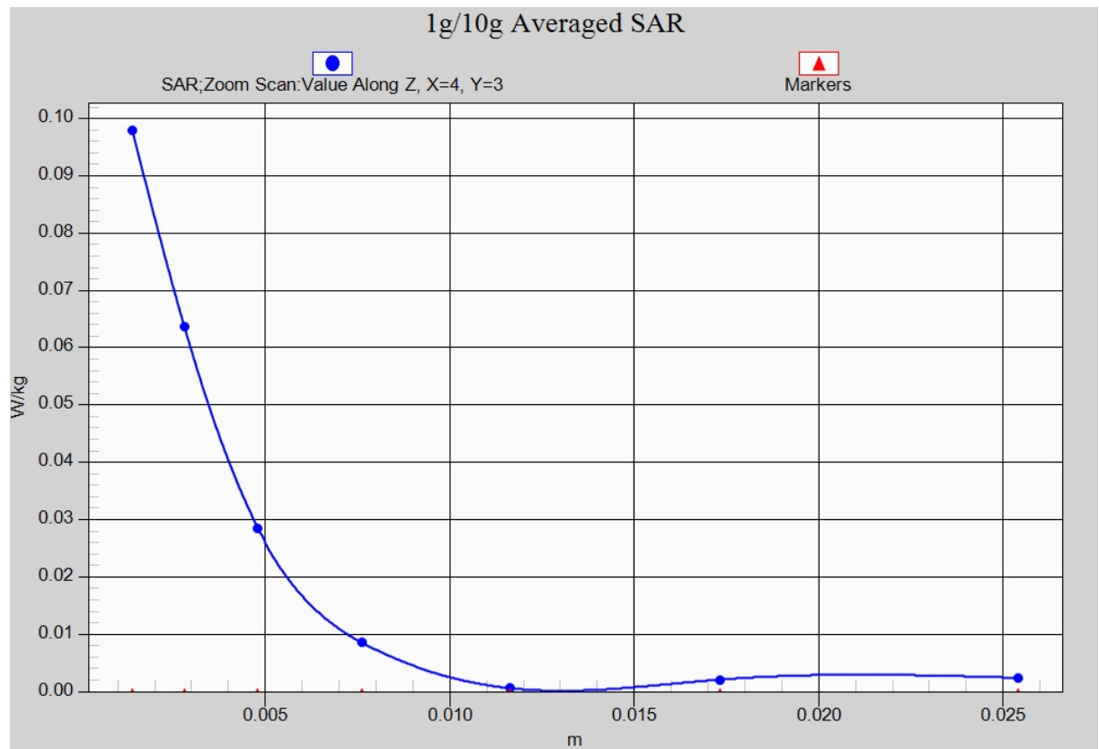
Fig. 55-1 Z-Scan at power reference point (5GHz)
