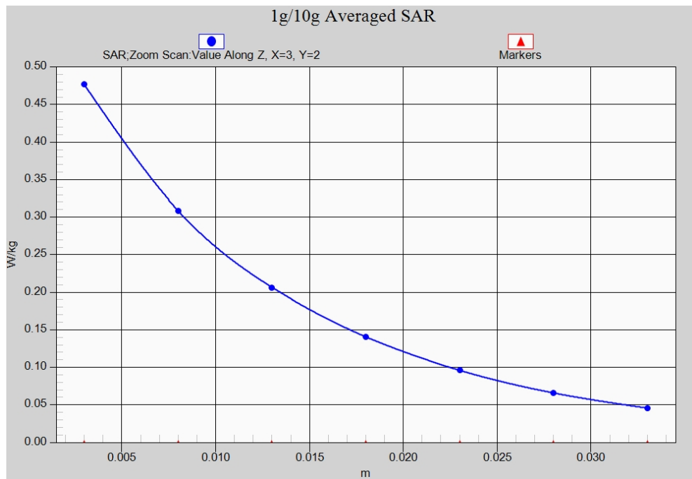
Fig. 46-1 Z-Scan at power reference point (CDMA BC0)
