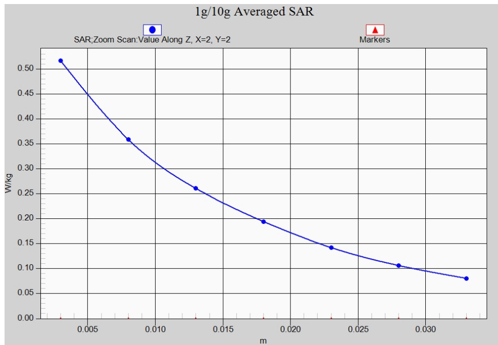
Fig. 43-1 Z-Scan at power reference point (LTE Band 26)
