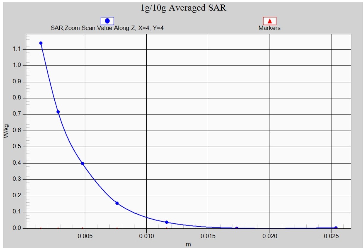
Fig. 56-1 Z-Scan at power reference point (5GHz)
