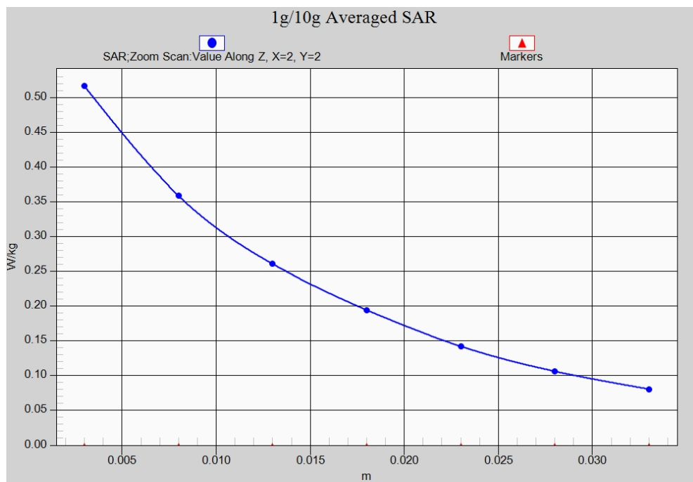
Fig. 41-1 Z-Scan at power reference point (LTE Band 26)
