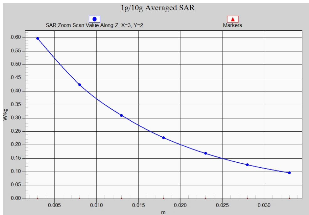
Fig. 50-1 Z-Scan at power reference point (CDMA BC10)
