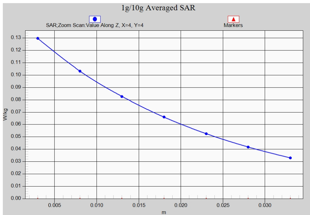
Fig. 51-1 Z-Scan at power reference point (CDMA BC10)
