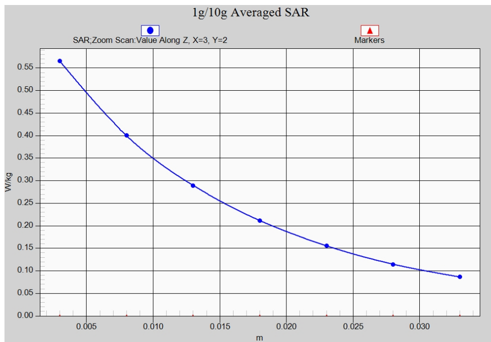
Fig. 44-1 Z-Scan at power reference point (CDMA BC0)
