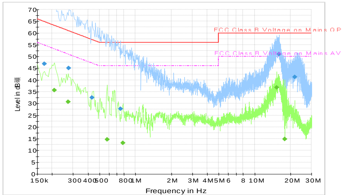
Fig.A.7.4 AC Powerline Conducted Emission-802.11b
