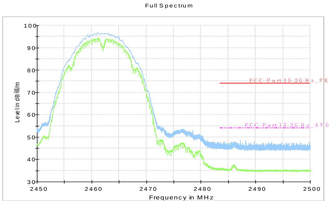
Fig.A.6.2.3 Transmitter Spurious Emission - Radiated (Power): 802.11b, ch11, 2.45 GHz - 2.50GHz
