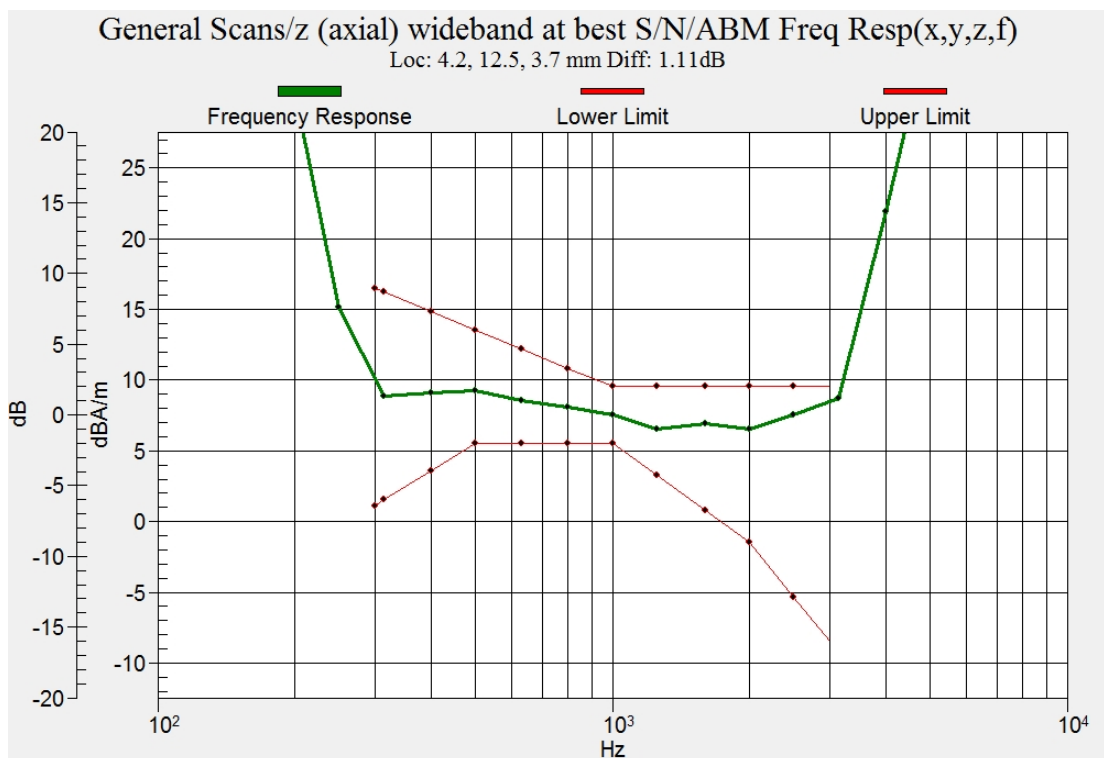
Figure C.8 Frequency Response of CDMA BC10_Channel 580
