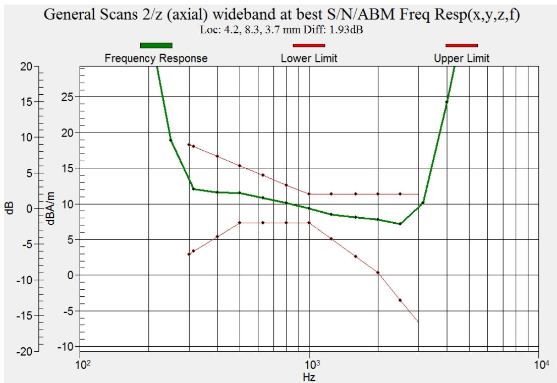
Figure C.7 Frequency Response of CDMA BC1_Channel 600
