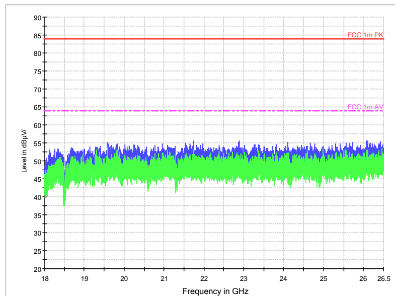
Fig.28. Transmitter Spurious Emission - Radiated: GFSK, 18 GHz - 26 GHz
