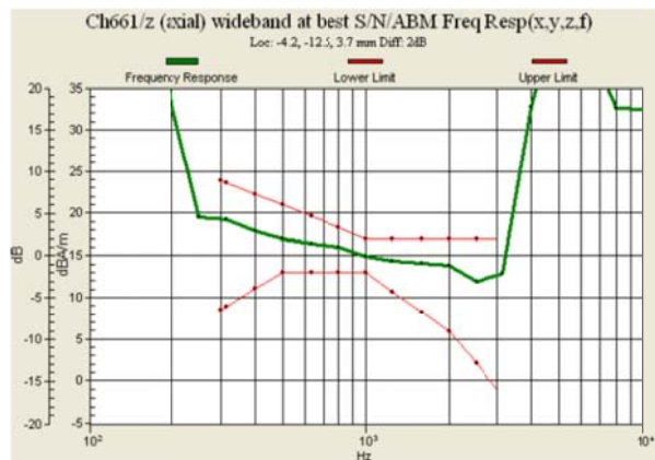
Fig 7.2 GSM1900 Ch661
