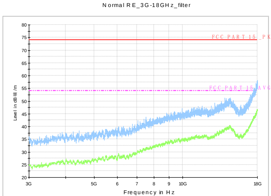
Fig.A.6.2.14 Transmitter Spurious Emission - Radiated (802.11g, Ch1, 3 GHz-18 GHz)
