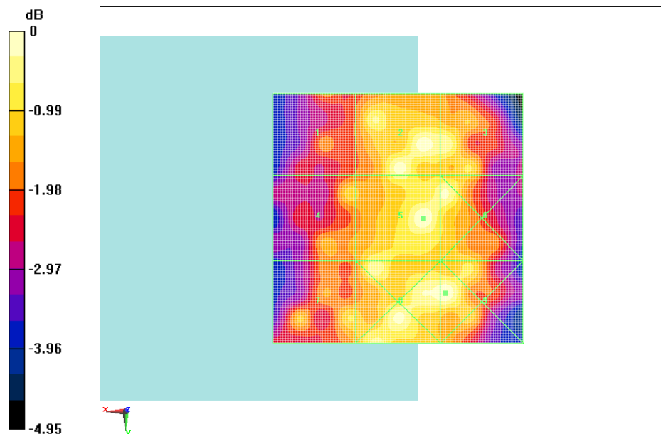
Fig B.3 HAC RF E-Field CDMA 835 Low
