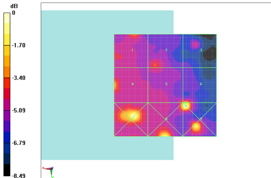
Fig B.6 HAC RF E-Field CDMA 1900 Low
