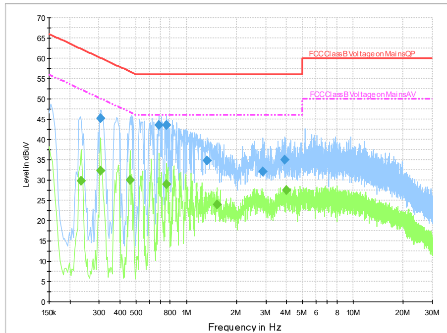
Fig.A.6.1. AC Powerline Conducted Emission
