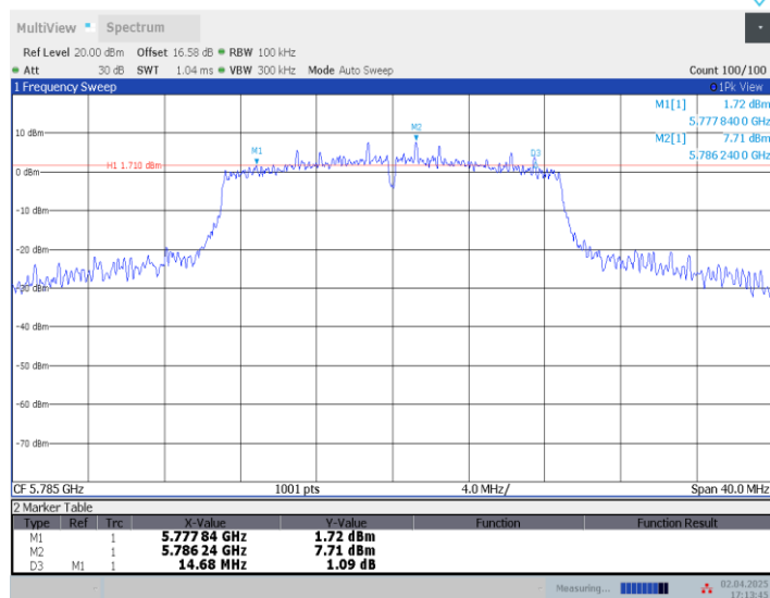
11N20SISO_Ant1_5785
