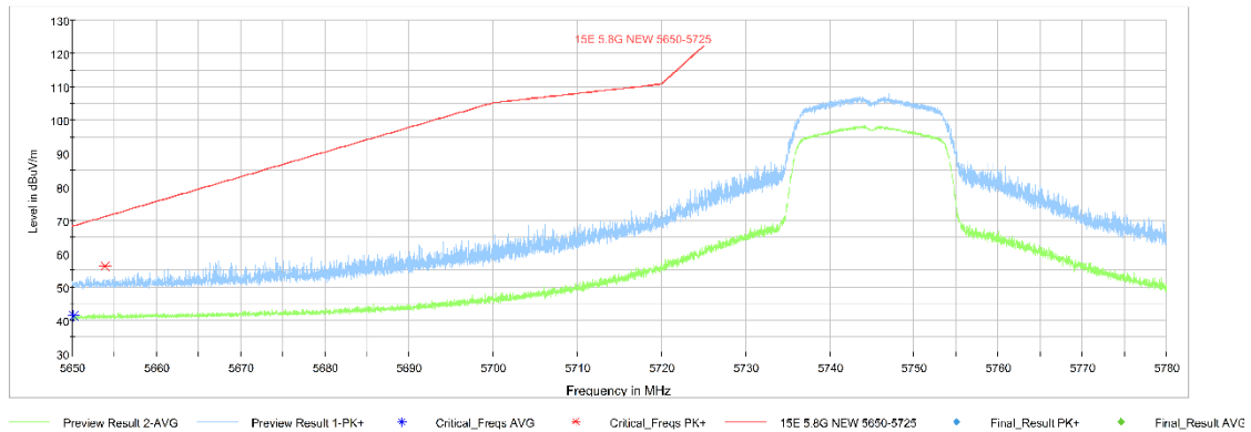
Fig. 7 Band Edges (802.11ac-HT20 Ch149, 5745MHz)
