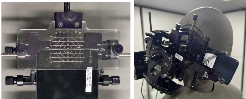
Pic 3: Handset Positioner (HHPIII) with mounted EUT mobile phone
