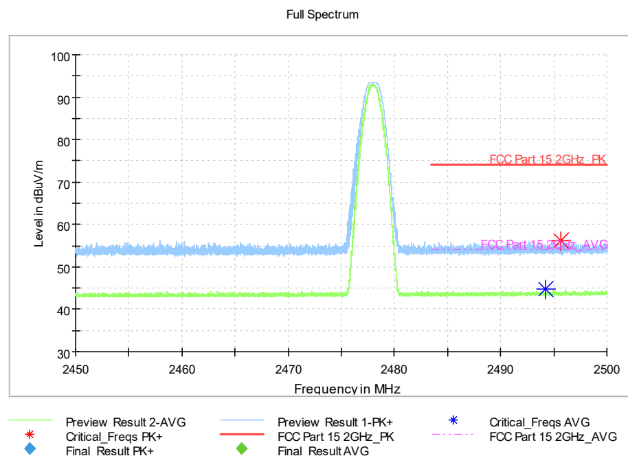
Fig.2. Frequency Band Edges: GFSK, 2480 MHz, Hopping Off, 2.45 GHz - 2.50GHz
