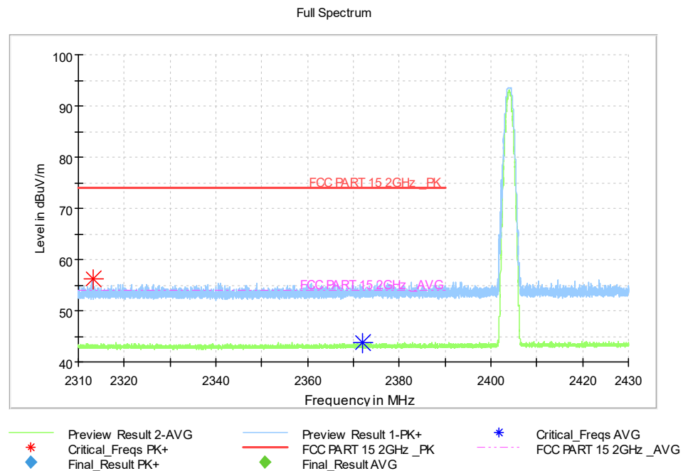
Fig.1. Frequency Band Edges: GFSK, 2402 MHz, Hopping Off, 2.31 GHz – 2.43GHz
