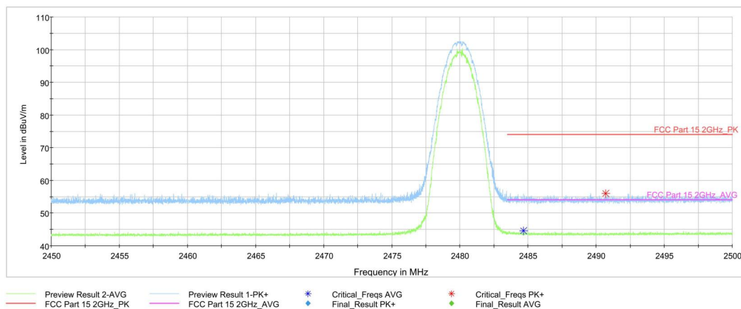
Fig.4. Frequency Band Edges: \pi/4 DQPSK, Channel 78, Hopping Off, 2.45 GHz - 2.50GHz
