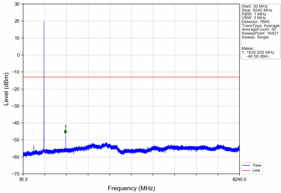
Band26a 3MHz 16QAM HCH 822.5MHz RB 1 0 NTNV
