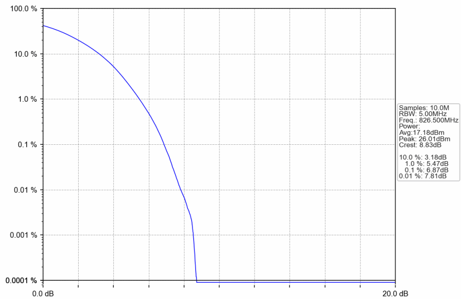
Band5 5MHz 256QAM LCH 826.5MHz RB 25 0 NTNV
