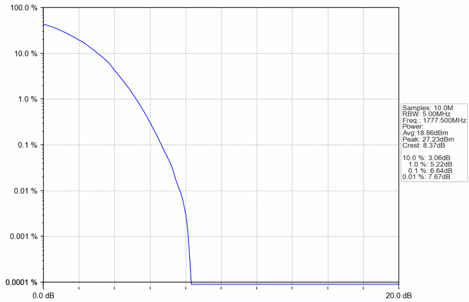
Band66 5MHz 64QAM HCH 1777.5MHz RB 25 0 NTNV
