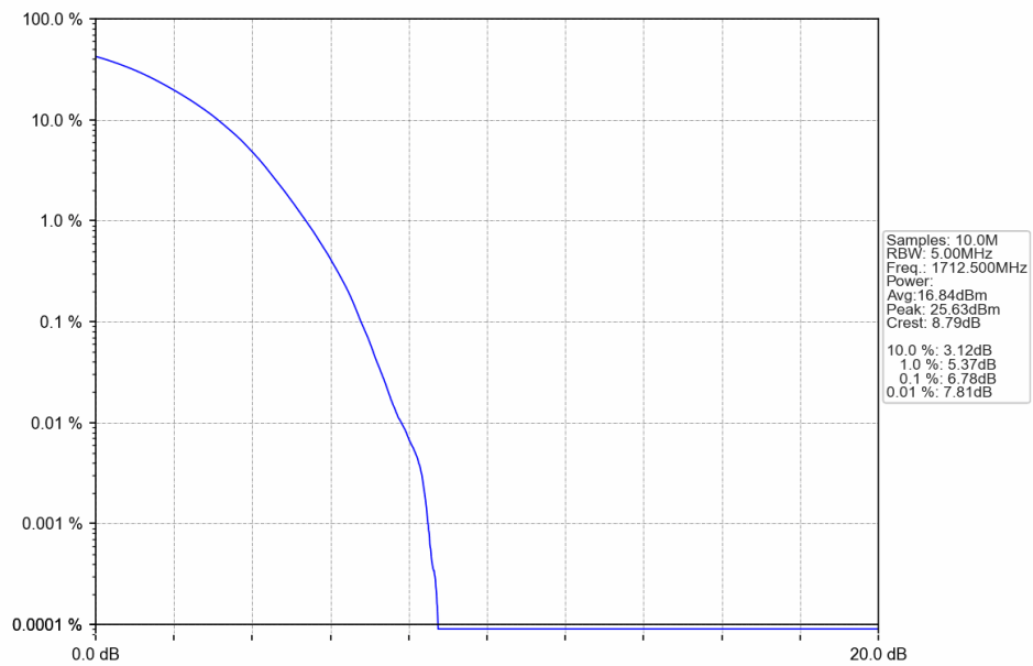
Band66 5MHz 256QAM LCH 1712.5MHz RB 25 0 NTNV
