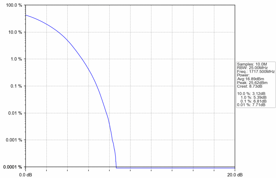
Band66 15MHz 256QAM LCH 1717.5MHz RB 75 0 NTNV
