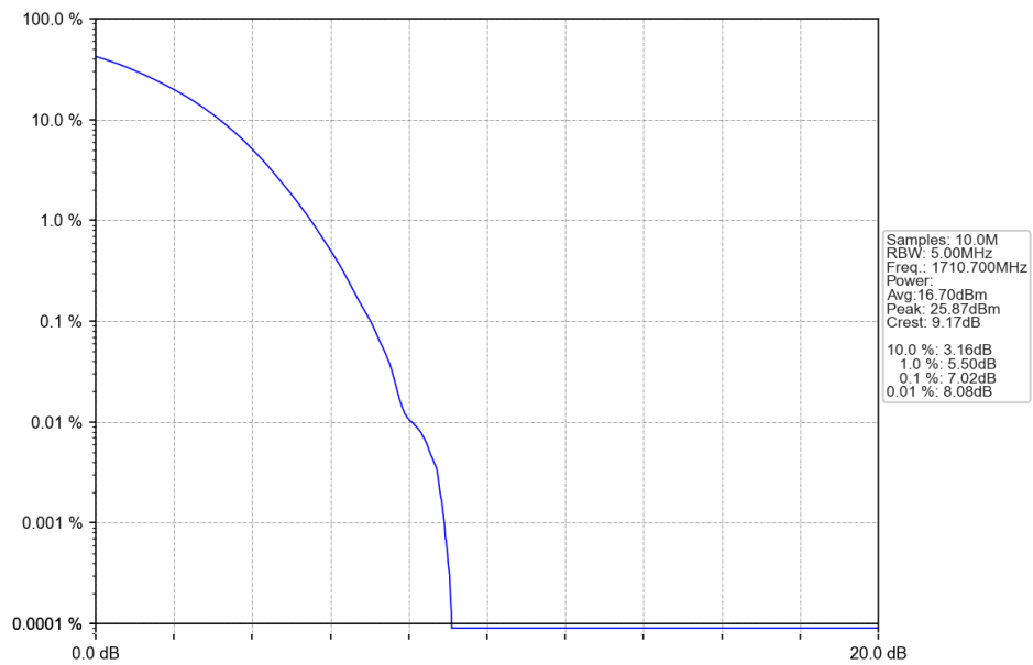
Band66 1.4MHz 256QAM LCH 1710.7MHz RB 6 0 NTNV
