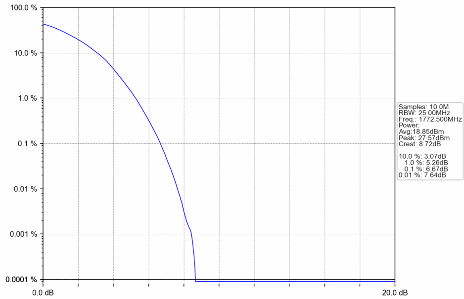
Band66 15MHz 64QAM HCH 1772.5MHz RB 75 0 NTNV
