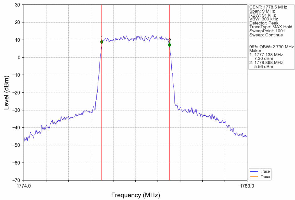
Band66 3MHz 256QAM HCH 1778.5MHz RB 15 0 NTN
