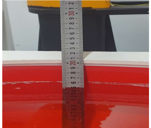
Photo 2: Tissue Simulant Liquid for HBBL600-10000MHz
