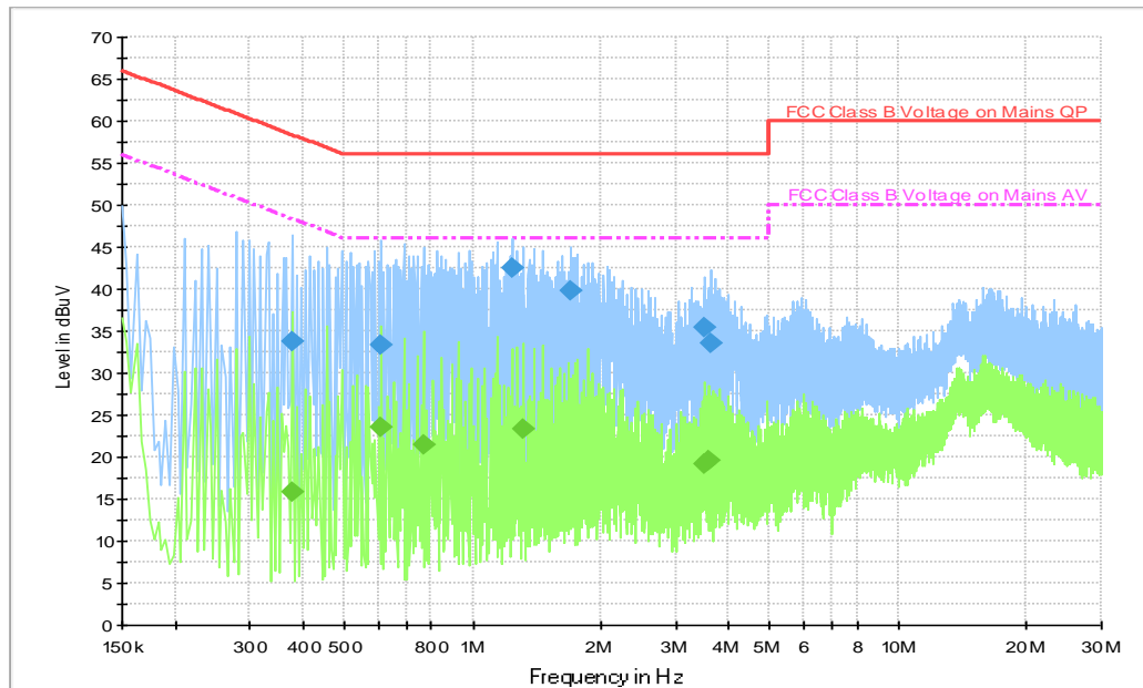
Fig.B.8.1 AC Powerline Conducted Emission- Bluetooth With charger QC16US
