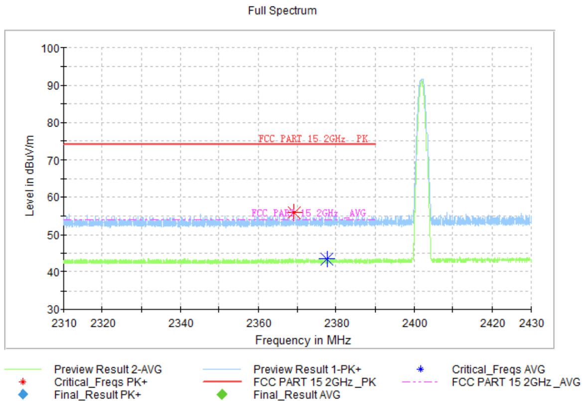
Fig.1. Frequency Band Edges: GFSK, 2402 MHz, Hopping Off, 2.31 GHz – 2.43GHz
