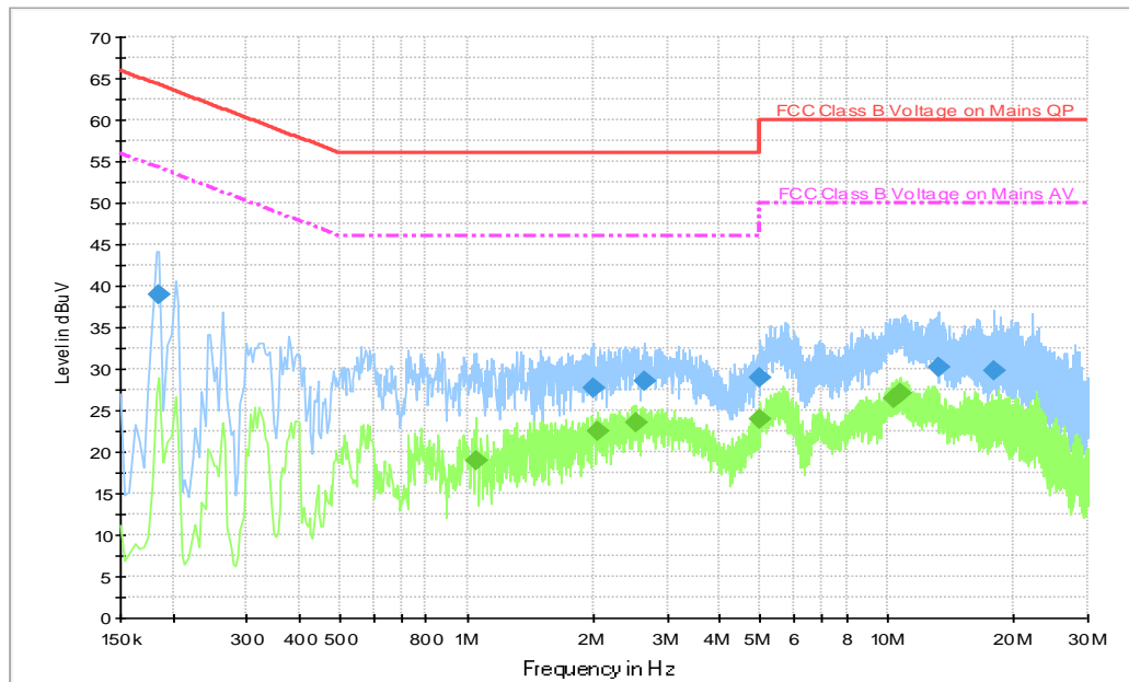
Fig.B.8.3 AC Powerline Conducted Emission- Bluetooth With charger QC16EU
