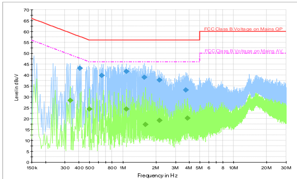
Fig.B.8.2 AC Powerline Conducted Emission-Iidle With charger QC16US
