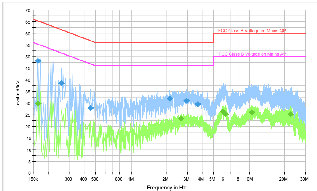
Fig.B.10.3 AC Powerline Conducted Emission- Bluetooth With charger QC16EU
