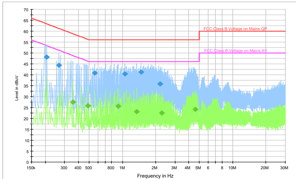
Fig.B.10.1 AC Powerline Conducted Emission- Bluetooth With charger QC16US
