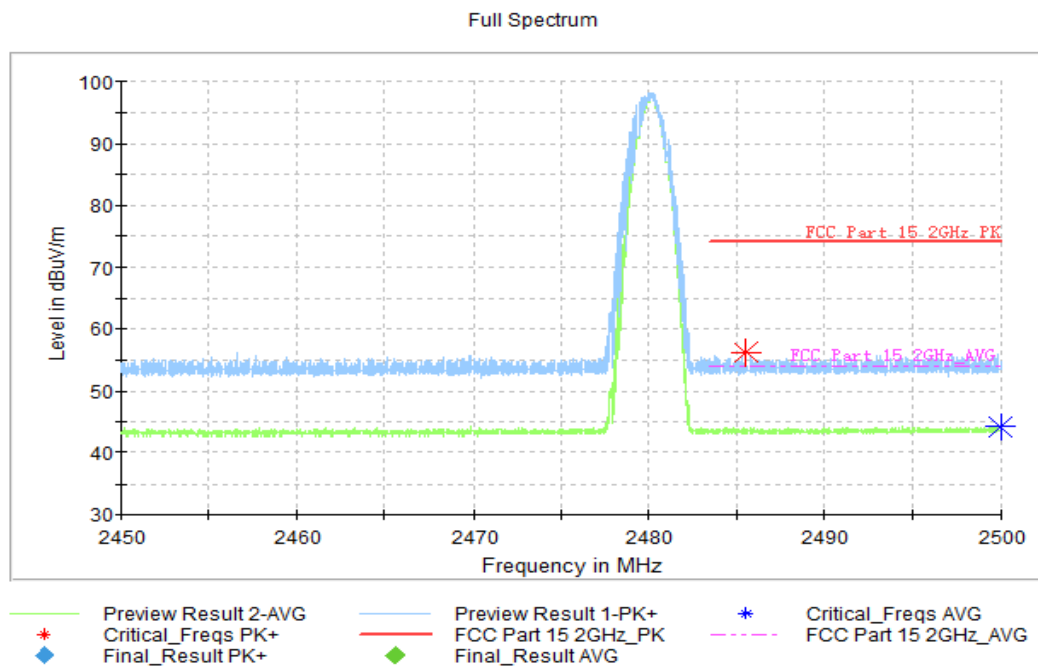
Fig.4. Frequency Band Edges: \pi/4 DQPSK, Channel 78, Hopping Off, 2.45 GHz - 2.50GHz
