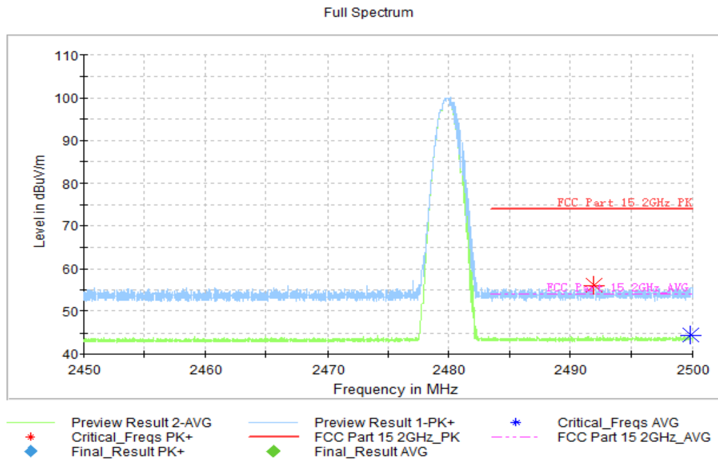
Fig.2. Frequency Band Edges: GFSK, Channel 78, Hopping Off, ch11, 2.45 GHz - 2.50GHz
