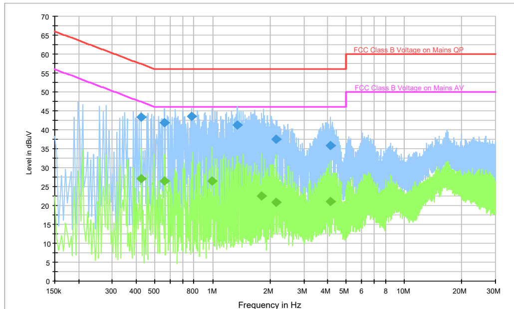
Fig.B.10.2 AC Powerline Conducted Emission-Idle With charger QC16US
