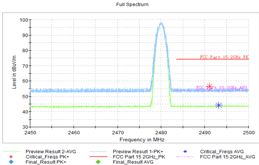
Fig.6. Frequency Band Edges: 8DPSK, Channel 78, 2.45 GHz - 2.50GHz
