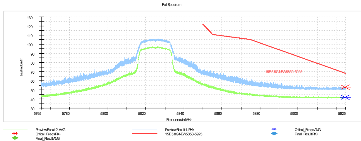
Fig. 2 Band Edges (802.11a Ch165, 5825MHz)
