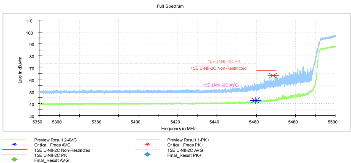
Fig. 19 Band Edges (802.11ac-HT40 Ch102, 5510MHz)
