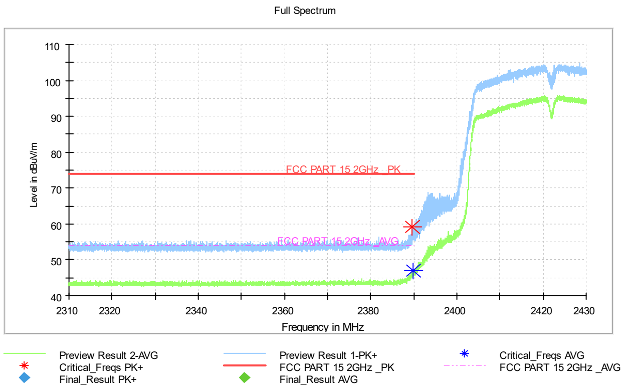
Fig.7 Transmitter Spurious Emission - Radiated (Power): 802.11n-HT40, ch3, 2.31 GHz - 2.43GHz
