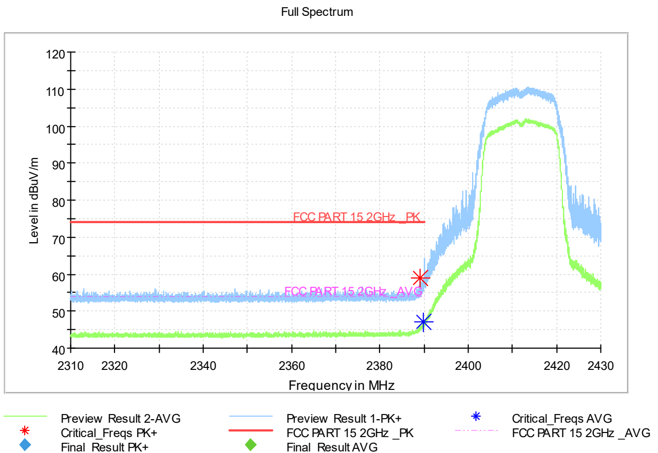
Fig.3 Transmitter Spurious Emission - Radiated (Power): 802.11g, ch1, 2.31 GHz - 2.43GHz
