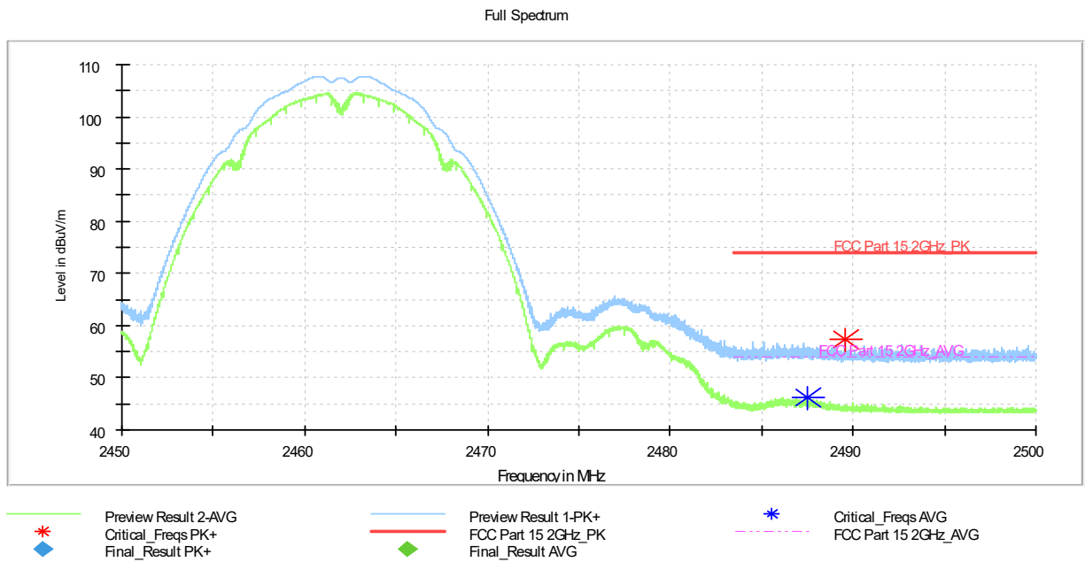
Fig.2 Transmitter Spurious Emission - Radiated (Power): 802.11b, ch11, 2.45 GHz - 2.50GHz
