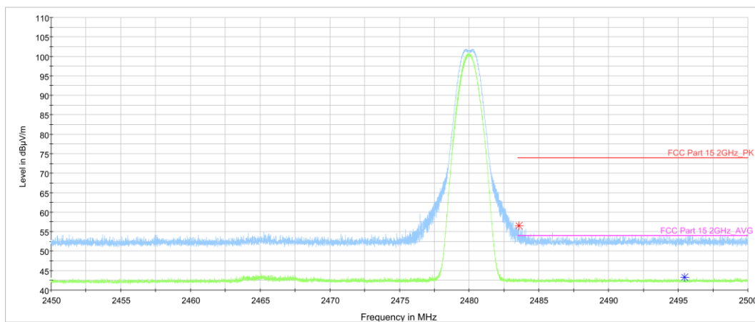
Fig.19. Frequency Band Edges: GFSK, 2480 MHz, Hopping Off, 2.45 GHz - 2.50GHz
